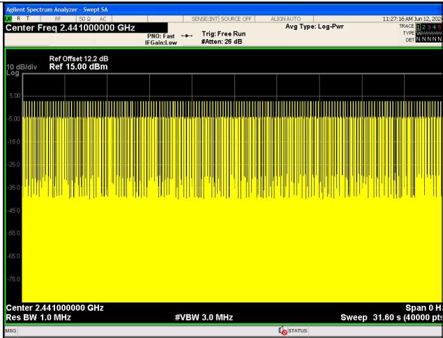
Number of Pulses in 31.6 seconds GFSK_DH1
