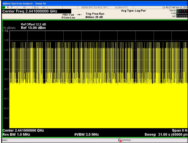
Number of Pulses in 31.6 seconds \pi/4 DQPSK 2-DH3
