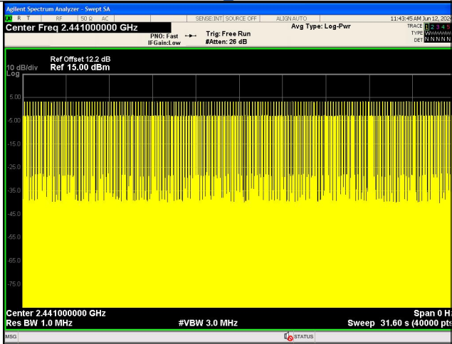
Number of Pulses in 31.6 seconds \pi/4 DQPSK 2-DH1
