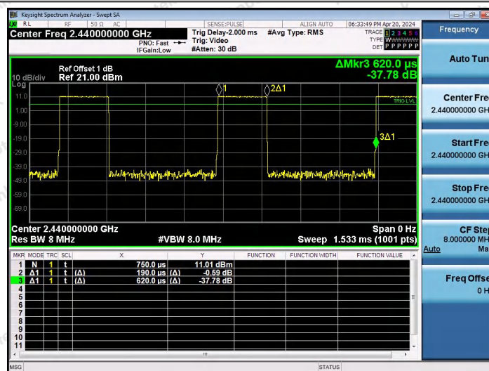
NTNV-BLE_2M-Ant2-2440
