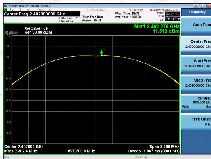
BLE_2M-Ant2-2402-PASS
