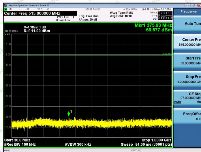
BLE_1M-Ant2-2440-30~1000-PASS
