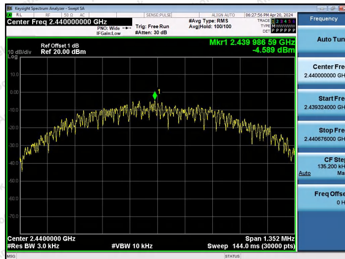
BLE_1M-Ant2-2440-PASS
