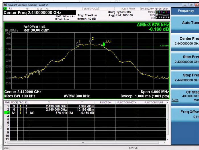
BLE_1M-Ant2-2440-PASS
