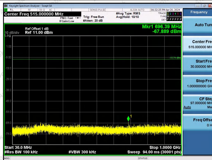
BLE_2M-Ant2-2402-30~1000-PASS
