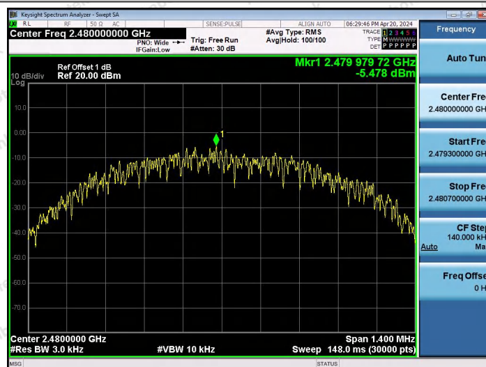
BLE_1M-Ant2-2480-PASS
