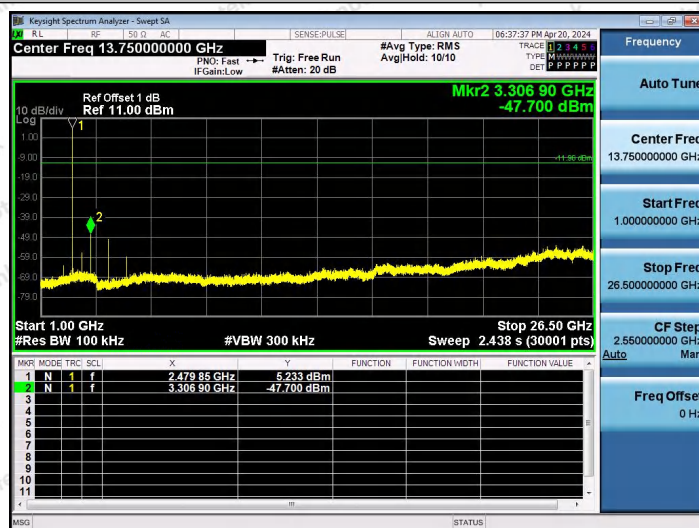
BLE_2M-Ant2-2480-1000~26500-PASS
