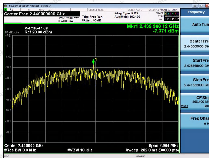
BLE_2M-Ant2-2440-PASS
