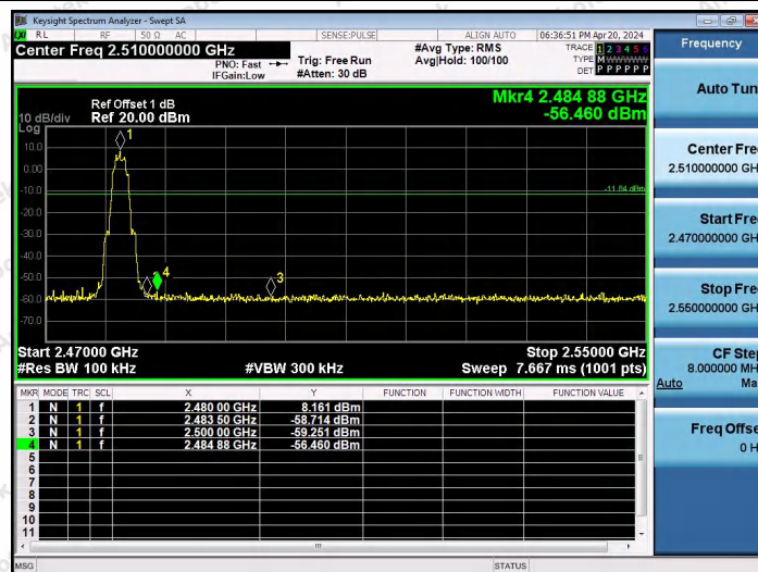
BLE_2M-Ant2-2480-PASS
