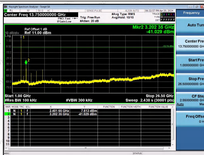
BLE_2M-Ant2-2402-1000~26500-PASS
