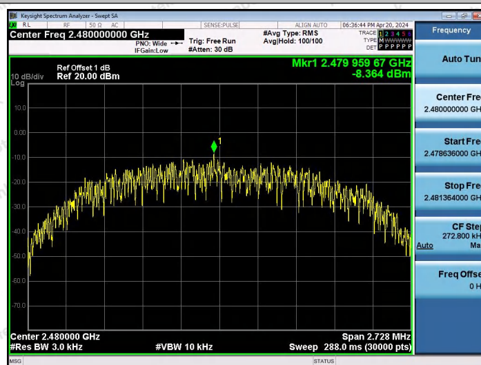
BLE_2M-Ant2-2480-PASS
