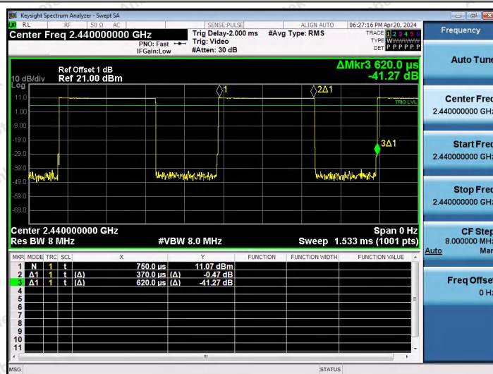
NTNV-BLE 1M-Ant2-2440
