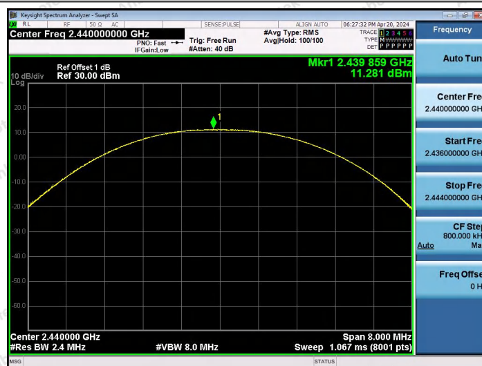
BLE_1M-Ant2-2440-PASS
