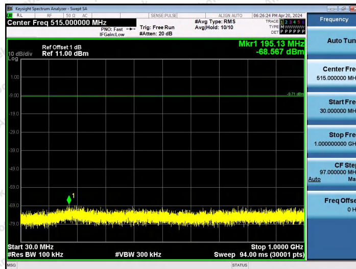
BLE_1M-Ant2-2402-30~1000-PASS
