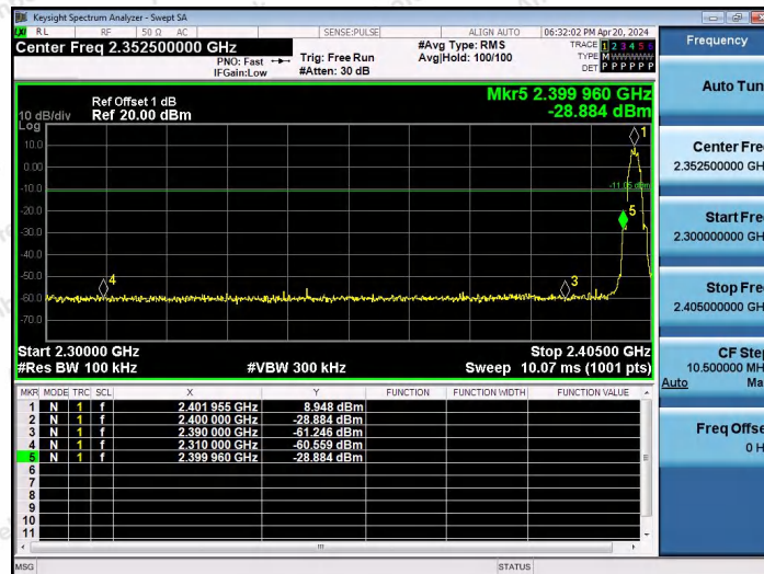
BLE_2M-Ant2-2402-PASS
