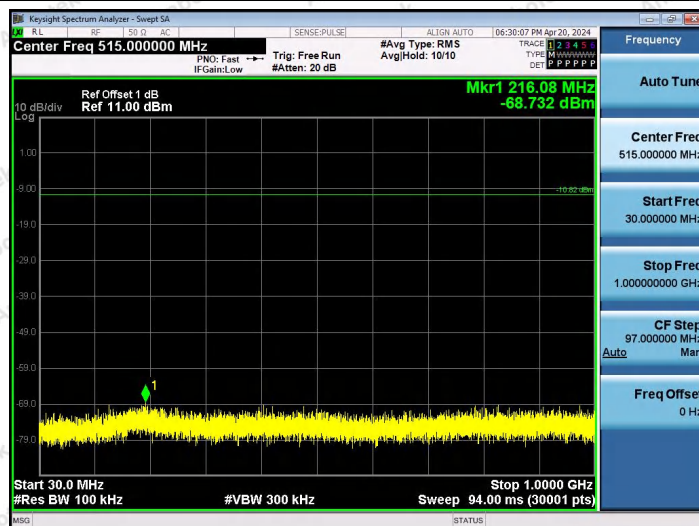
BLE_1M-Ant2-2480-30~1000-PASS
