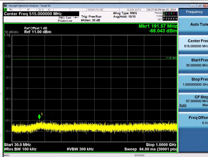
BLE_2M-Ant2-2480-30~1000-PASS
