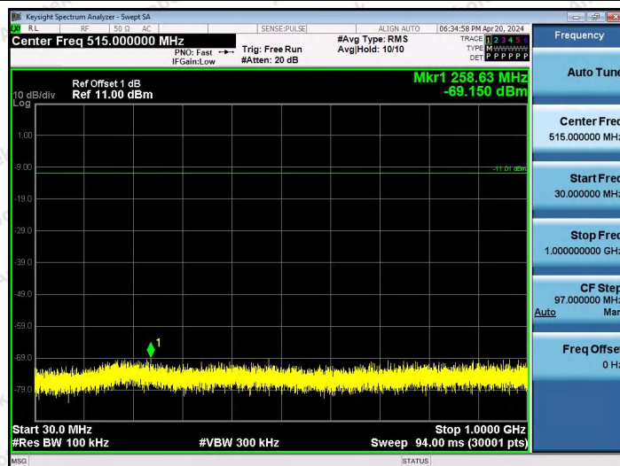
BLE_2M-Ant2-2440-30~1000-PASS
