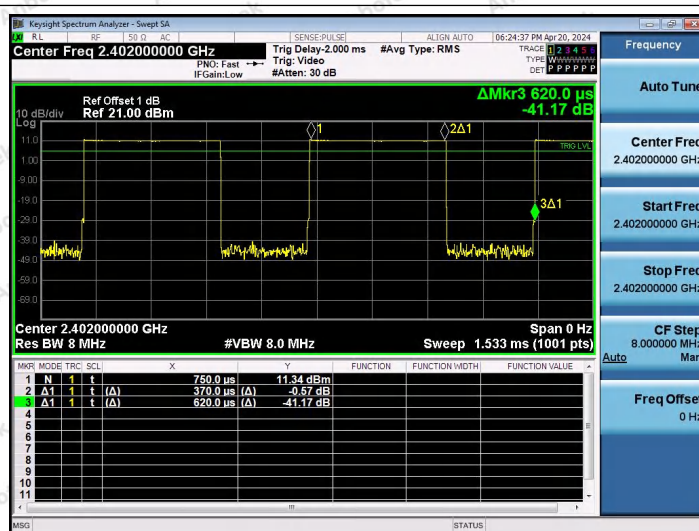
NTNV-BLE 1M-Ant2-2402
