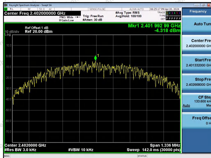
BLE_1M-Ant2-2402-PASS
