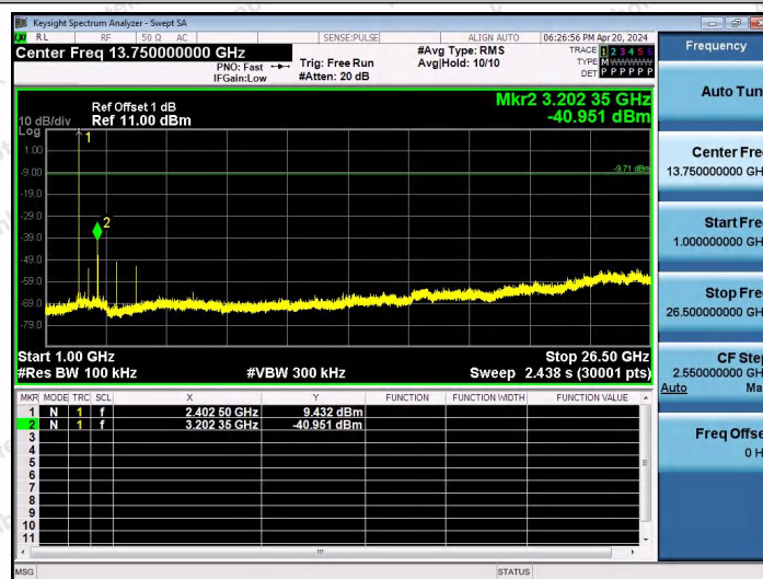
BLE_1M-Ant2-2402-1000~26500-PASS
