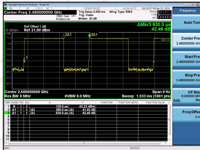
NTNV-BLE_1M-Ant2-2480
