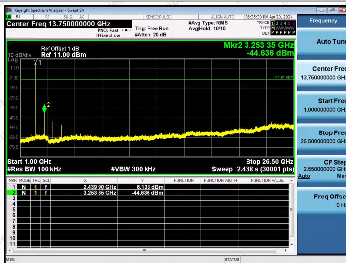
BLE_2M-Ant2-2440-1000~26500-PASS
