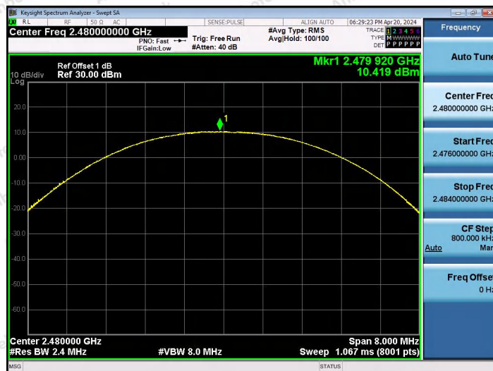
BLE_1M-Ant2-2480-PASS
