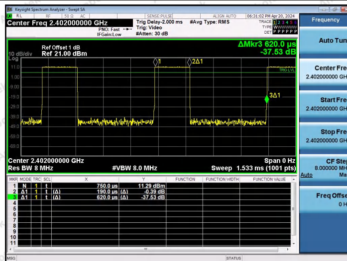
NTNV-BLE_2M-Ant2-2402
