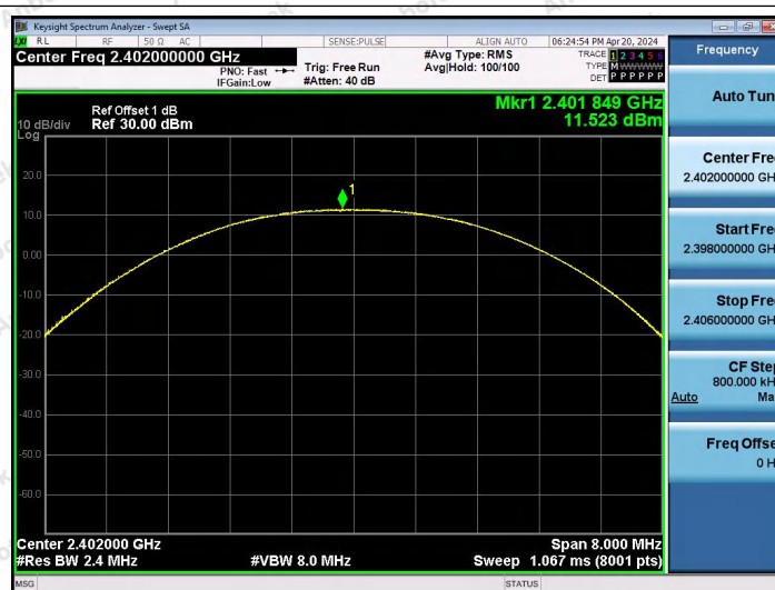
BLE_1M-Ant2-2402-PASS
