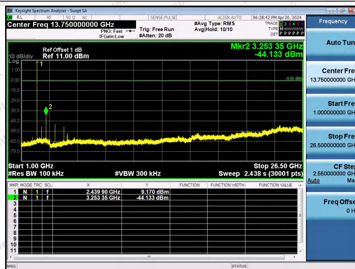
BLE_1M-Ant2-2440-1000~26500-PASS
