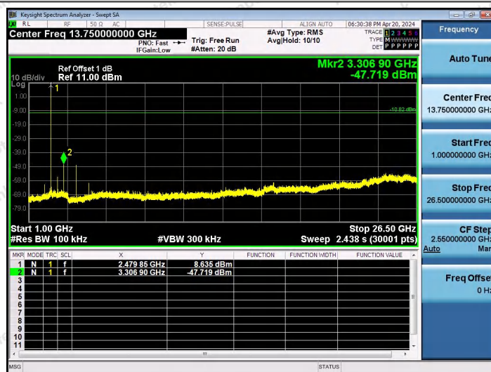
BLE_1M-Ant2-2480-1000~26500-PASS
