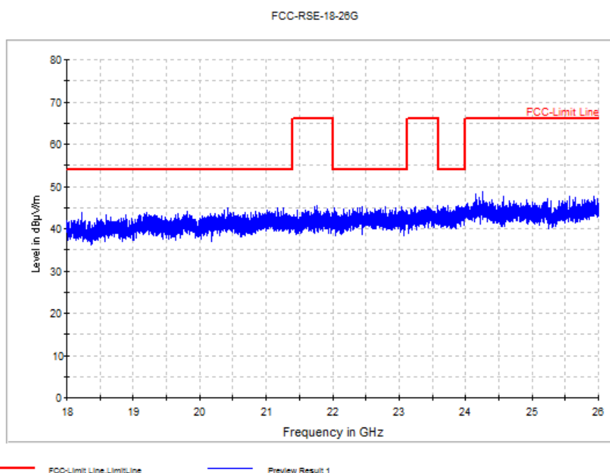
Fig. 77 Radiated Spurious Emission (All channel, 18 GHz ~26 GHz)
