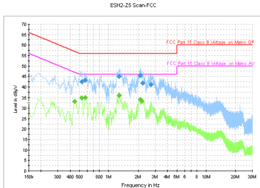
Fig. 102 AC Power line Conducted Emission (GFSK, Ch39)
