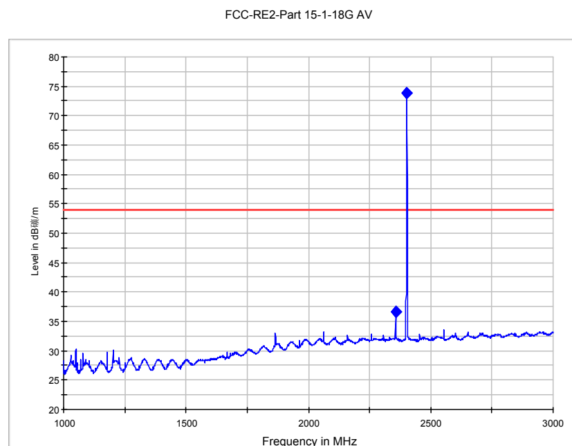
Fig. 69 Radiated Spurious Emission (8DPSK, Ch0, 1 GHz ~3 GHz)
