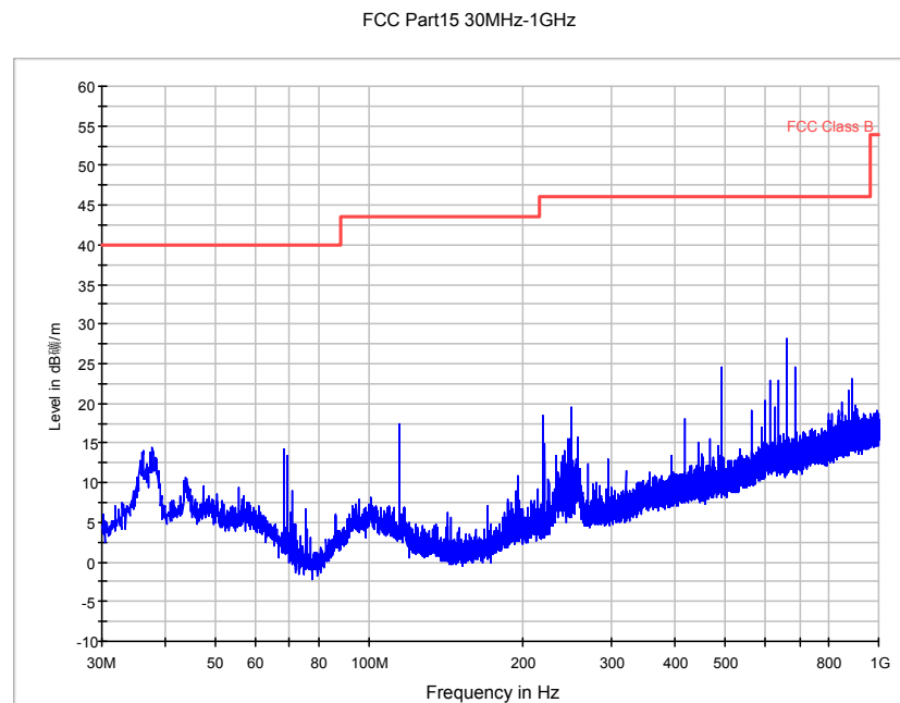
Fig. 74 Radiated Spurious Emission (8DPSK, Ch78, 30 MHz ~1 GHz)
