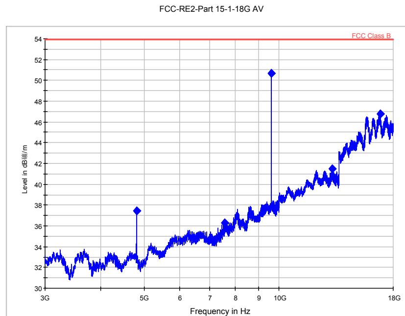
Fig. 52 Radiated Spurious Emission (GFSK, Ch0, 3 GHz ~18 GHz)
