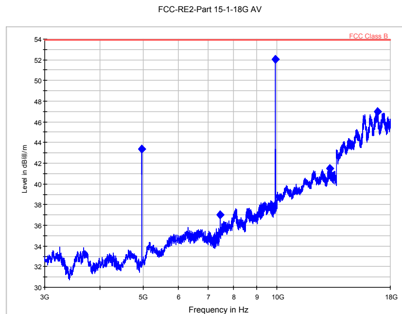
Fig. 67 Radiated Spurious Emission ( \pi/4 DQPSK, Ch78, 3 GHz ~18 GHz)
