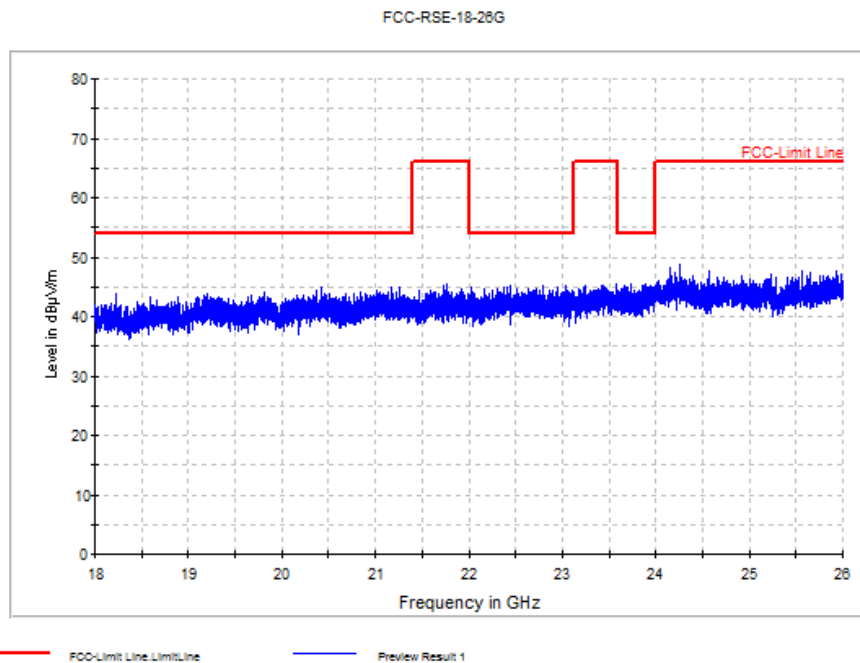
Fig. 77 Radiated Spurious Emission (All channel, 18 GHz ~26 GHz)
