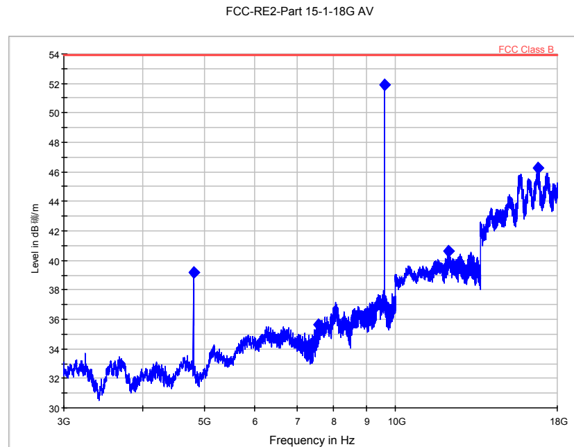
Fig. 64 Radiated Spurious Emission ( \pi/4 DQPSK, Ch39, 3 GHz ~18 GHz)
