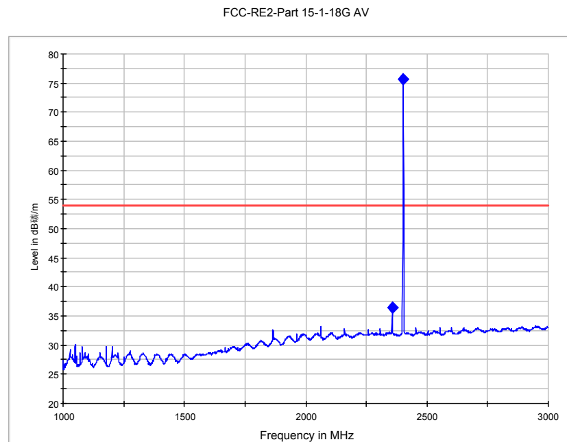
Fig. 51 Radiated Spurious Emission (GFSK, Ch0, 1 GHz ~3 GHz)
