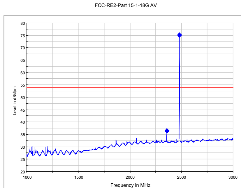
Fig. 75 Radiated Spurious Emission (8DPSK, Ch78, 1 GHz ~3 GHz)
