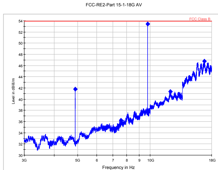
Fig. 55 Radiated Spurious Emission (GFSK, Ch39, 3 GHz ~18 GHz)
