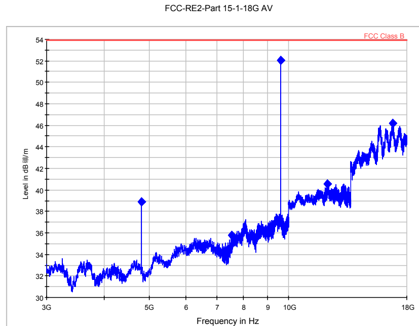
Fig. 70 Radiated Spurious Emission (8DPSK, Ch0, 3 GHz ~18 GHz)
