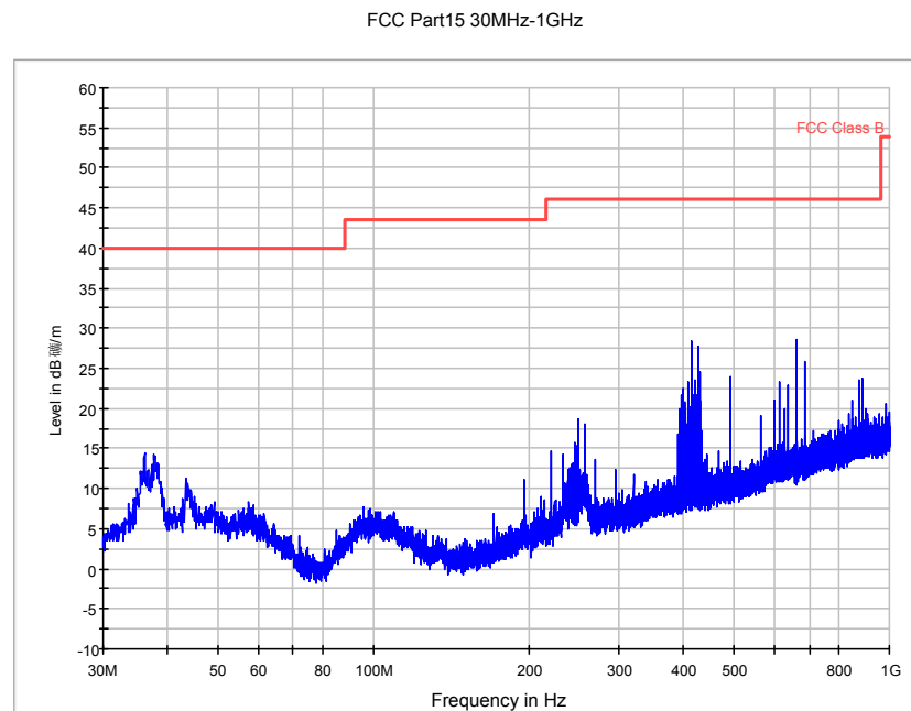
Fig. 68 Radiated Spurious Emission (8DPSK, Ch0, 30 MHz ~1 GHz)
