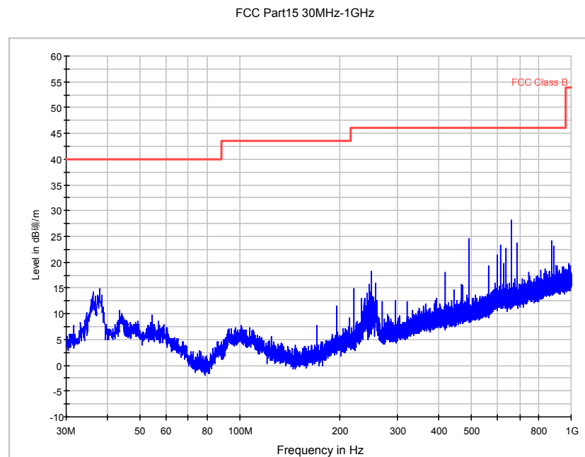
Fig. 56 Radiated Spurious Emission (GFSK, Ch78, 30 MHz ~1 GHz)
