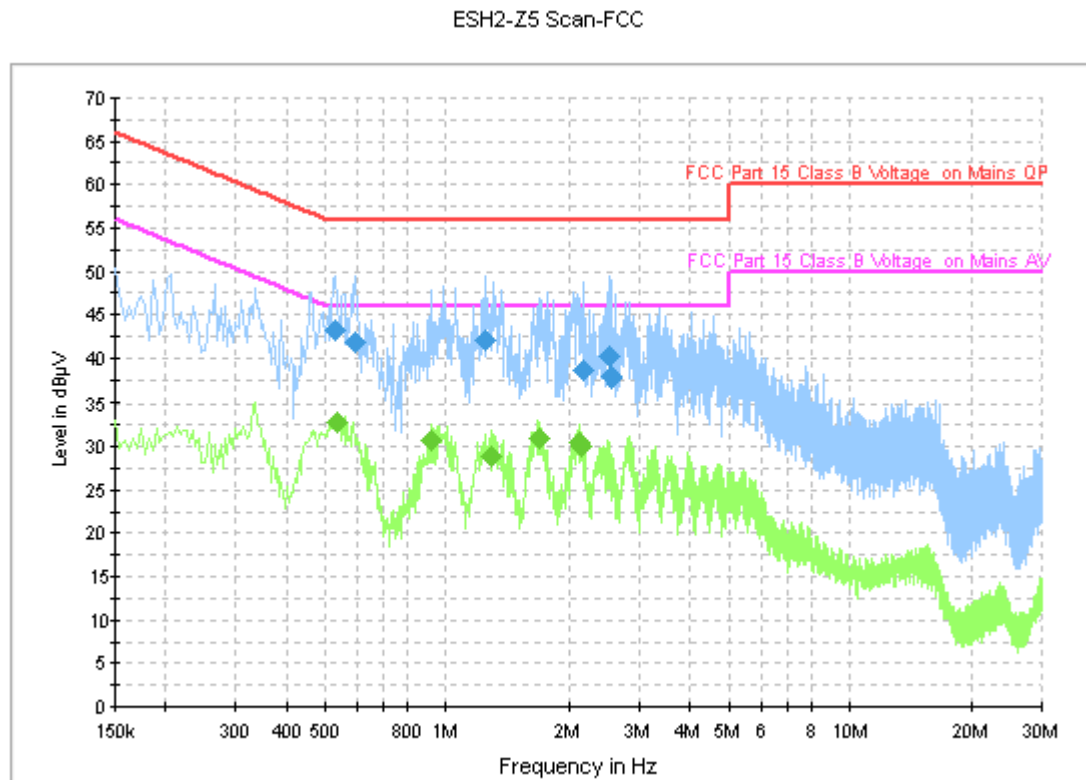
Fig. 102 AC Power line Conducted Emission (GFSK, Ch39)
