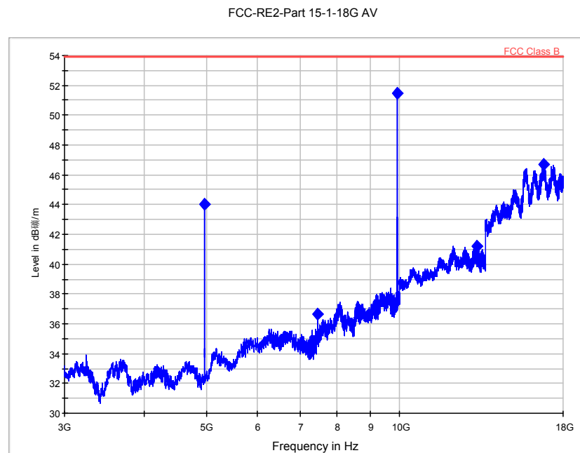
Fig. 76 Radiated Spurious Emission (8DPSK, Ch78, 3 GHz ~18 GHz)
