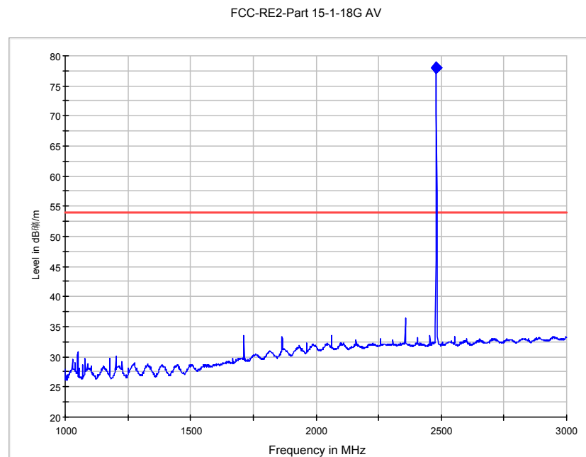
Fig. 57 Radiated Spurious Emission (GFSK, Ch78, 1 GHz ~3 GHz)
