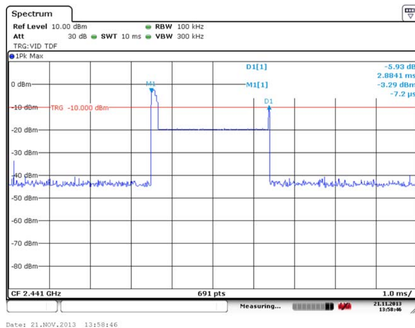
Fig. 89 Time of Occupancy(Dwell Time) ( \pi/4 DQPSK, Ch39)
