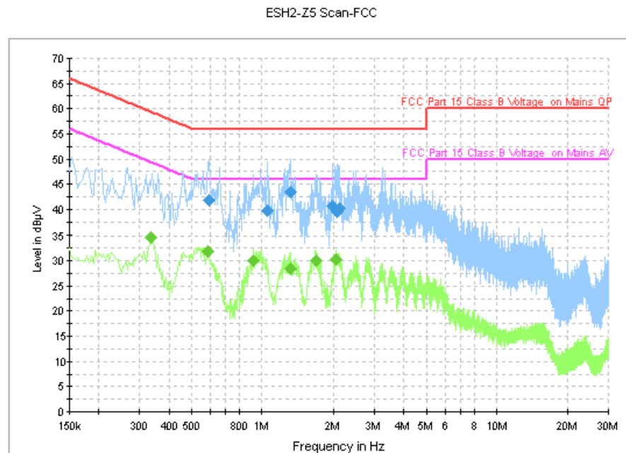
Fig. 104 AC Power line Conducted Emission (8DPSK, Ch39)
