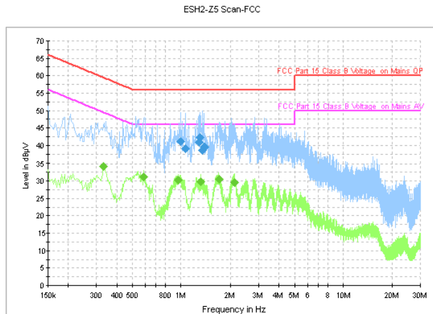
Fig. 103 AC Power line Conducted Emission ( \pi/4 DQPSK, Ch39)
