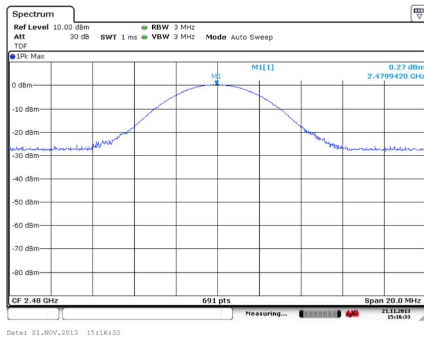
Fig. 9 Maximum Peak Output Power (8DPSK, Ch78, Hopping OFF)
