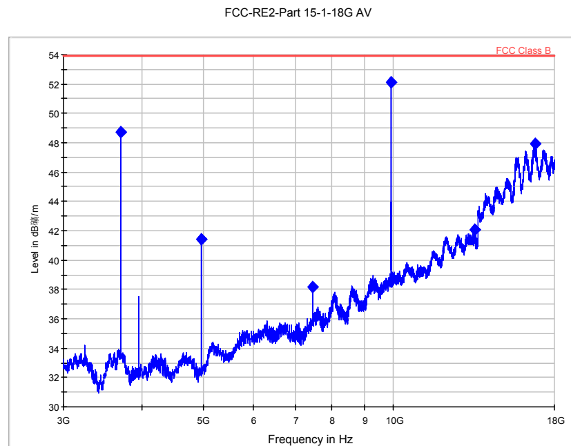
Fig. 58 Radiated Spurious Emission (GFSK, Ch78, 3 GHz ~18 GHz)
