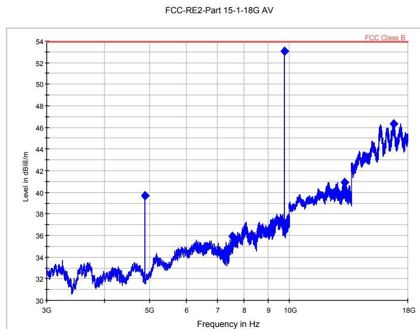
Fig. 73 Radiated Spurious Emission (8DPSK, Ch39, 3 GHz ~18 GHz)
