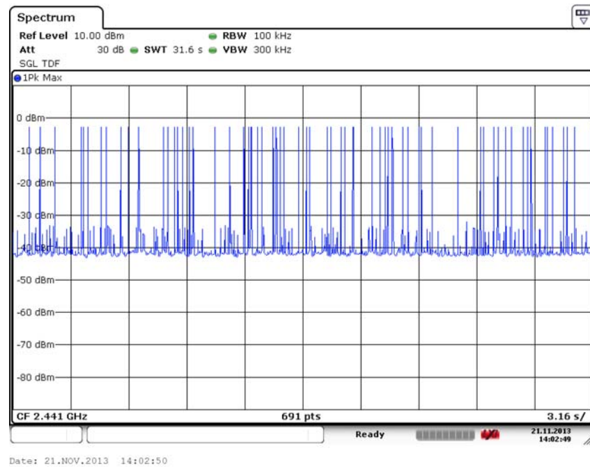
Fig. 90 Number of Transmissions ( \pi/4 DQPSK, Ch39)
