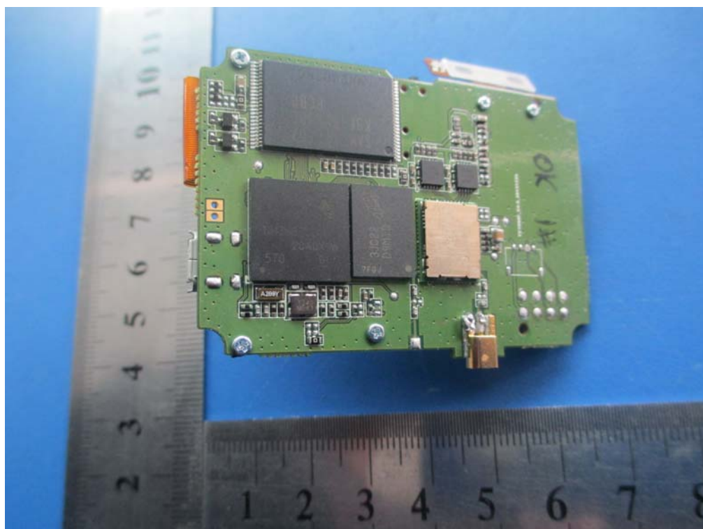
Mainboard- TopView
