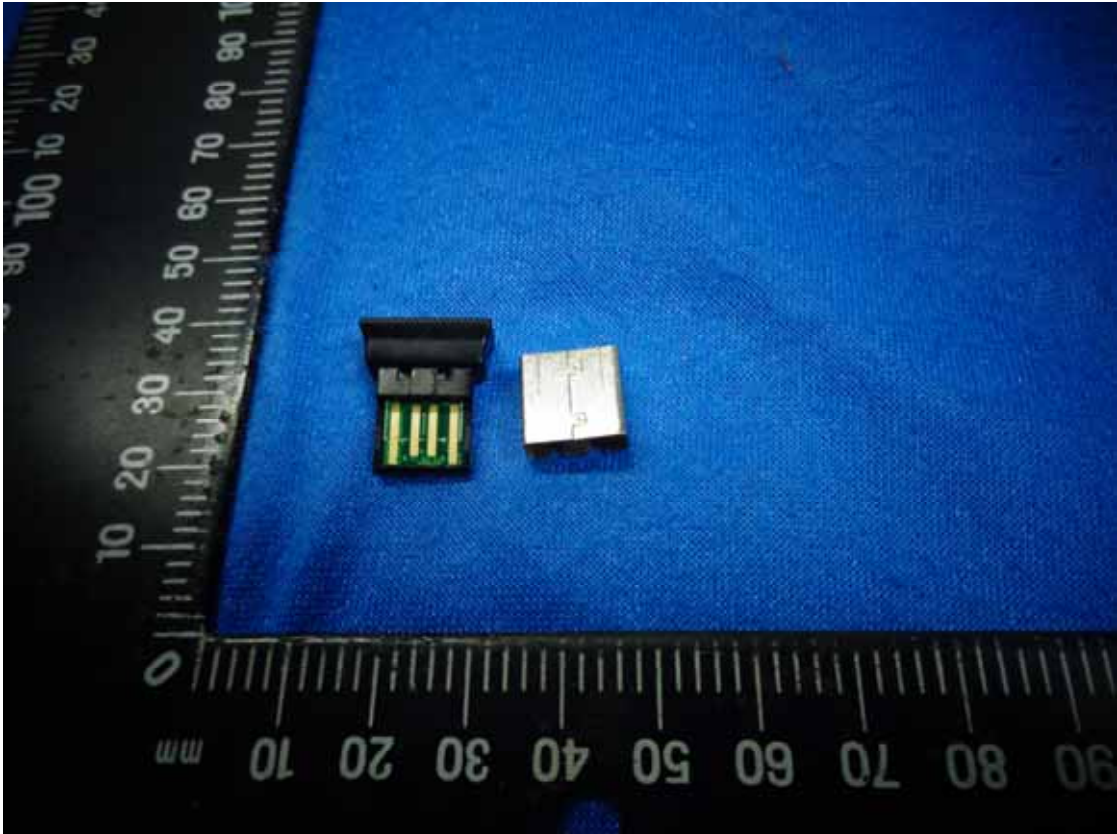
Figure 1 Internal View
