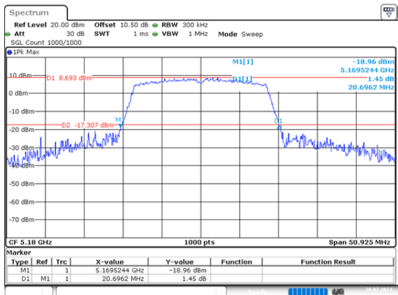
n20_5180MHz_Chain 0 20.696MHz
