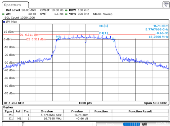
n20_5785MHz_Chain 0 16.767MHz
