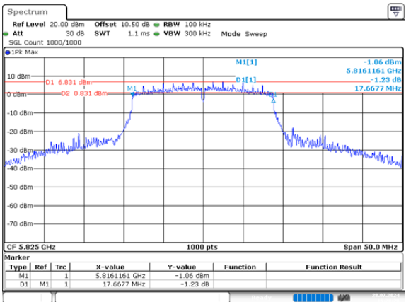
n20_5825MHz_Chain 1 17.668MHz
