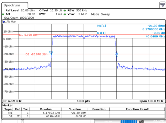
ax40_5190MHz_RU_Full_Chain 1 40.040MHz
