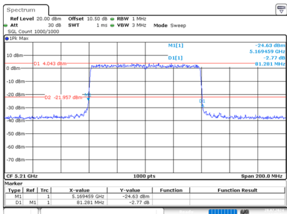
ax80_5210MHz_RU_Full_Chain 0 81.281MHz
