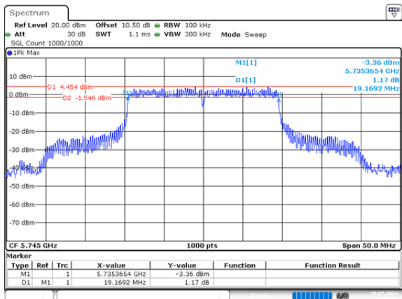
ax20_5745MHz_RU_Full_Chain 0 19.169MHz
