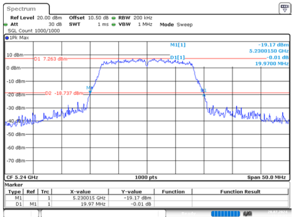
a_5240MHz_Chain 0 19.970MHz
