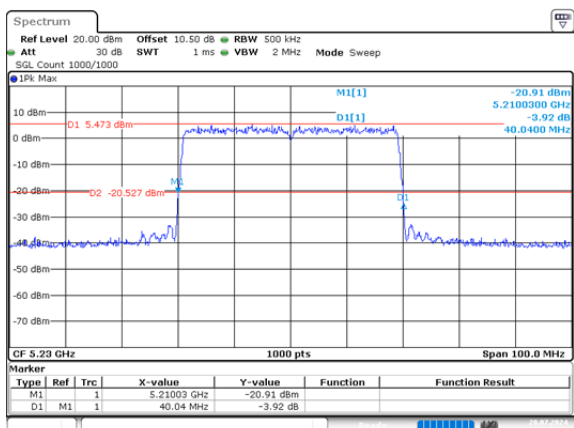
ax40_5230MHz_RU_Full_Chain 0 40.040MHz
