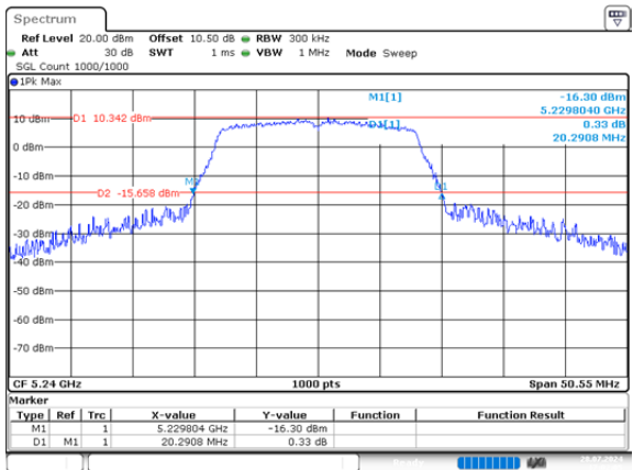
a_5240MHz_Chain 1 20.291MHz
