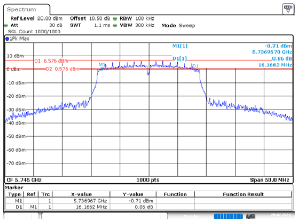
n20_5745MHz_Chain 0 16.166MHz
