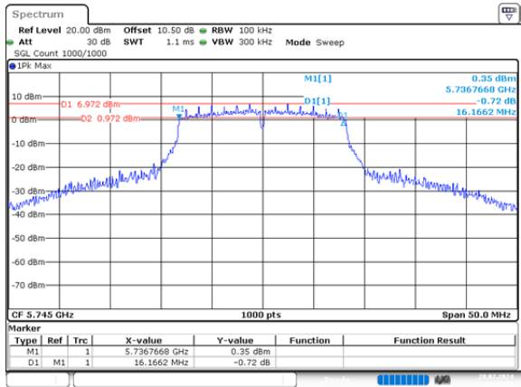
a_5745MHz_Chain 0 16.166MHz
