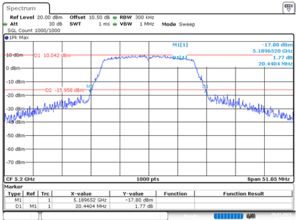
a_5200MHz_Chain 1 20.440MHz
