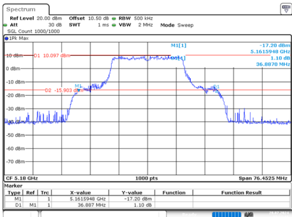
ax20_5180MHz_RU_Full_Chain 1 36.887MHz
