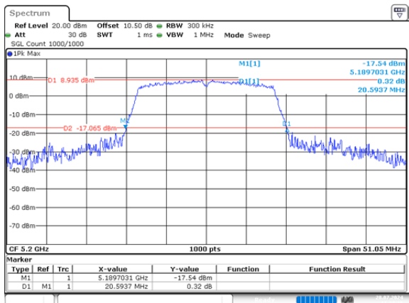
n20_5200MHz_Chain 0 20.594MHz
