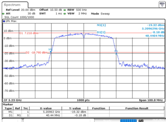
n40_5230MHz_Chain 0 40.440MHz
