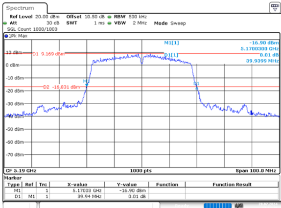
n40_5190MHz_Chain 1 39.940MHz
