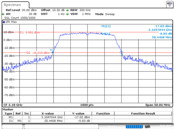
a_5180MHz_Chain 1 20.441MHz
