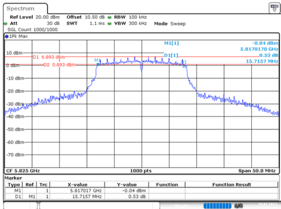
a_5825MHz_Chain 0 15.716MHz
