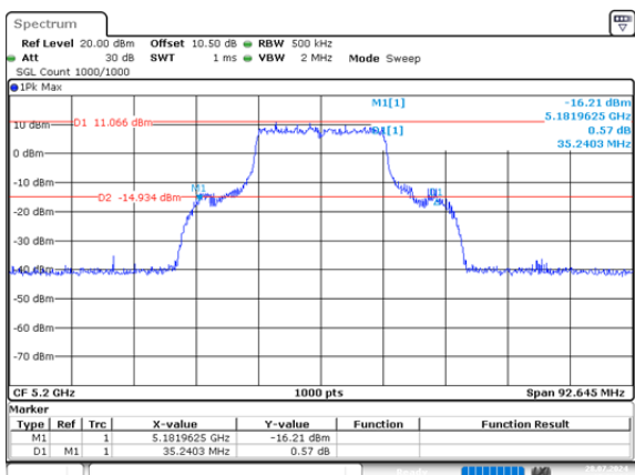
ax20_5200MHz_RU_Full_Chain 1 35.240MHz
