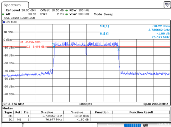
ac80_5775MHz_Chain 1 76.677MHz
