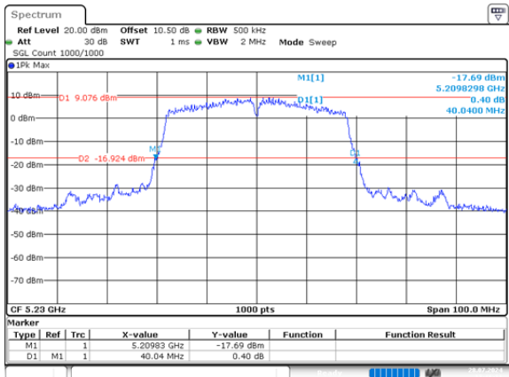
n40_5230MHz_Chain 1 40.040MHz
