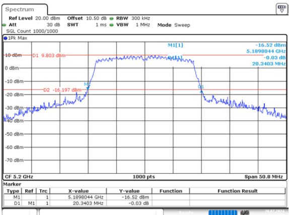
n20_5200MHz_Chain 1 20.340MHz
