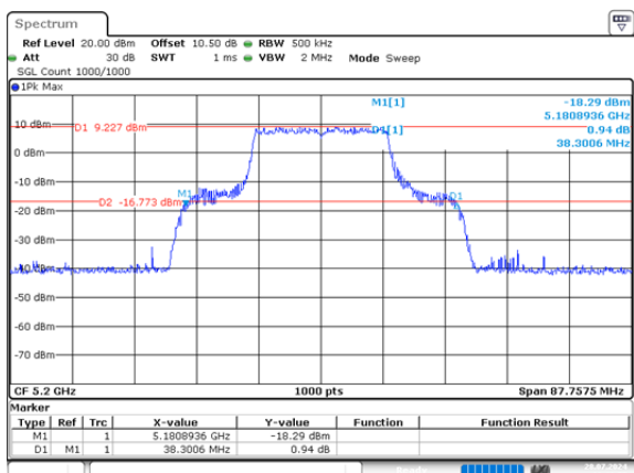
ax20_5200MHz_RU_Full_Chain 0 38.301MHz
