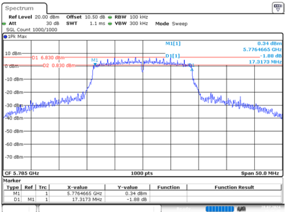
n20_5785MHz_Chain 1 17.317MHz
