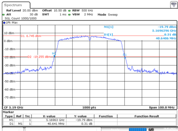
n40_5190MHz_Chain 0 40.641MHz
