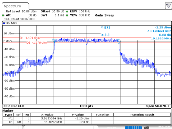
ax20_5825MHz_RU_Full_Chain 1 19.169MHz
