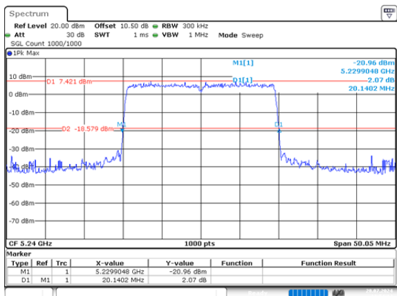
ax20_5240MHz_RU_Full_Chain 0 20.140MHz
