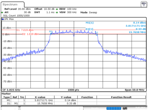
a_5825MHz_Chain 1 15.766MHz
