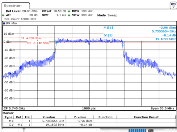
ax20_5745MHz_RU_Full_Chain 1 19.169MHz
