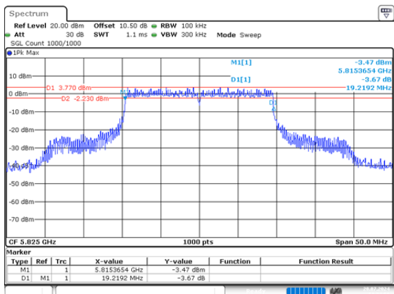
ax20_5825MHz_RU_Full_Chain 0 19.219MHz
