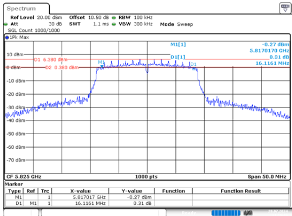
n20_5825MHz_Chain 0 16.116MHz
