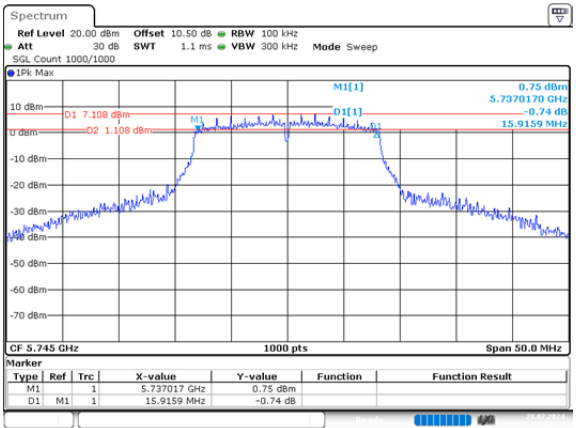
a_5745MHz_Chain 1 15.916MHz
