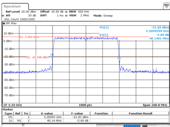
ax40_5230MHz_RU_Full_Chain 1 40.140MHz
