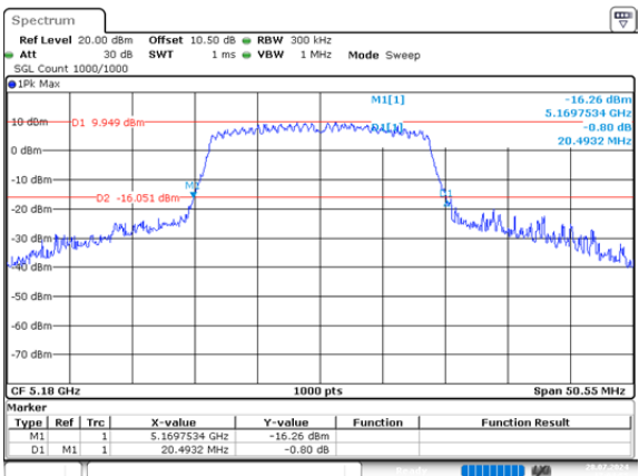
n20_5180MHz_Chain 1 20.493MHz
