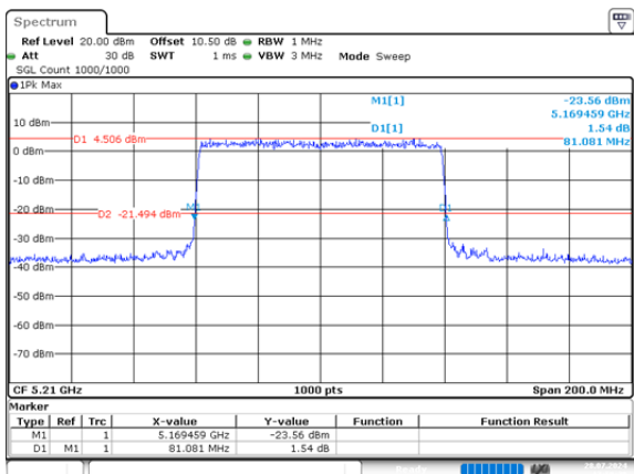
ax80_5210MHz_RU_Full_Chain 1 81.081MHz
