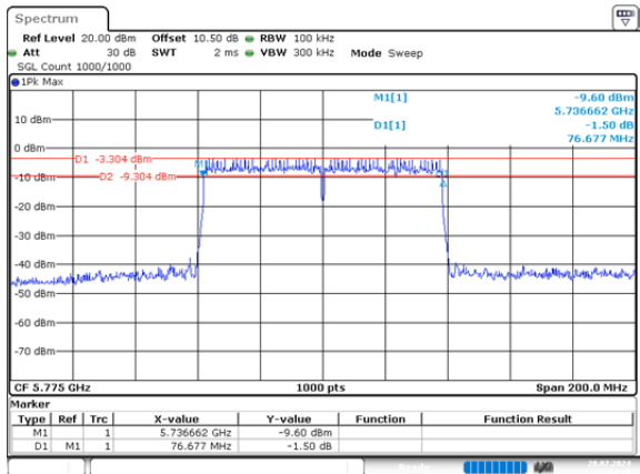
ac80_5775MHz_Chain 0 76.677MHz
