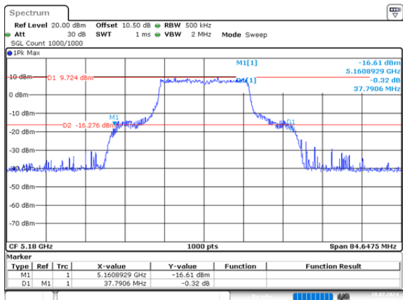
ax20_5180MHz_RU_Full_Chain 0 37.791MHz
