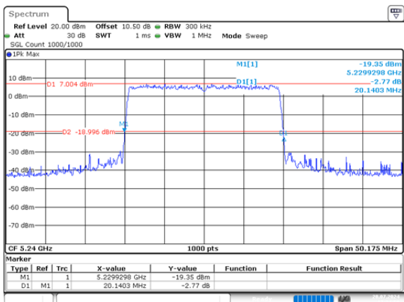
ax20_5240MHz_RU_Full_Chain 1 20.140MHz
