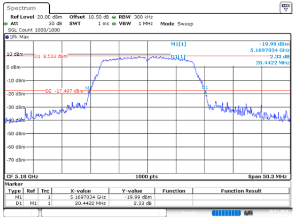
a_5180MHz_Chain 0 20.442MHz
