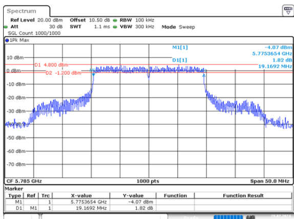
ax20_5785MHz_RU_Full_Chain 0 19.169MHz
