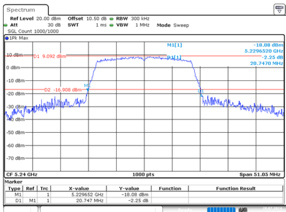
n20_5240MHz_Chain 0 20.747MHz
