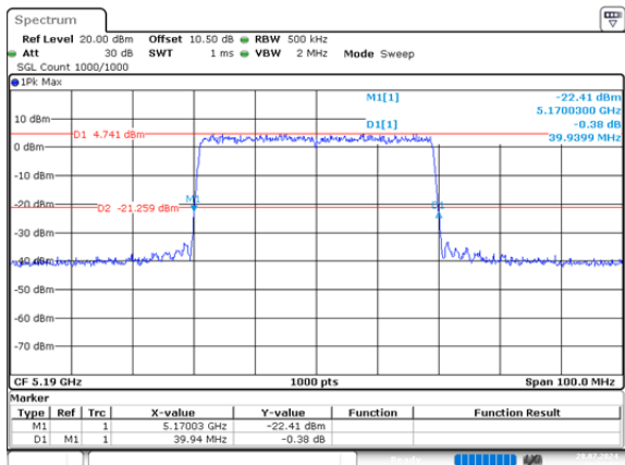
ax40_5190MHz_RU_Full_Chain 0 39.940MHz
