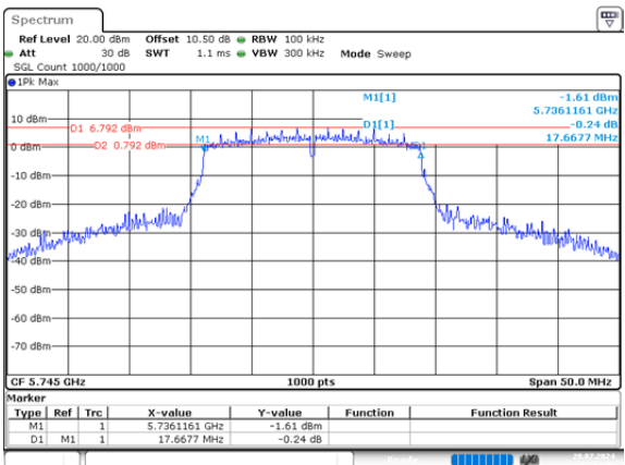
n20_5745MHz_Chain 1 17.668MHz
