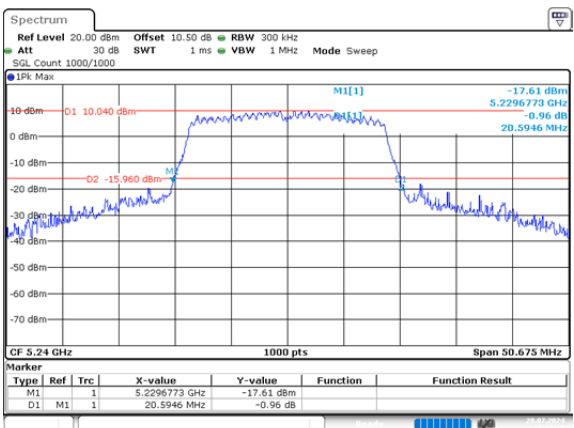
n20_5240MHz_Chain 1 20.595MHz
