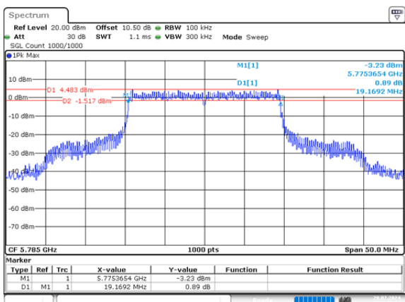
ax20_5785MHz_RU_Full_Chain 1 19.169MHz
