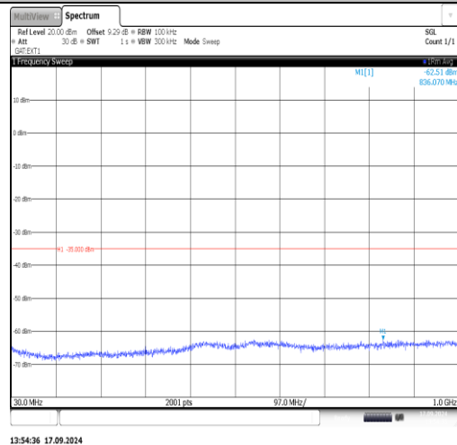
Band38-5MHz-16QAM-38225-1RB#0-20000~27000-PASS
