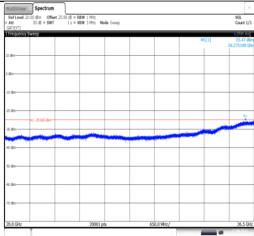
Band38-10MHz-16QAM-38200-1RB#0-20000~26500-PASS
