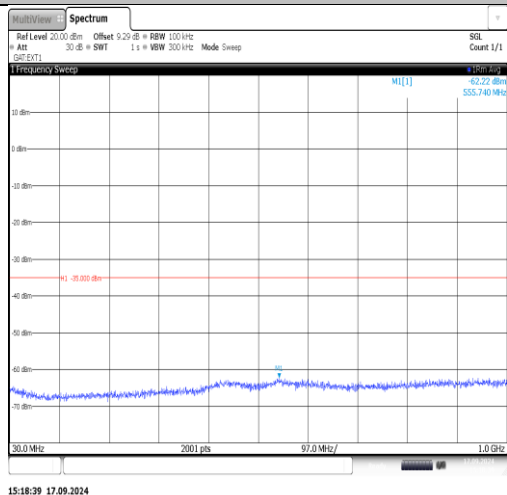
Band38-20MHz-16QAM-38000-1RB#0-20000~27000-PASS
