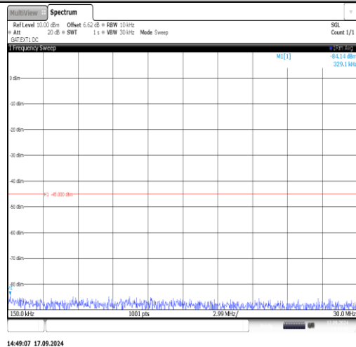
Band38-15MHz-16QAM-38000-1RB#0-20000~26500-PASS
