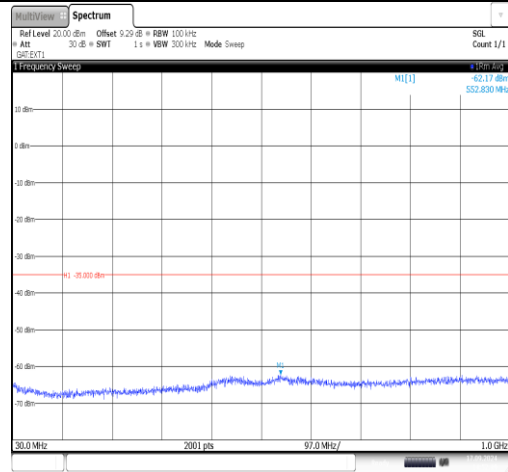
Band38-15MHz-16QAM-38175-1RB#0-30~1000-PASS
