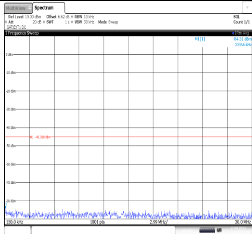
Band38-10MHz-16QAM-38200-1RB#0-0.15~30-PASS
