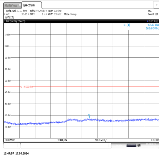
Band38-5MHz-QPSK-38000-1RB#0-20000~27000-PASS
