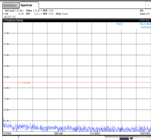
Band38-5MHz-16QAM-38000-1RB#0-0.009~0.15-PASS
