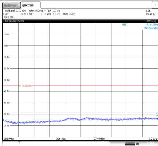
Band38-5MHz-16QAM-38000-1RB#0-30~1000-PASS
