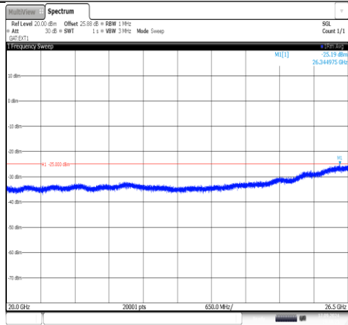
Band38-15MHz-16QAM-38175-1RB#0-20000~26500-PASS
