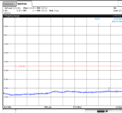
Band38-10MHz-16QAM-38200-1RB#0-30~1000-PASS
