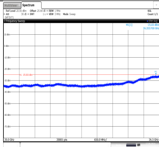
Band38-5MHz-16QAM-38000-1RB#0-20000~26500-PASS
