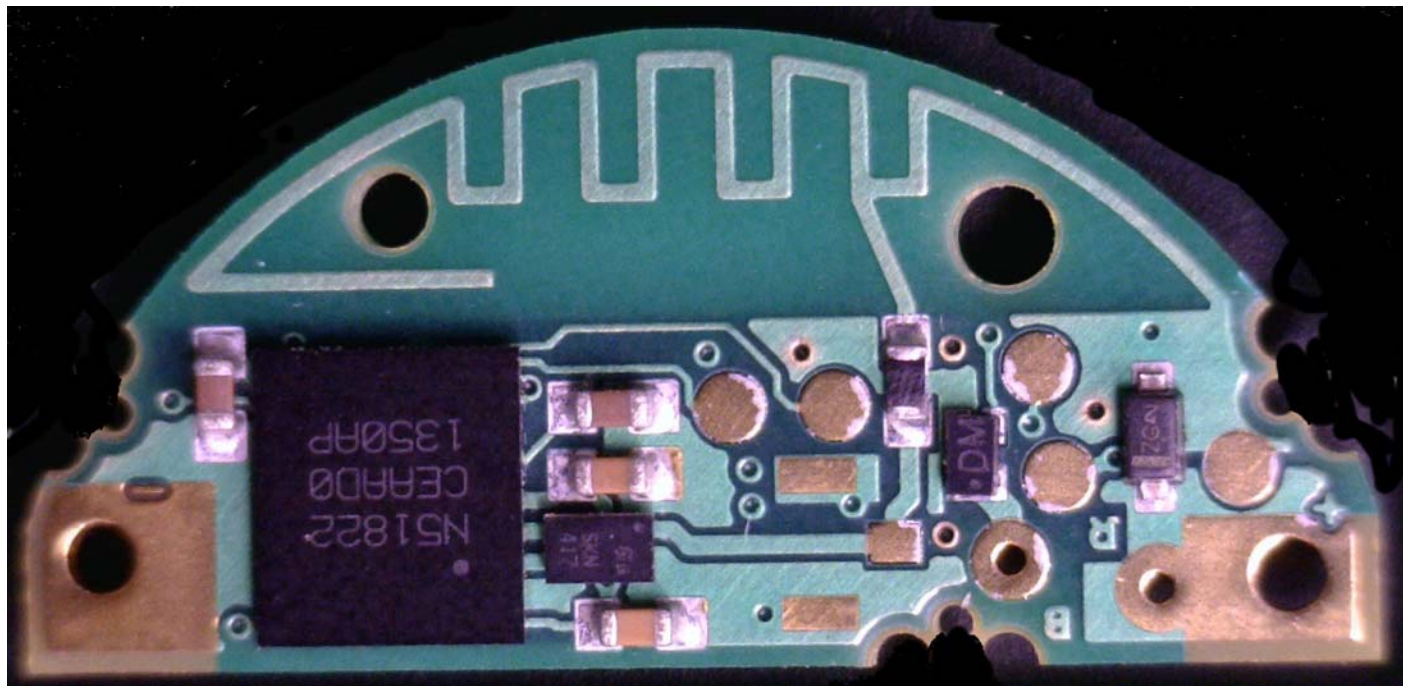
Figure 1 - ditto PWB front side, showing antenna
