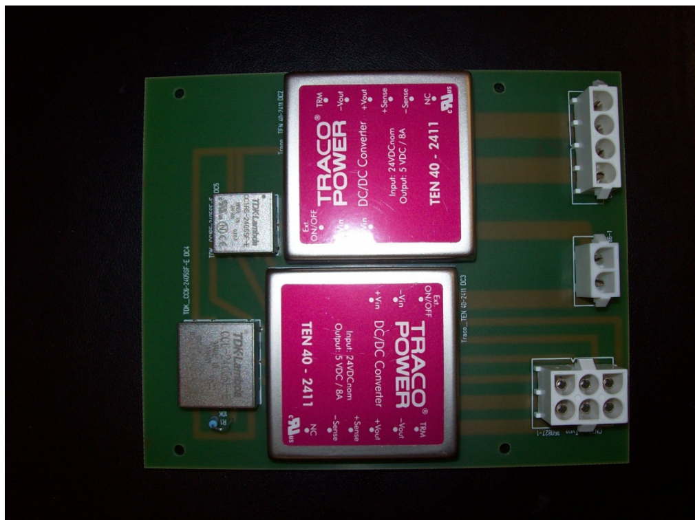
Photo 2: DC/DC-Converter
