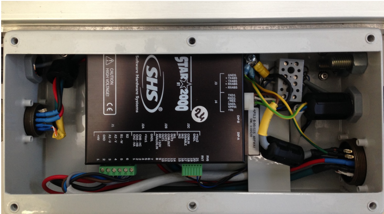
Photo 3: Position Controller
