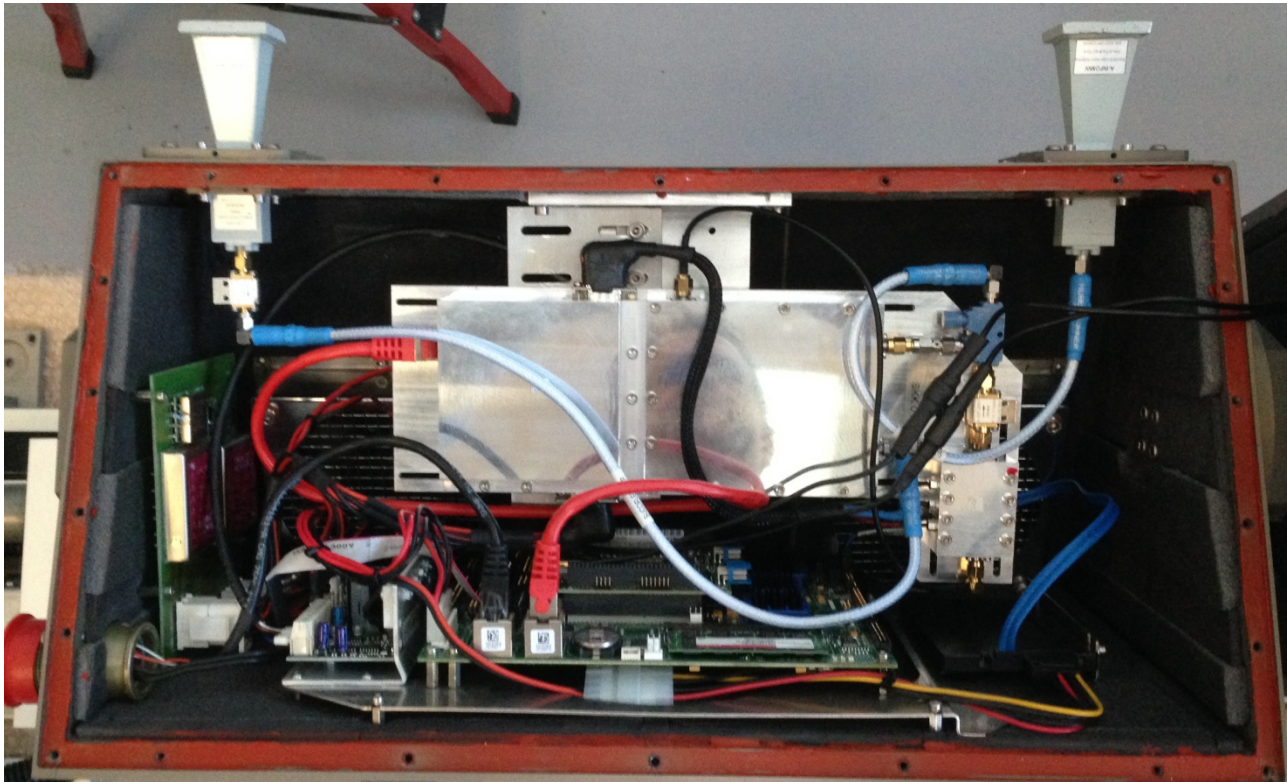
Photo 4: Measure Head
