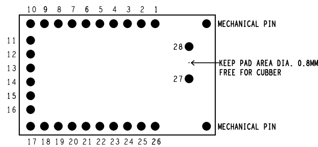
Figure 3: Module pin-out (top-view)
