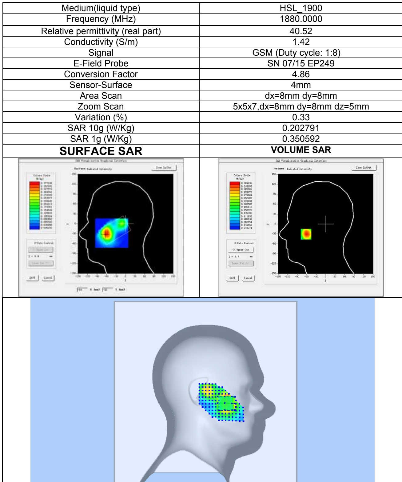
Plot 13: GSM1900, Middle channel (Left Head, Tilt) Product Description: GSM Mobile Phone Test Date: May 22,2017
