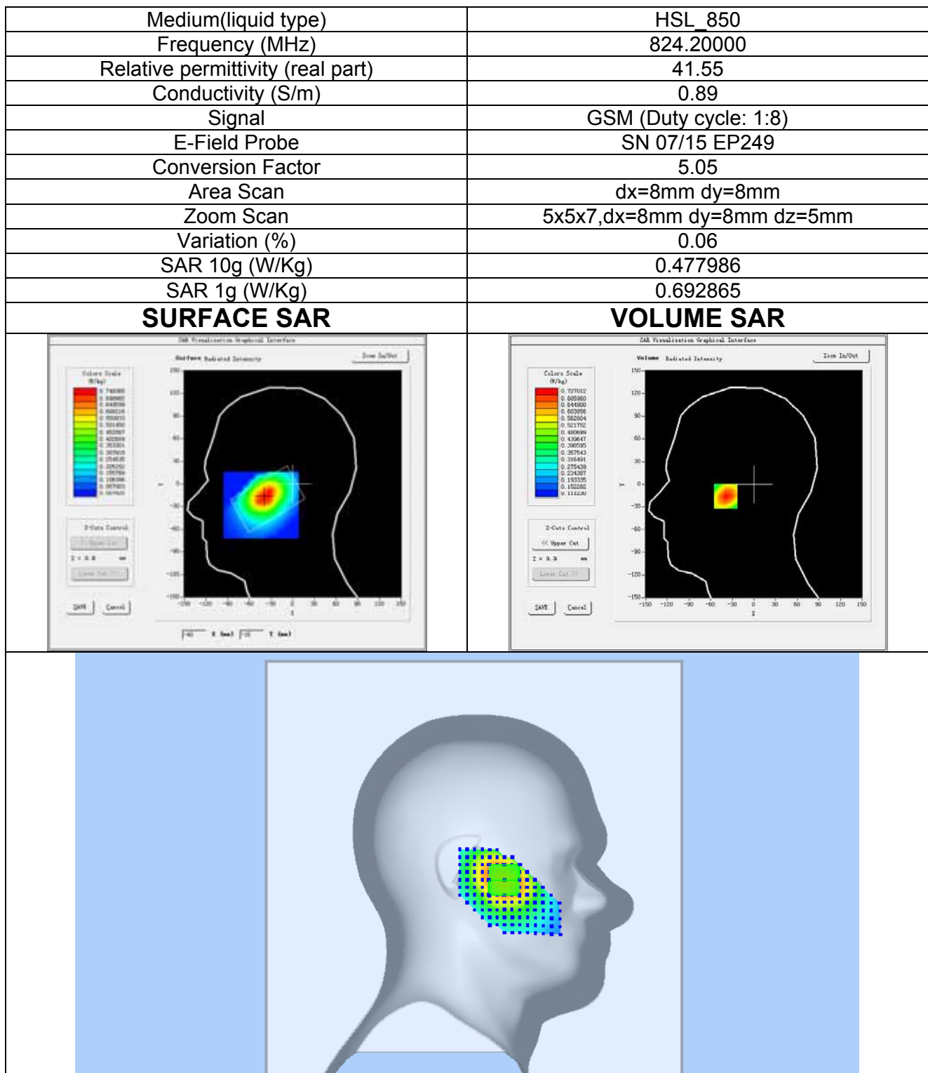
Plot 3: GSM850MHz, Middle channel (Left Head , Cheek) Product Description: GSM Mobile Phone Test Date:May 16,2017
