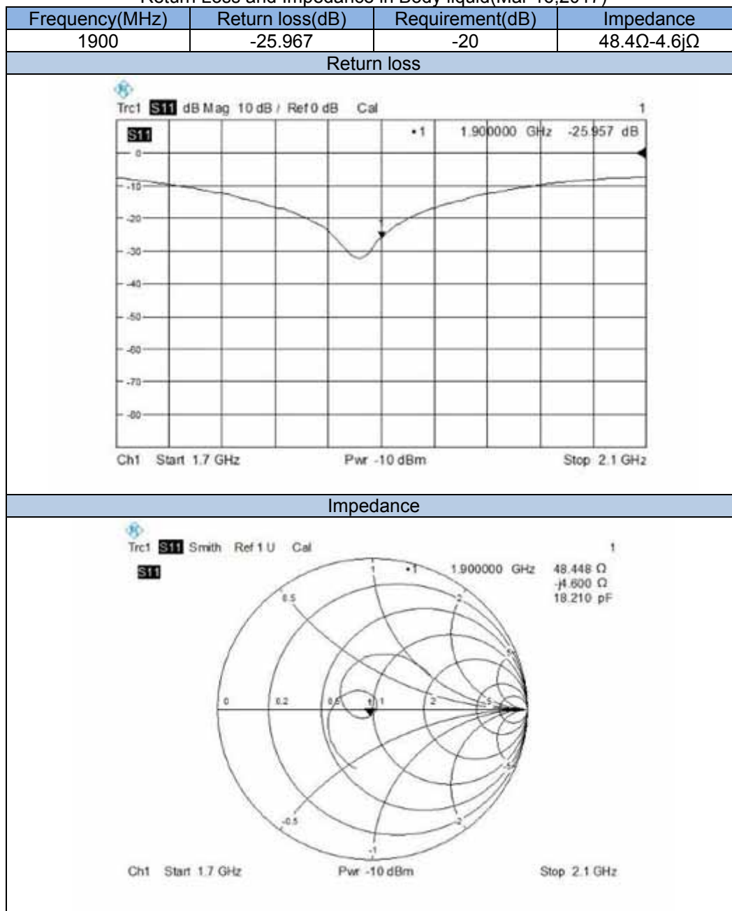
Return Loss and Impedance in Body liquid(Mar 16,2017)
