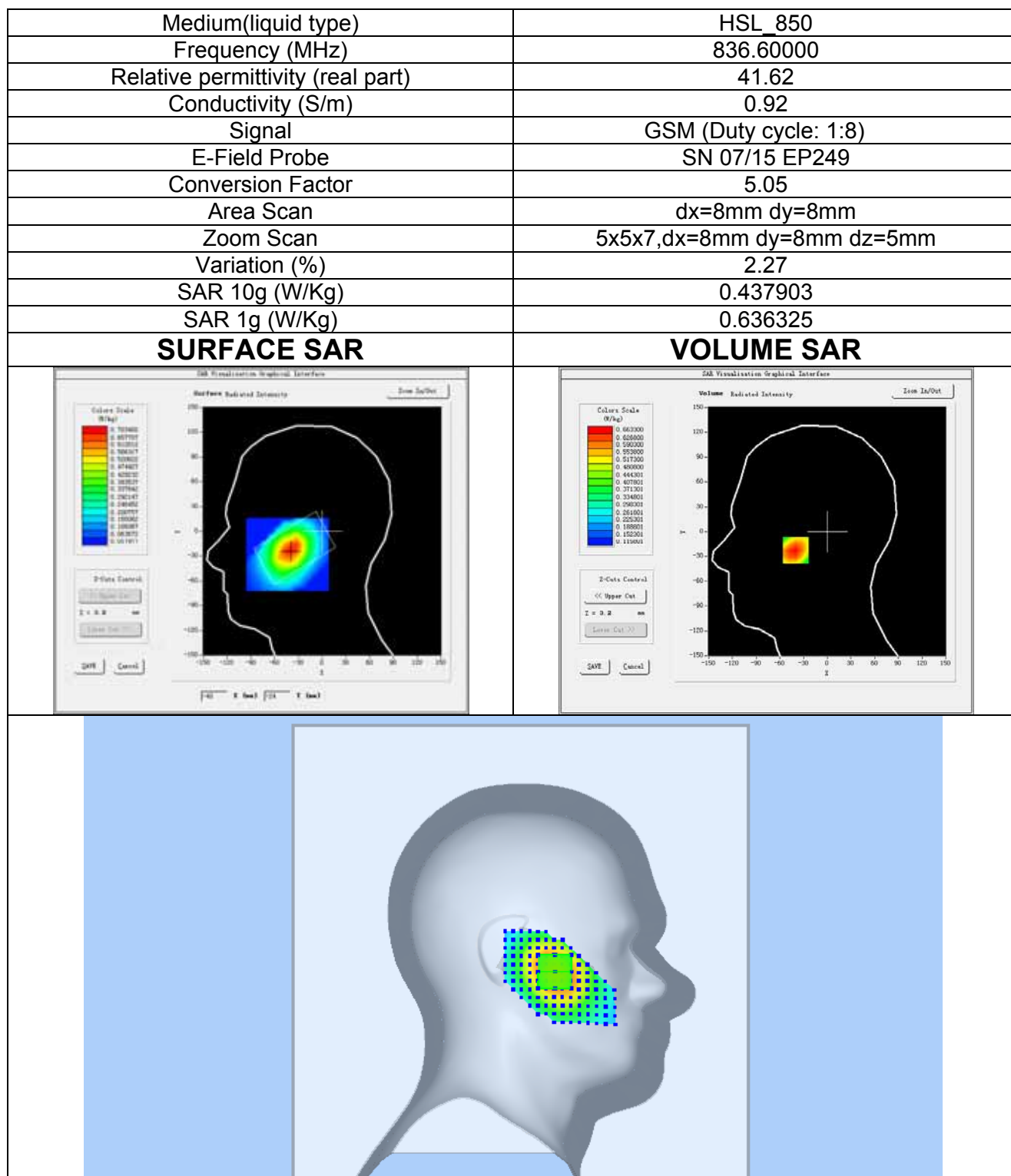
Plot 4: GSM850MHz, Mid channel (Left Head , Tilt) Product Description: GSM Mobile Phone Test Date:Jul 25,2017
