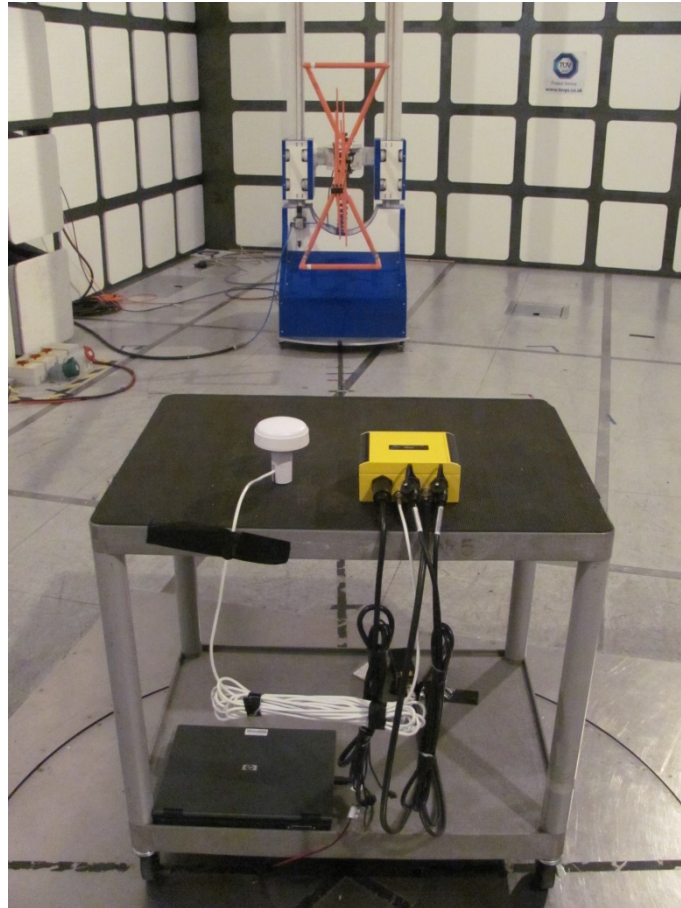
FCC Part 15B Radiated Emissions 30 MHz to 2 GHz
