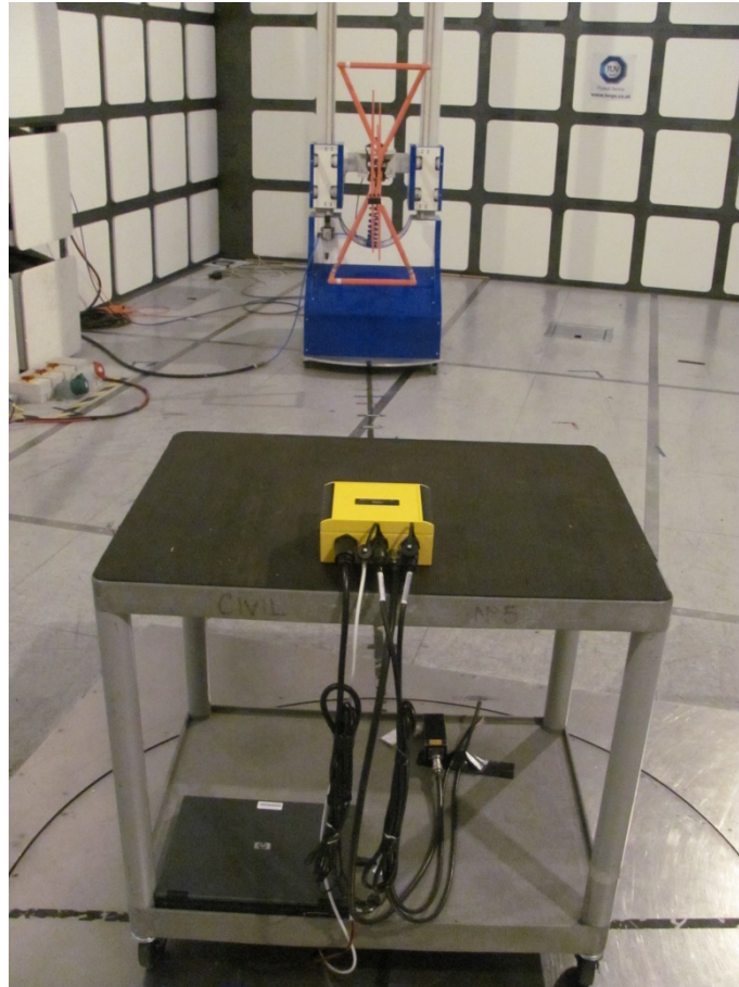
FCC Part 80 Radiated Emissions 30 MHz to 2 GHz
