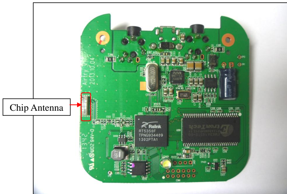
Bottom view of main PCB
