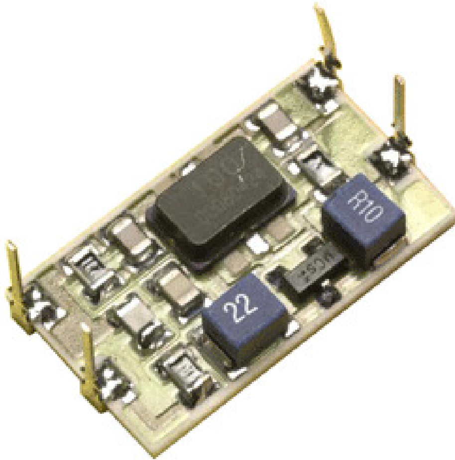
Photo 3 – Top View of the AM Transmitter Module 1
