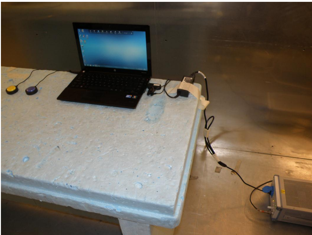
Photograph 2. Conducted emissions at mains ports.
