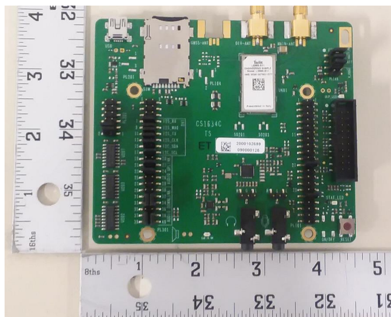
Figure B2. DUT Top View
