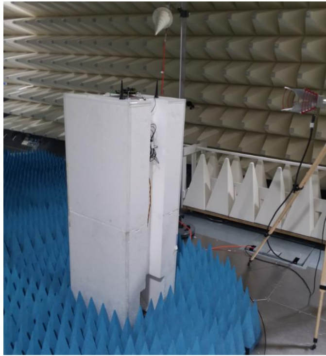
Figure B5. Radiated Setup HR
