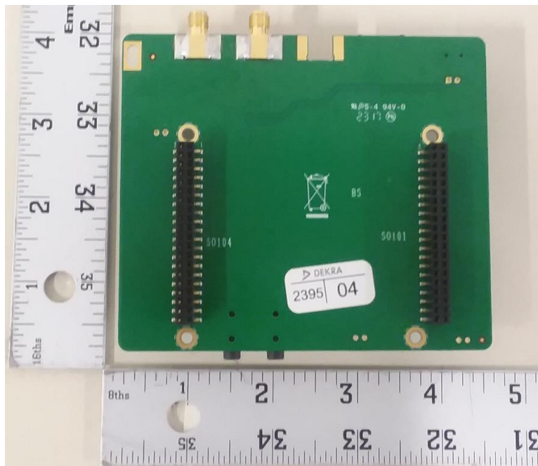
Figure B3. DUT Rear View
