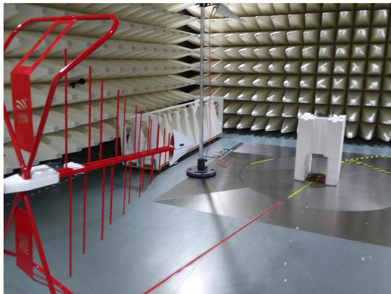
Figure B4. Radiated Setup LR
