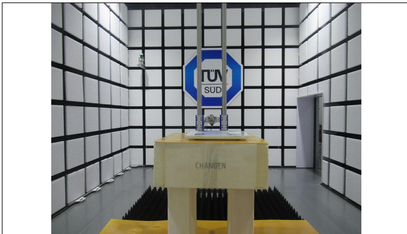
Radiated Emission test (18000MHz to 26000MHz)
