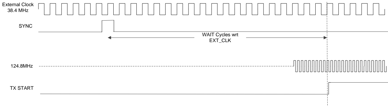
Figure 23: Synchronised Transmission
