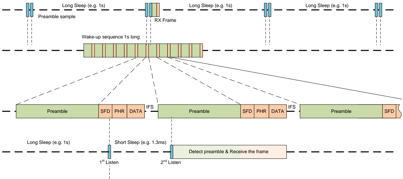
Figure 15: Low power listening with two sleep times
