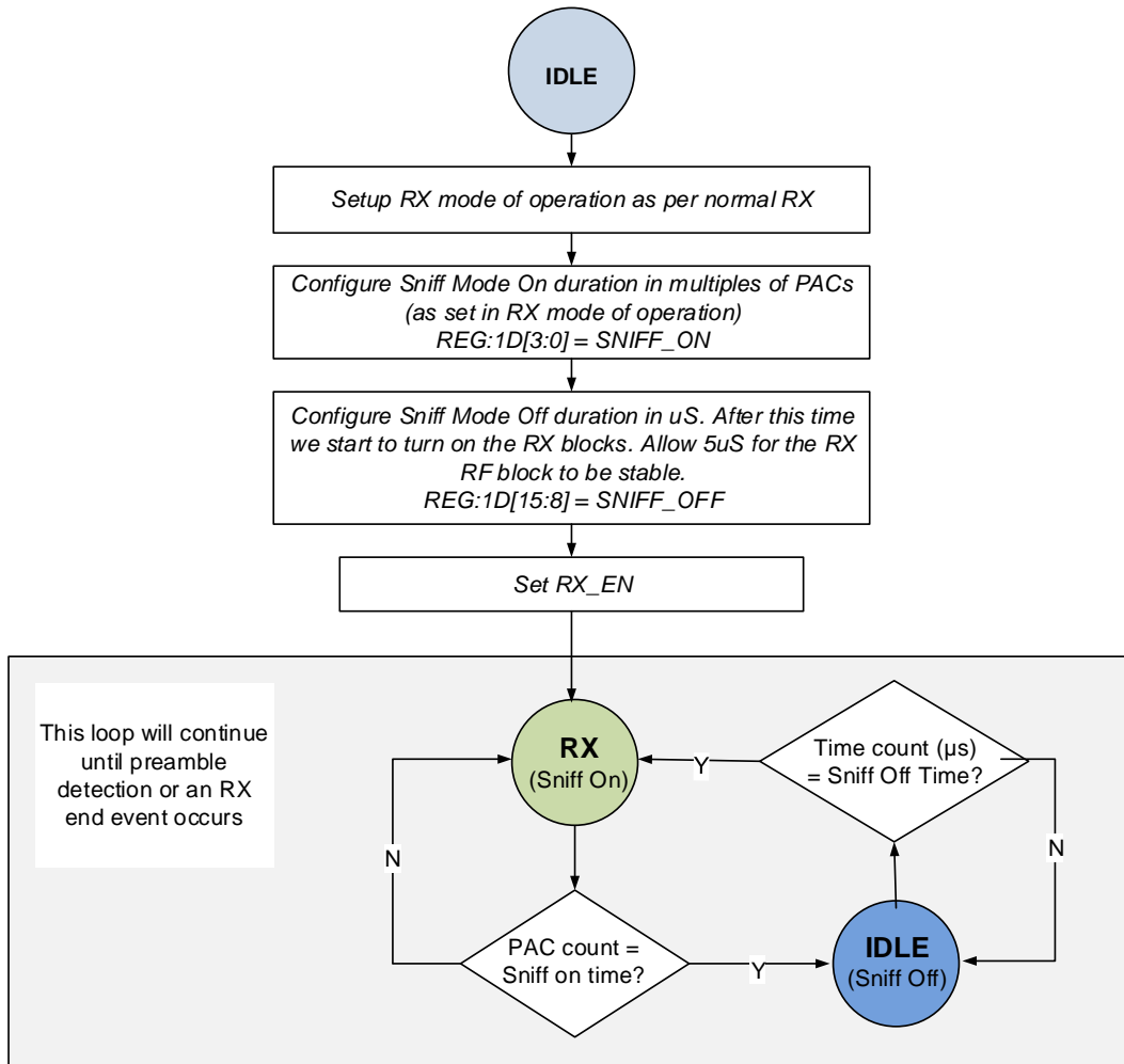
Figure 17: State transitions during SNIFF mode
