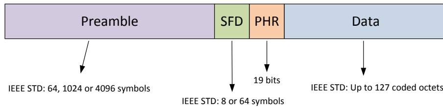
Figure 30: UWB PHY Frame structure
