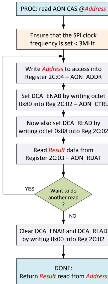
Figure 27: Flow chart for direct read of AON address
