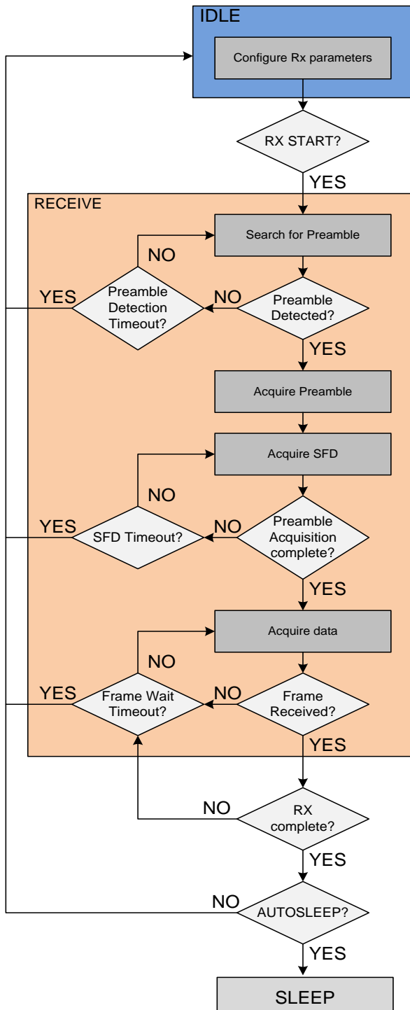
Figure 12: Basic receive sequence
