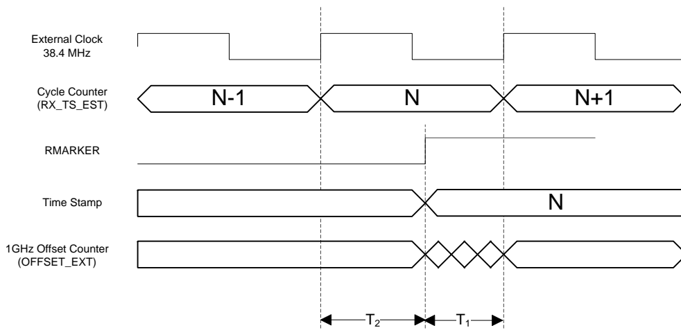
Figure 24: OSRS Mode Receive Timebase Synchronisation
