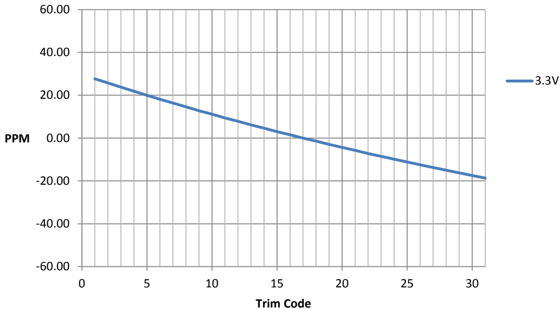
Figure 28: PPM vs Crystal Trim Setting, V BATT = 3.3 V
