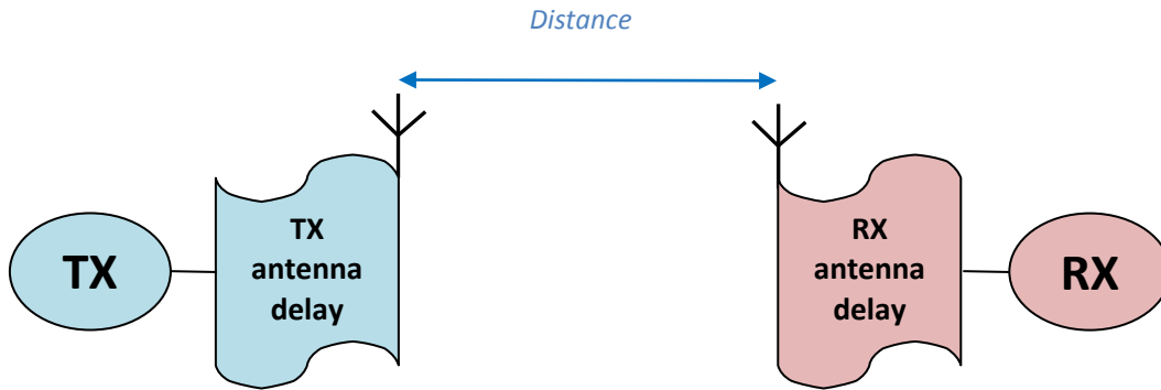
Figure 29: Transmit and Receive Antenna Delay
