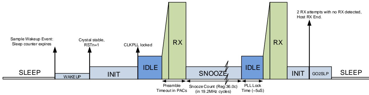
Figure 16: Power profile for low power listening mode where no frame is received
