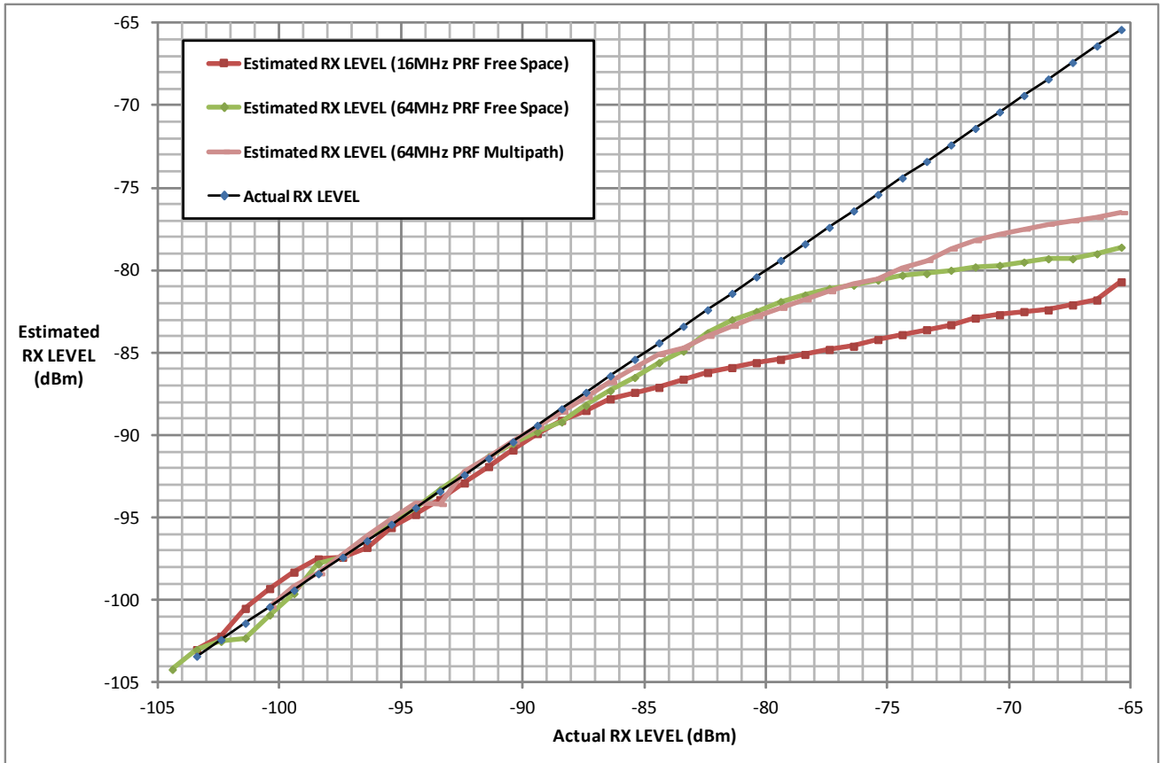
Figure 21: Estimated RX level versus actual RX level
