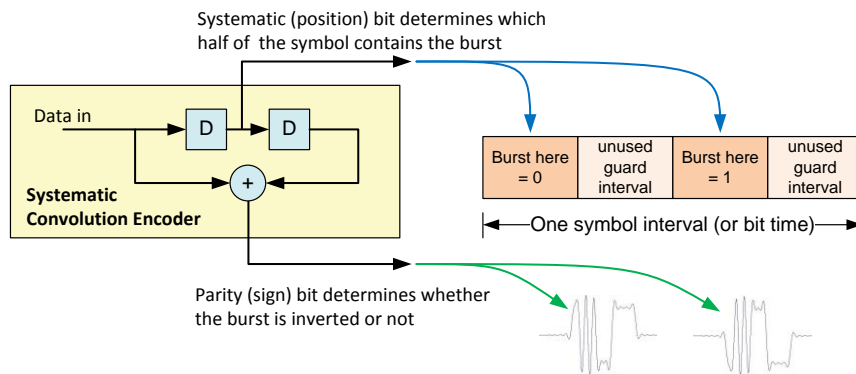
Figure 31:- BPM/BPSK data and PHR modulation
