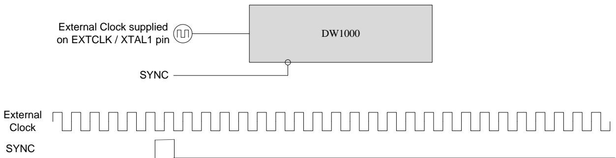
Figure 22: DW1000 External Synchronisation Interface
