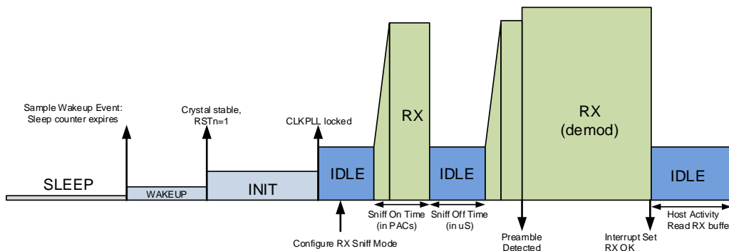
Figure 19: Power profile for SNIFF where a frame is received
