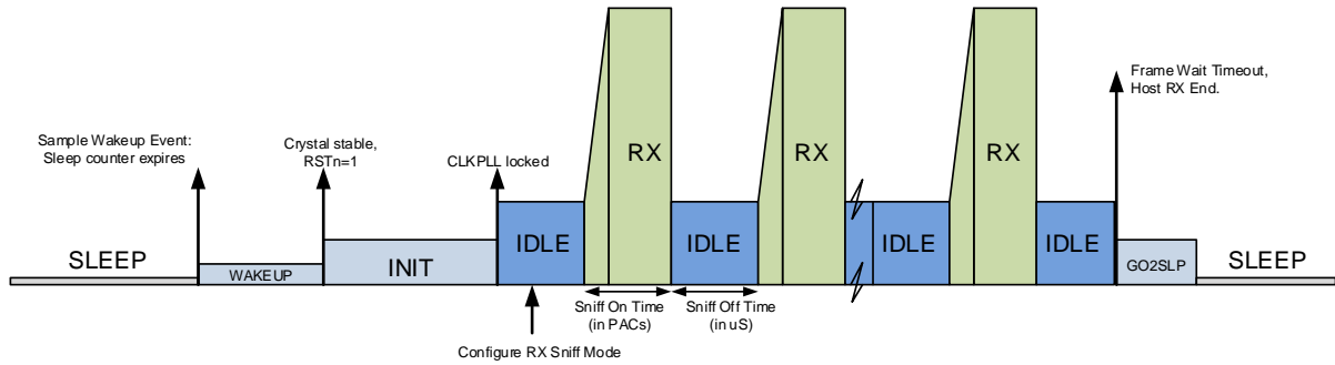
Figure 18: Power profile for SNIFF where a frame is not received
