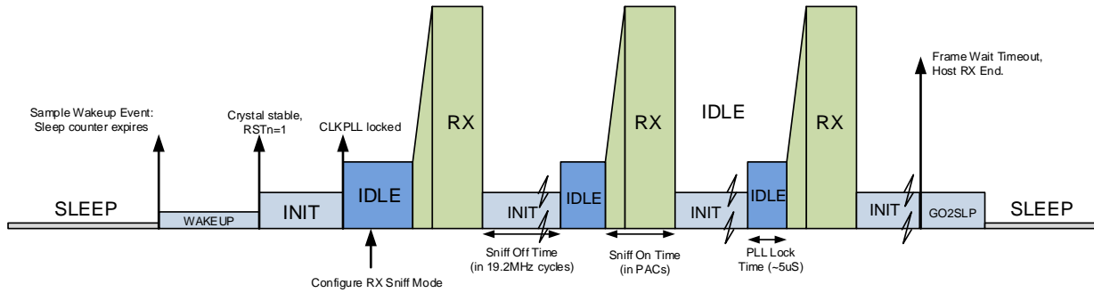
Figure 20: Power profile for Low duty-cycle SNIFF where a frame is not received
