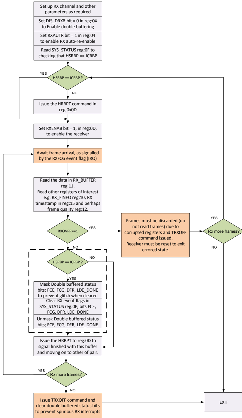
Figure 13: Flow chart for using double RX buffering
