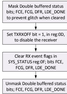
Figure 14 : TRXOFF in Double-Buffered Mode
