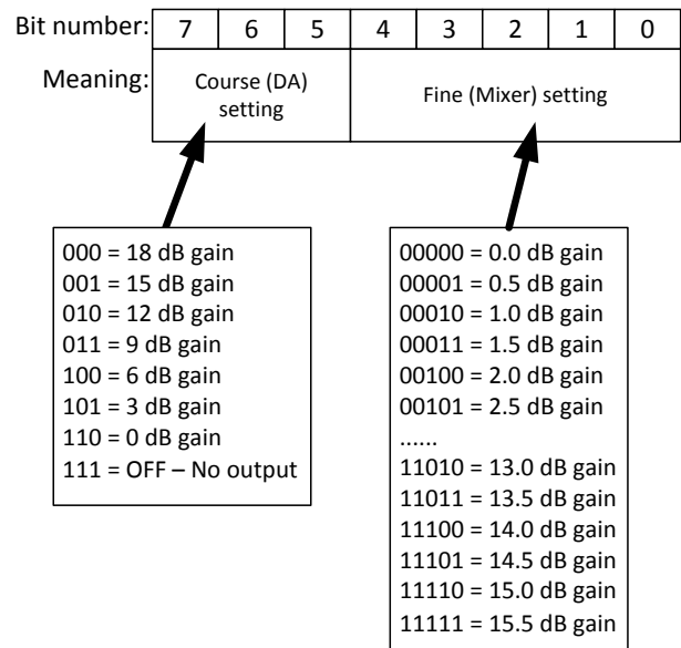
Figure 25: Transmit power control octet
