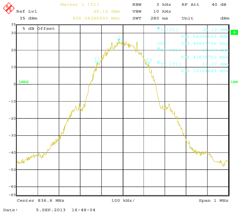
99% Occupied Bandwidth
