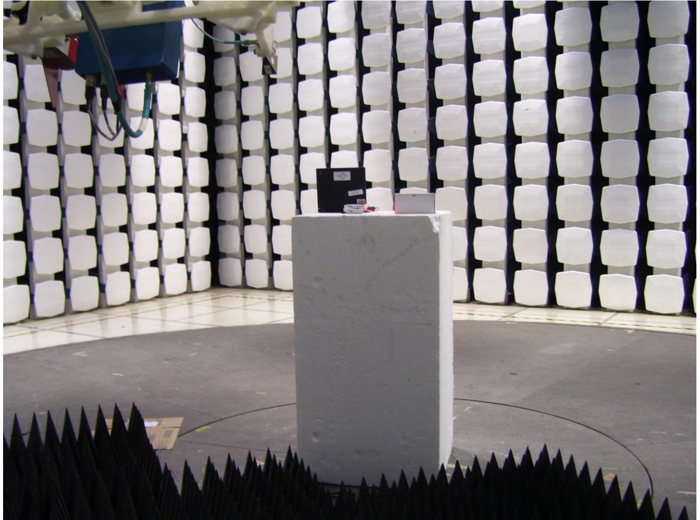
Figure 3: ANSI C63.10:2013 Setup Front
