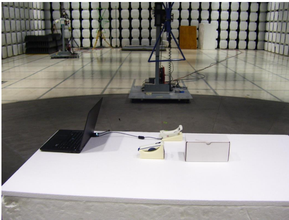
Figure 5: 30-1000 MHz Emissions setup
