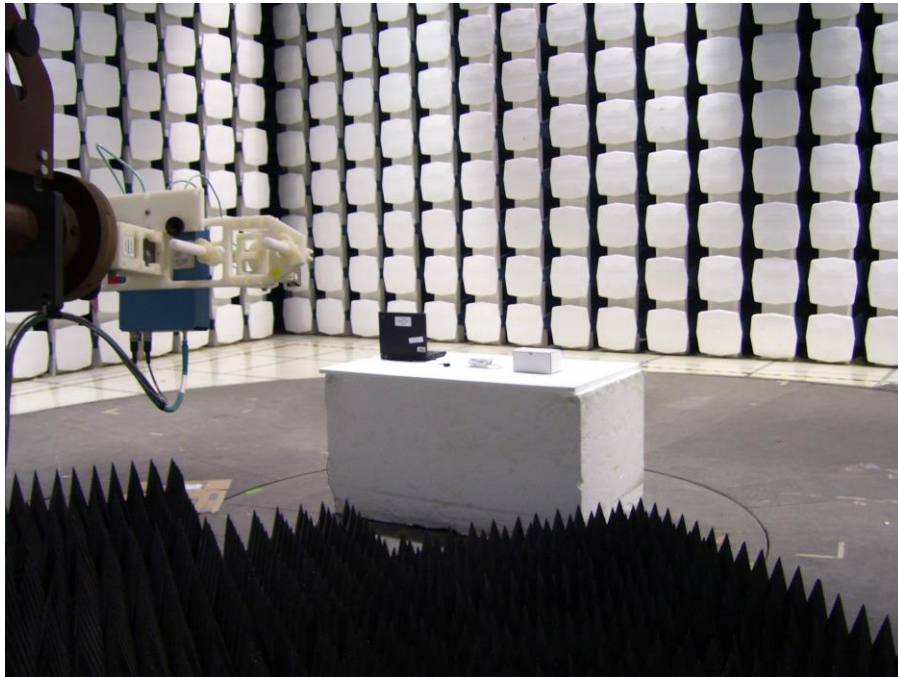
Figure 1: ANSI C63.10:2009 Setup Front
