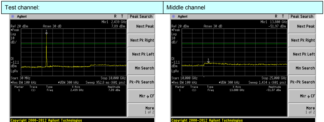
30MHz~10GHz
