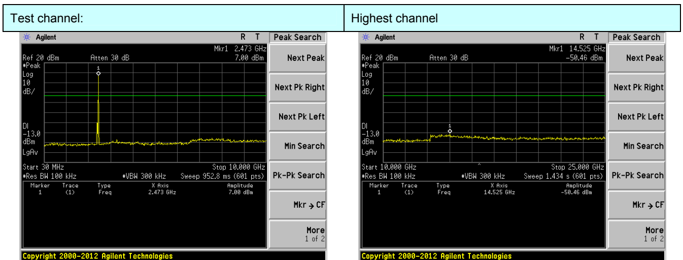
30MHz~10GHz
