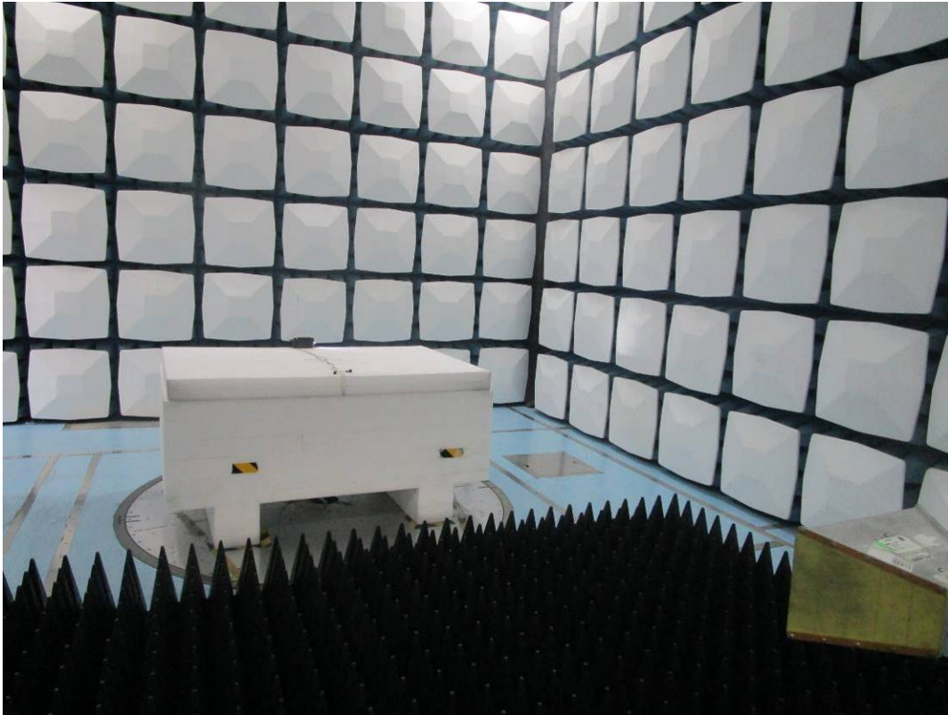
Radiated Emissions Above 1G rear View M2-M11
