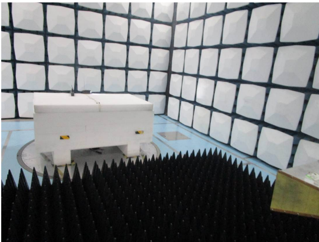
Radiated Emissions Above1G rear View M12
