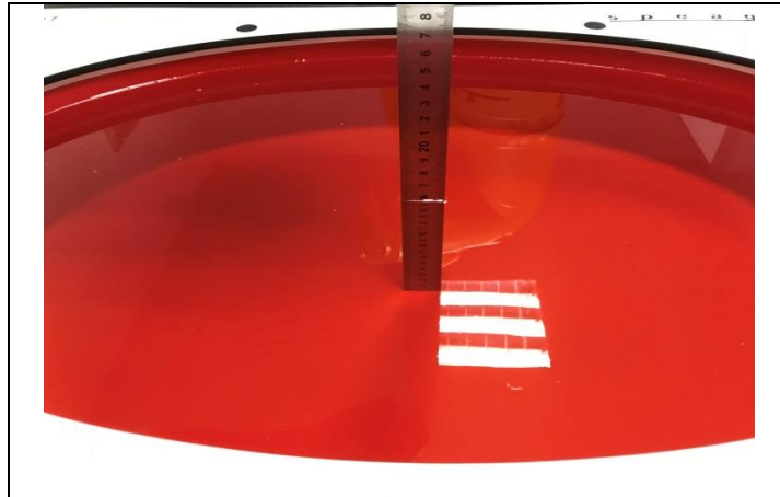
Liquid depth in the flat Phantom (150MHz) (15.3cm deep)
