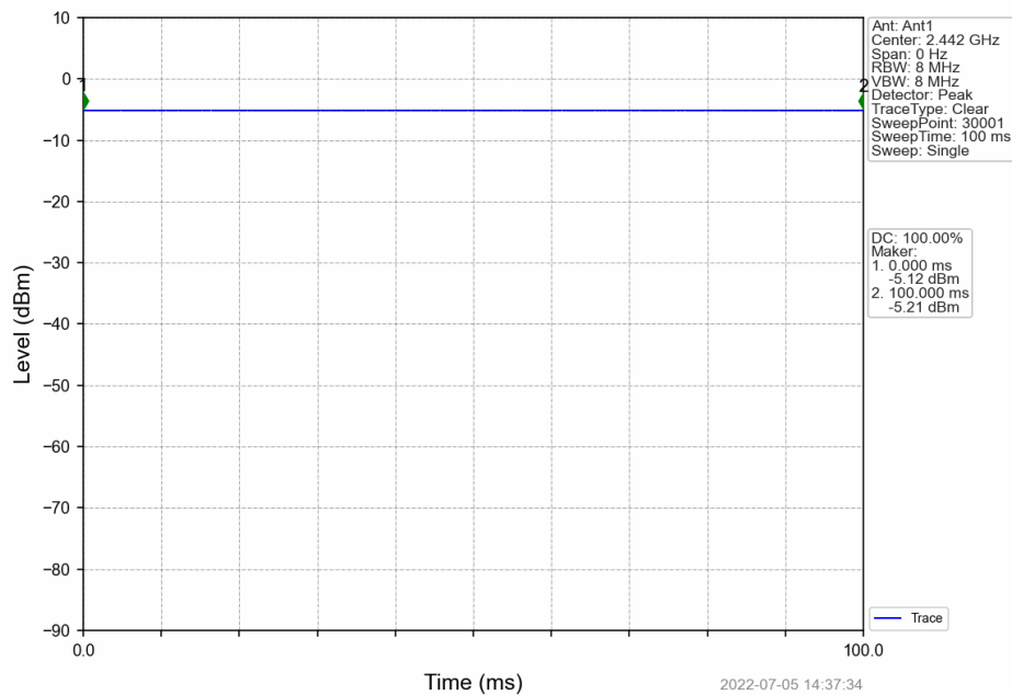
GFSK_MCH_2442MHz_Ant1_NTNV
