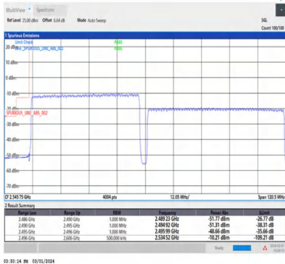
NTNV_CA_n41C_PC3_30+30_50+60_L+L_TID3_1_#1
