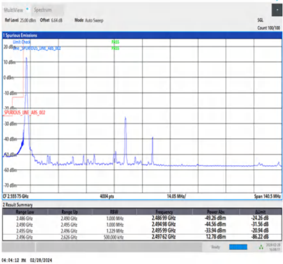
NTNV_CA_n41C_PC3_30+30_50+80_L+L_TID1_1_#1
