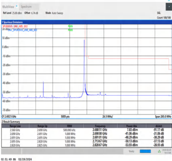
NTNV_CA_n41C_PC3_30+30_50+80_H+H_TID5_1_#1
