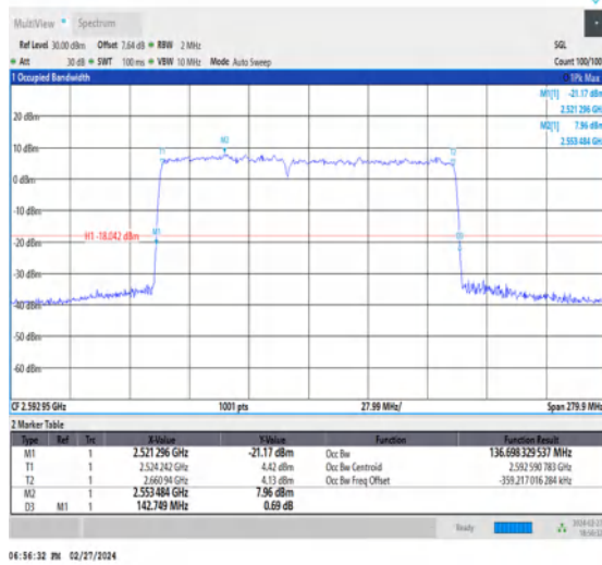
NTNV_CA_n41C_PC3_30+30_60+80_M+M_Ant1_TID4_1_#1
