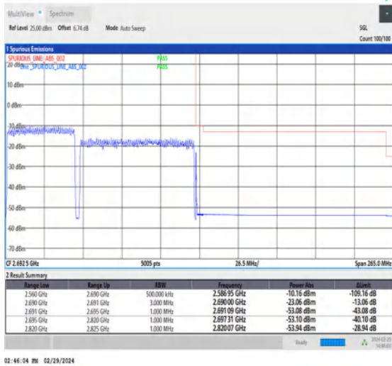
NTNV_CA_n41C_PC3_30+30_50+80_H+H_TID3_1_#1
