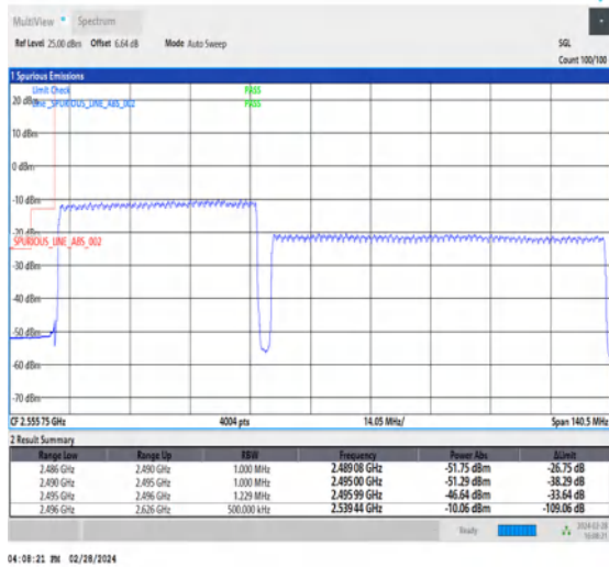
NTNV_CA_n41C_PC3_30+30_50+80_L+L_TID3_1_#1
