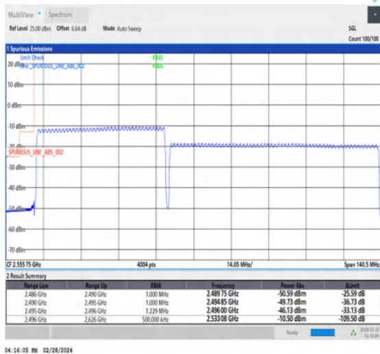
NTNV_CA_n41C_PC3_30+30_50+80_L+L_TID6_1_#1
