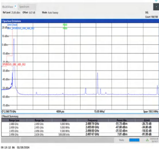
NTNV_CA_n41C_PC3_30+30_80+60_L+L_TID4_1_#1
