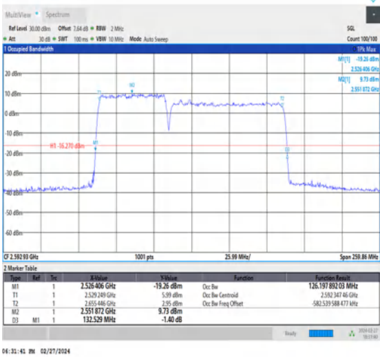
NTNV_CA_n41C_PC3_30+30_50+80_M+M_Ant1_TID6_1_#1
