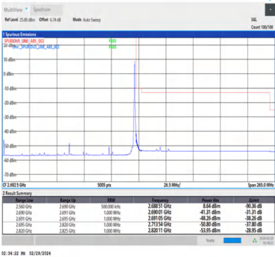
NTNV_CA_n41C_PC3_30+30_50+80_H+H_TID2_1_#1
