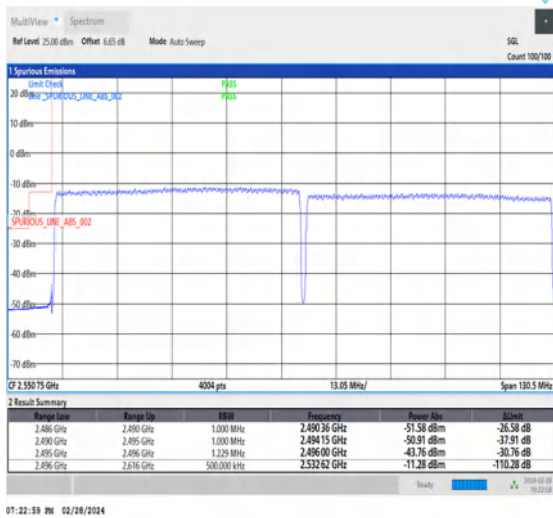
NTNV_CA_n41C_PC3_30+30_60+60_L+L_TID3_1_#1
