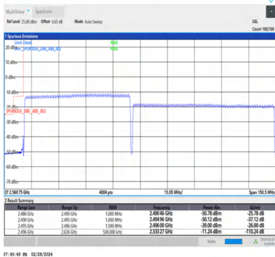
NTNV_CA_n41C_PC3_30+30_60+80_L+L_TID6_1_#1
