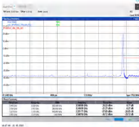
1-N78-3450-3550-30-90-H-5-CP-QPSK-Edge_1RB_Right-1@244-Ant0-1--PASS-see graph
