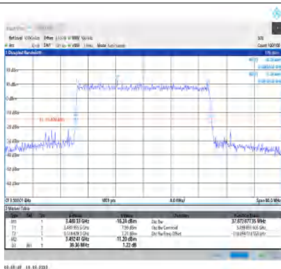
1-N78-3450-3550-30-40-M-6-CP-QPSK-Outer_Full- 106@0-Ant0-37.873-39.360-≤40-PASS
