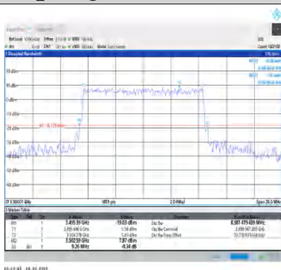
1-N78-3450-3550-30-10-M-6-CP-QPSK-Outer_Full- 24@0-Ant0-8.581-9.260-≤10-PASS
