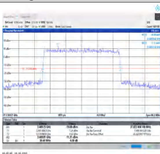
1-N78-3450-3550-30-40-M-8-CP-64QAM-Outer_Full- 106@0-Ant0-37.872-39.440-≤40-PASS
