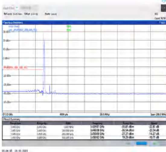
1-N78-3450-3550-30-15-L-4-CP-QPSK-Edge_1RB_Left-1@0-Ant0-1--PASS-see graph
