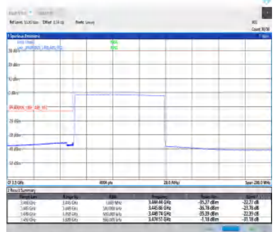
1-N78-3450-3550-30-70-L-6-CP-QPSK-Outer_Full-189@0-Ant0-1--PASS-see graph
