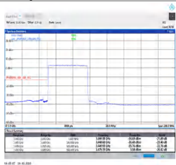
1-N78-3450-3550-30-50-L-3-DFT-PI2BPSK-Outer_Full-128@0-Ant0-1--PASS-see graph
