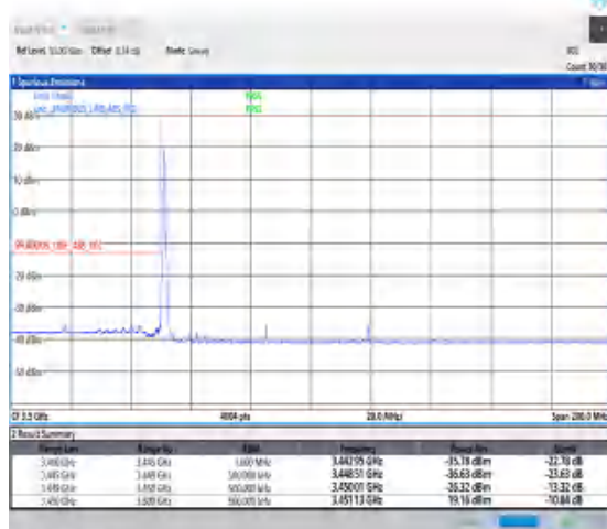
1-N78-3450-3550-30-70-L-4-CP-QPSK-Edge_1RB_Left-1@0-Ant0-1--PASS-see graph
