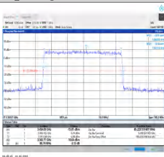
1-N78-3450-3550-30-90-M-5-DFT-256QAM- Outer Full-240@0-Ant0-85.226-88.740-≤90-PASS
