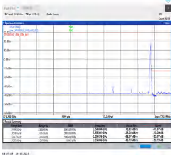
1-N78-3450-3550-30-40-H-5-CP-QPSK- Edge 1RB Right-1@105-Ant0-1--PASS-see graph
