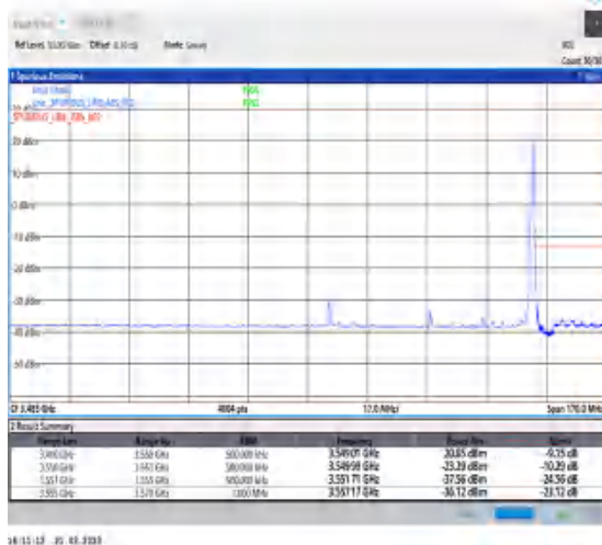
1-N78-3450-3550-30-60-H-5-CP-QPSK-Edge_1RB_Right-1@161-Ant0-1--PASS-see graph
