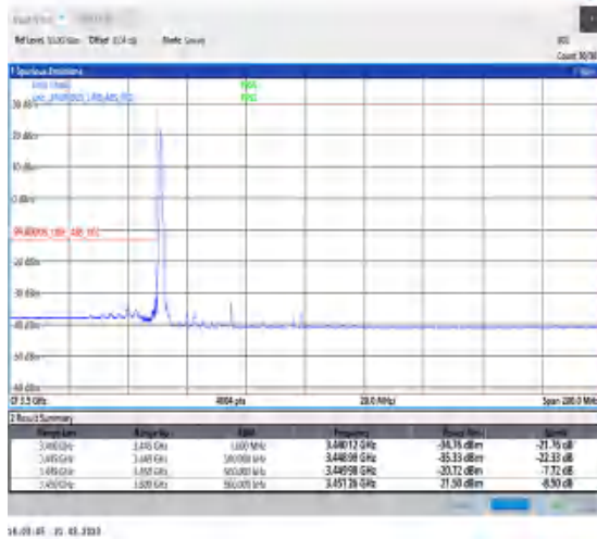
1-N78-3450-3550-30-50-L-4-CP-QPSK-Edge_1RB_Left-1@0-Ant0-1--PASS-see graph
