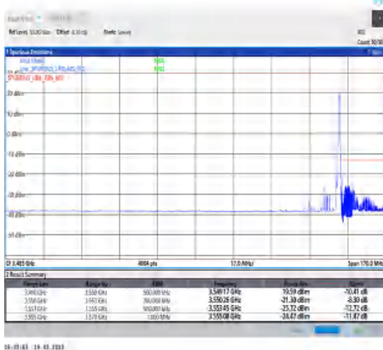
1-N78-3450-3550-30-15-H-5-CP-QPSK-Edge_1RB_Right-1@37-Ant0-1--PASS-see graph
