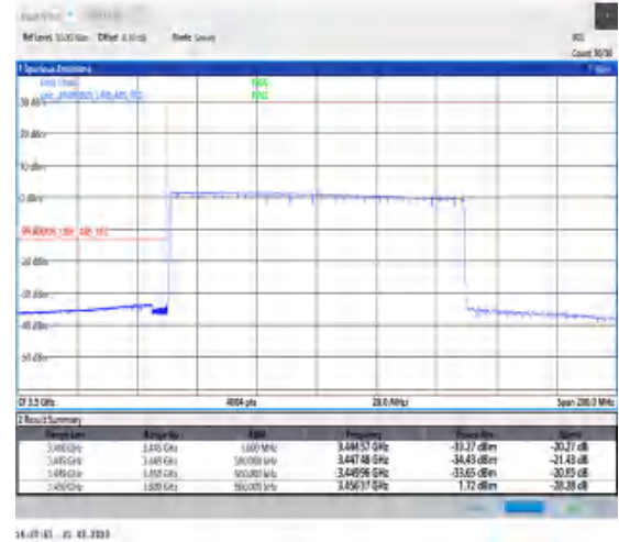
1-N78-3450-3550-30-100-L-6-CP-QPSK-Outer_Full-273@0-Ant0-1--PASS-see graph
