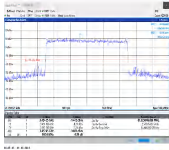
1-N78-3450-3550-30-90-M-8-CP-64QAM-Outer_Full-245@0-Ant0-87.329-90.540-≤90-PASS
