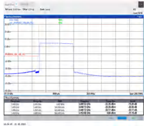
1-N78-3450-3550-30-50-L-6-CP-QPSK-Outer_Full-133@0-Ant0-1--PASS-see graph
