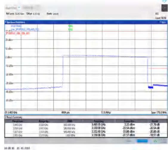
1-N78-3450-3550-30-90-H-6-CP-QPSK-Outer_Full-245@0-Ant0-1--PASS-see graph
