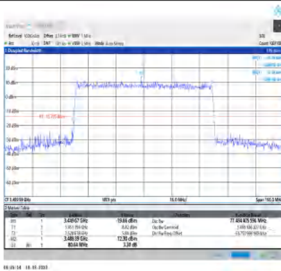
1-N78-3450-3550-30-80-L-7-CP-16QAM-Outer_Full-217@0-Ant0-77.484-80.640-≤80-PASS
