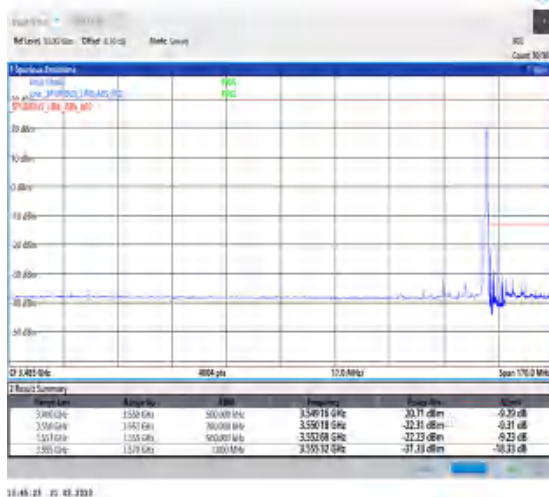
1-N78-3450-3550-30-15-H-5-CP-QPSK-Edge_1RB_Right-1@37-Ant0-1--PASS-see graph
