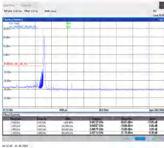
1-N78-3450-3550-30-70-L-4-CP-QPSK-Edge_1RB_Left-1@0-Ant0-1--PASS-see graph
