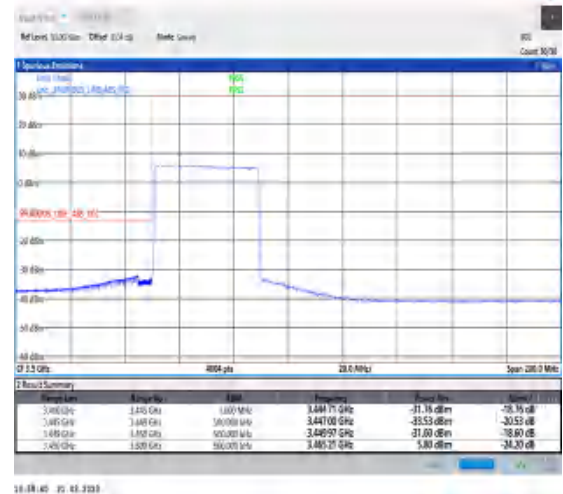
1-N78-3450-3550-30-40-L-6-CP-QPSK-Outer_Full-106@0-Ant0-1--PASS-see graph
