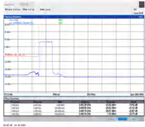
1-N78-3450-3550-30-20-L-3-DFT-PI2BPSK-Outer_Full-50@0-Ant0-1--PASS-see graph
