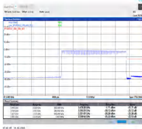
1-N78-3450-3550-30-80-H-6-CP-QPSK- Outer Full-217@0-Ant0-1--PASS-see graph
