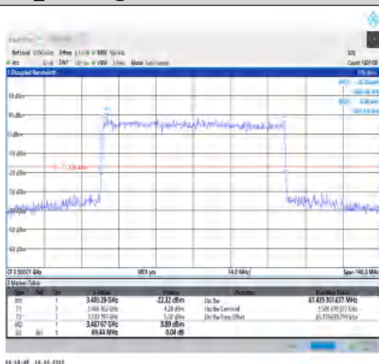
1-N78-3450-3550-30-70-M-7-CP-16QAM-Outer_Full- 189@0-Ant0-67.435-69.440-≤70-PASS
