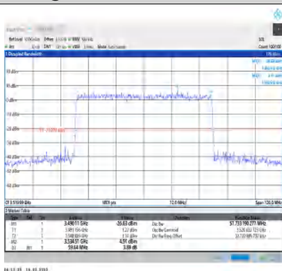
1-N78-3450-3550-30-60-H-9-CP-256QAM- Outer Full-162@0-Ant0-57.733-59.640-≤60-PASS
