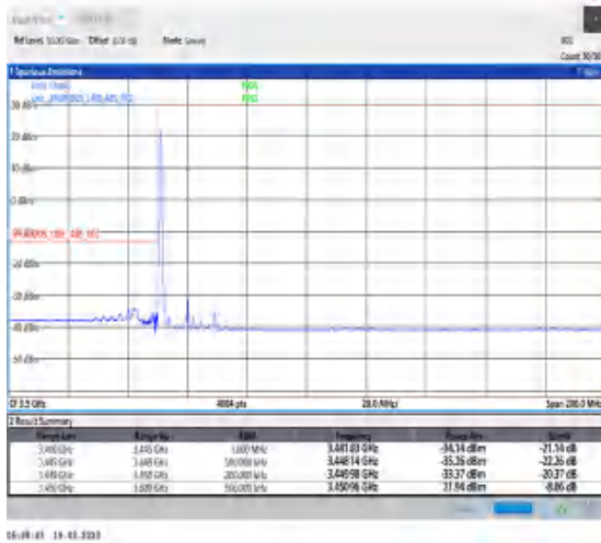
1-N78-3450-3550-30-20-L-1-DFT-PI2BPSK-Edge_1RB_Left-1@0-Ant0-1--PASS-see graph
