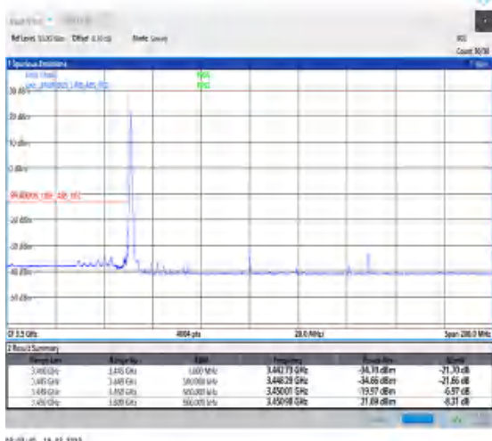
1-N78-3450-3550-30-100-L-1-DFT-PI2BPSK-Edge_1RB_Left-1@0-Ant0-1--PASS-see graph
