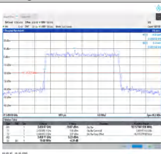
1-N78-3450-3550-30-20-L-9-CP-256QAM- Outer Full-51@0-Ant0-18.157-19.080-≤20-PASS
