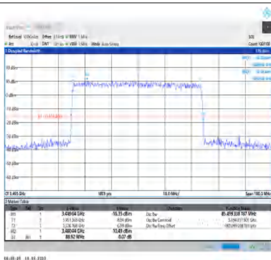
1-N78-3450-3550-30-90-L-4-DFT-64QAM- Outer Full-240@0-Ant0-85.499-88.920-≤90-PASS
