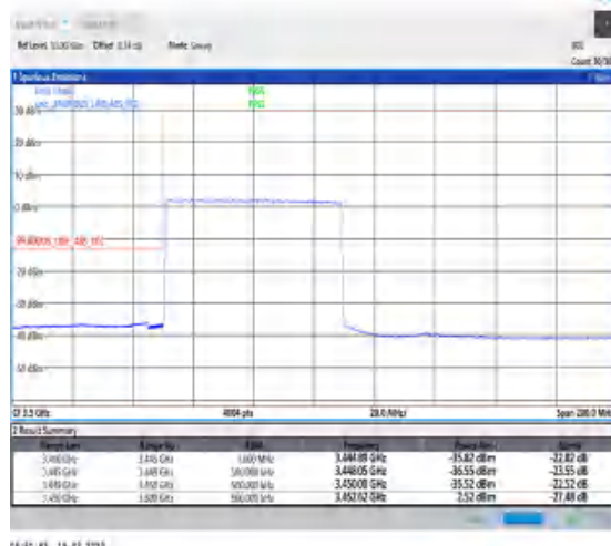
1-N78-3450-3550-30-60-L-3-DFT-PI2BPSK-Outer_Full-162@0-Ant0-1--PASS-see graph
