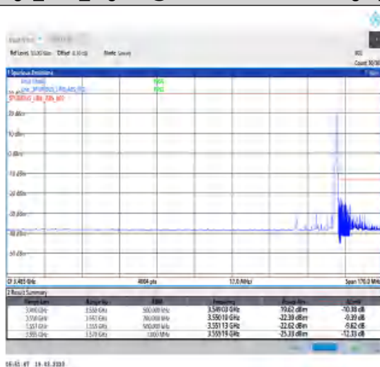
1-N78-3450-3550-30-20-H-5-CP-QPSK-Edge_1RB_Right-1@50-Ant0-1--PASS-see graph
