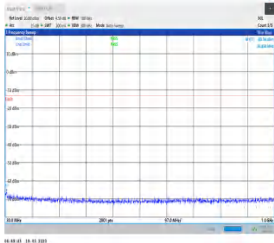
1-N78-3450-3550-30-100-L-1-DFT-PI2BPSK- Inner_1RB_Left-1@1-30-1000-Ant0-34.85--65.98-- 13-PASS
