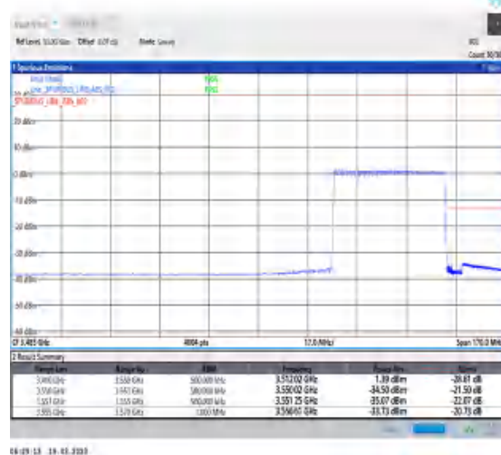
1-N78-3450-3550-30-40-H-6-CP-QPSK- Outer Full-106@0-Ant0-1--PASS-see graph
