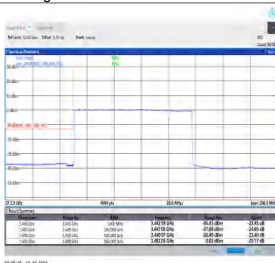
1-N78-3450-3550-30-90-L-3-DFT-PI2BPSK-Outer_Full-240@0-Ant0-1--PASS-see graph
