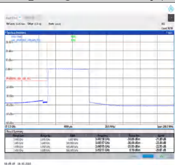
1-N78-3450-3550-30-50-L-6-CP-QPSK-Outer_Full-133@0-Ant0-1--PASS-see graph
