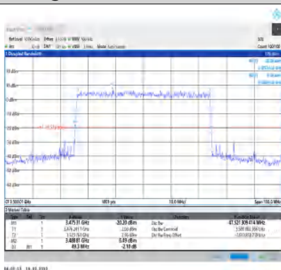
1-N78-3450-3550-30-50-M-9-CP-256QAM- Outer Full-133@0-Ant0-47.521-49.300-≤50-PASS
