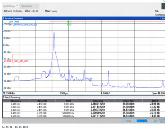
7-7-10MHz-20MHz-QPSK-QPSK-20805-20949-50RB#0-100RB#0
