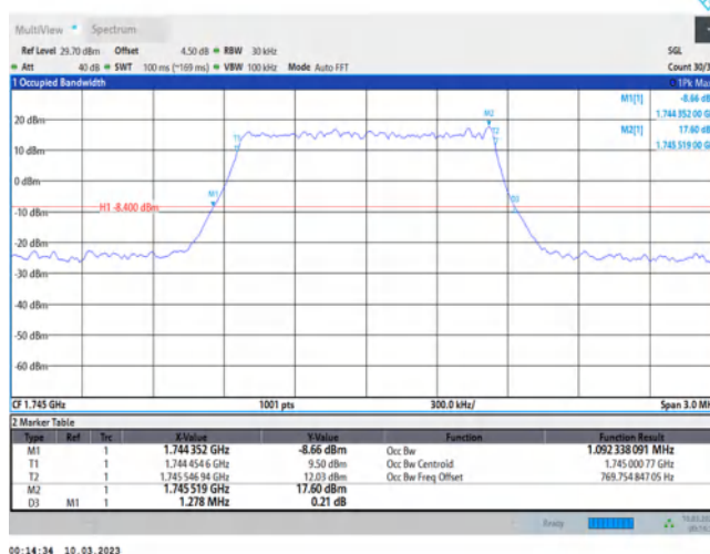
Band66-1.4MHz-QPSK-132322-6RB#0
