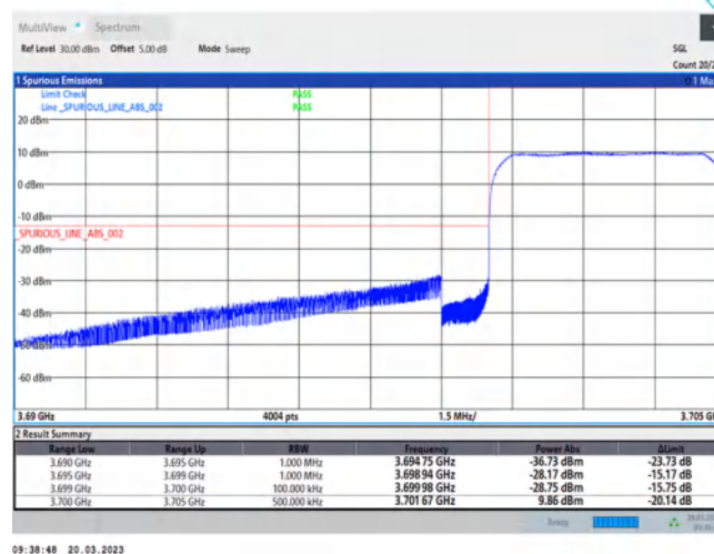
Band43-5MHz-QPSK-44615-25RB#0
