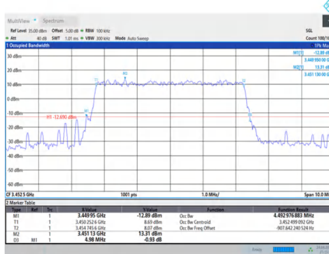
Band42-5MHz-QPSK-42590-25RB#0
