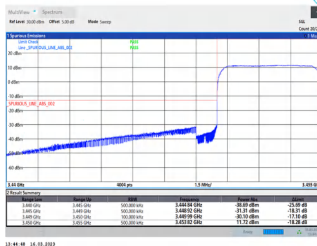
Band42-5MHz-QPSK-42115-25RB#0
