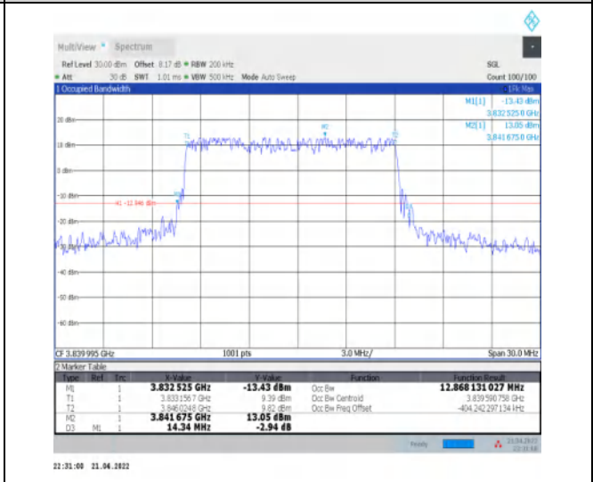
1-N77-3700-3980--30-15-M-4-DFT-64QAM-Outer_Full Full-36@0-Ant1-12.868-14.340≤15-PASS
