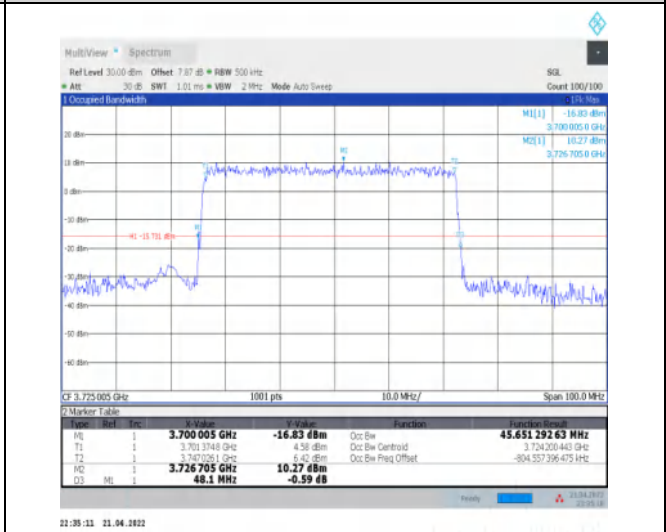
1-N77-3700-3980--30-50-L-5-DFT-256QAM-Outer_Full-128@0-Ant1-45.651-48.100-<math>\leq 50</math>-PASS
