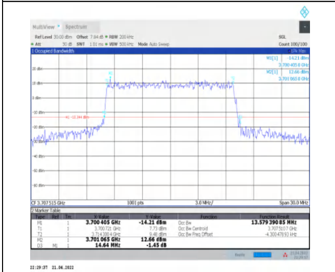
1-N77-3700-3980--30-15-L-8-CP-64QAM-Outer_Full-38@0-Ant1-13.579-14.640-≤15-PASS
