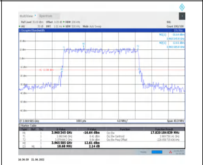
1-N77-3700-3980--30-20-H-4-DFT-64QAM-Outer_Full ll-50@0-Ant1-17.82-18.680-≤20-PASS
