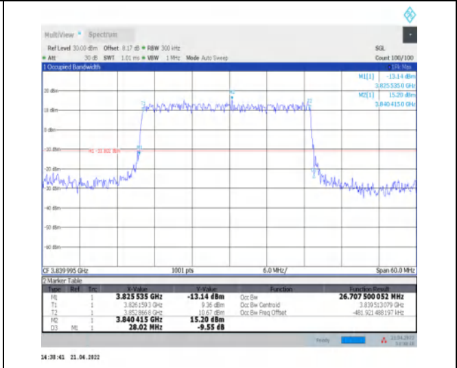
1-N77-3700-3980--30-30-M-2-DFT-PI2BPSK-Outer_Full Full-75@0-Ant1-26.71-28.020-<30-PASS
