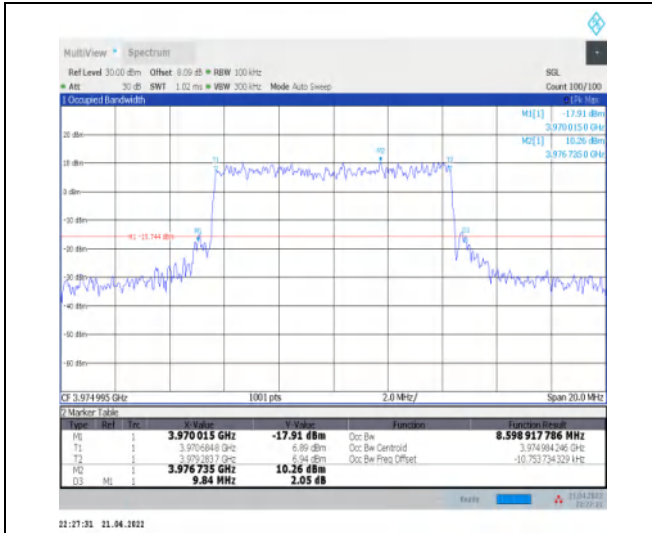
1-N77-3700-3980--30-10-H-7-CP-16QAM-Outer_Full -24@0-Ant1-8.599-9.840-≤10-PASS
