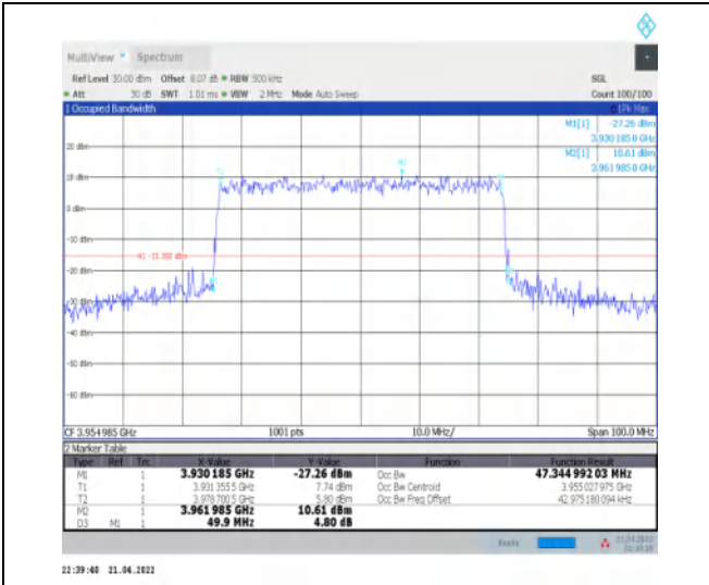
1-N77-3700-3980--30-50-H-8-CP-64QAM-Outer_Full -133@0-Ant1-47.345-49.900-≤50-PASS
