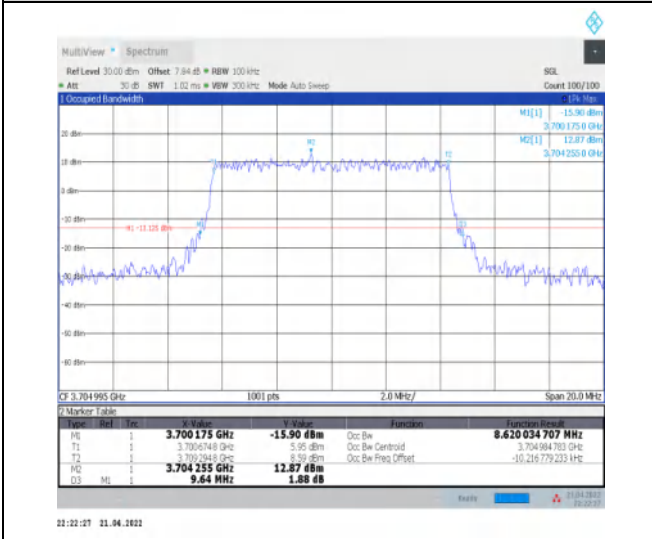
1-N77-3700-3980--30-10-L-3-DFT-16QAM-Outer_Full -24@0-Ant1-8.62-9.640-≤10-PASS
