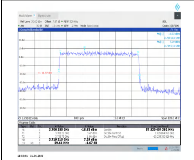
1-N77-3700-3980--30-60-L-9-CP-256QAM-Outer_Fu ll-162@0-Ant1-57.53-59.640-≤60-PASS
