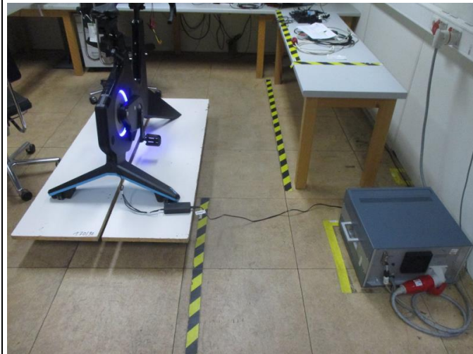
Conducted Emission test set up
