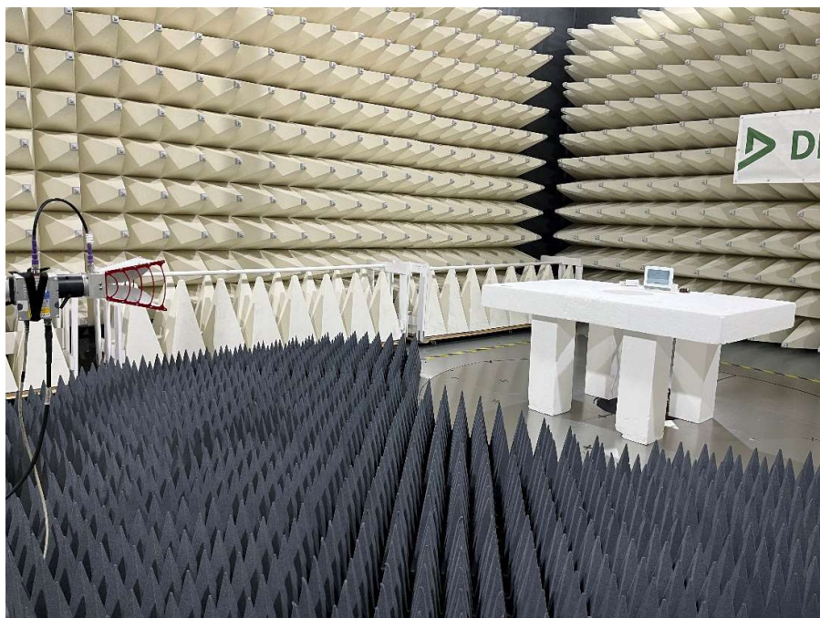
4. Radiated Emission test setup High Range
