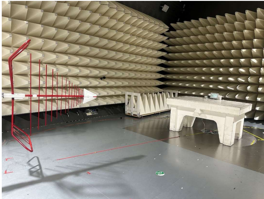
3. Radiated Emission test setup Low Range
