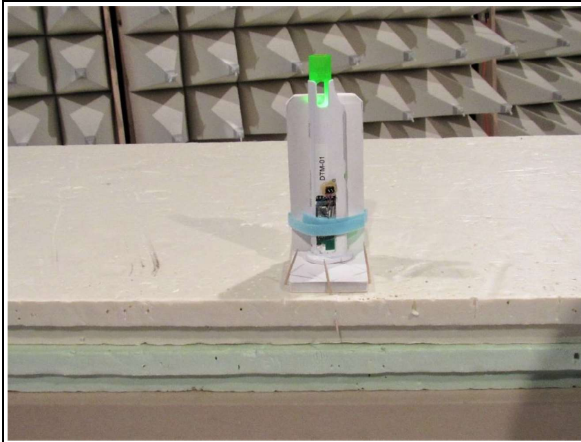
Test setup below 1GHz - C
