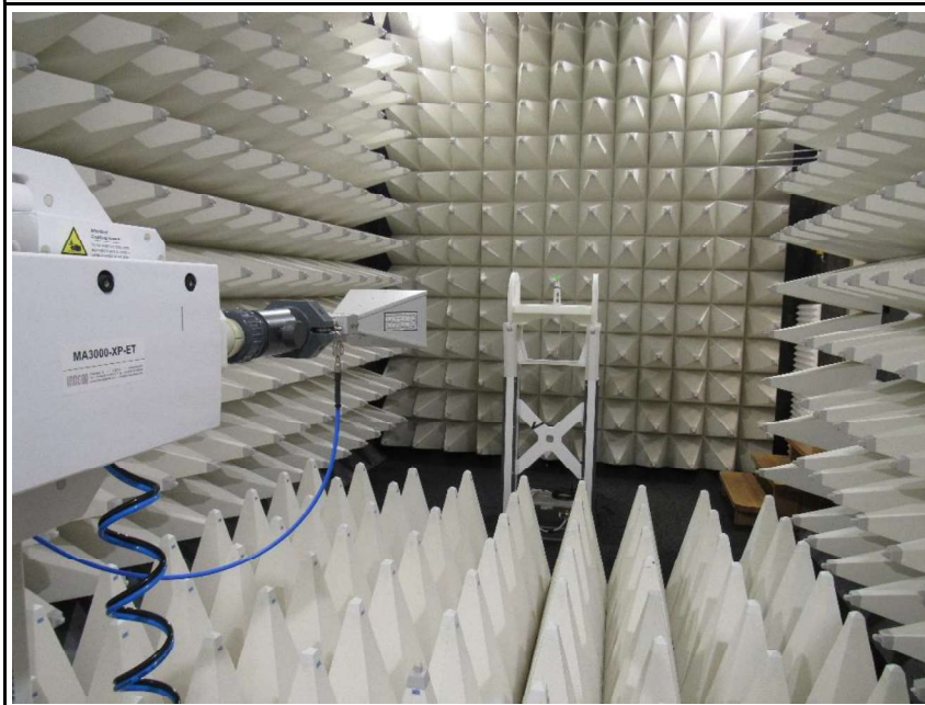
Test setup above 1GHz - A
