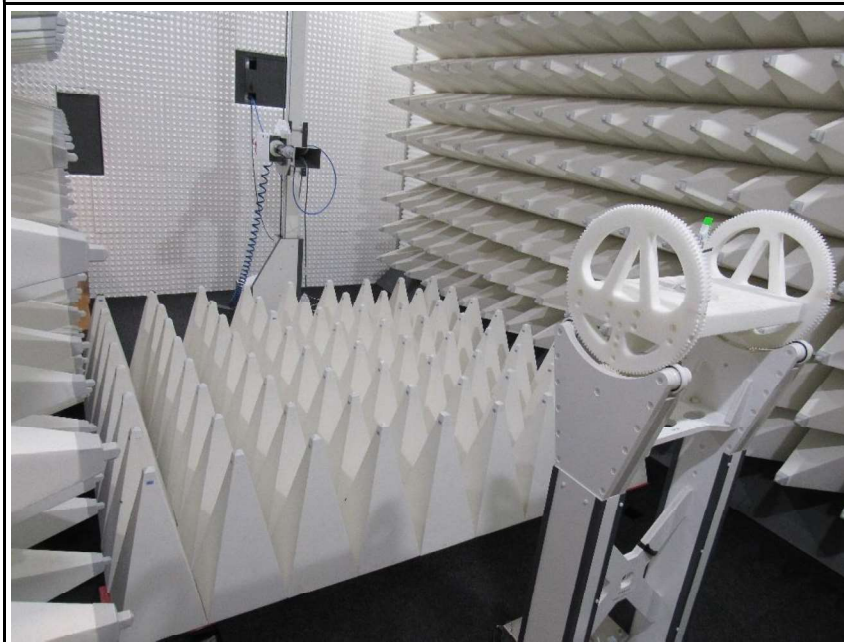
Test setup above 1GHz - B
