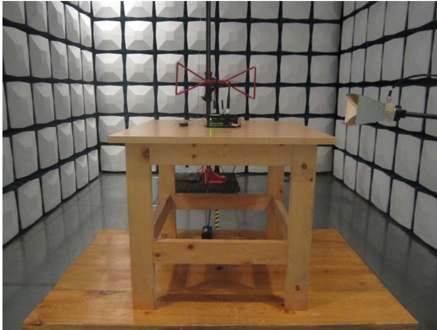
Radiated Emission View---Below 1G
