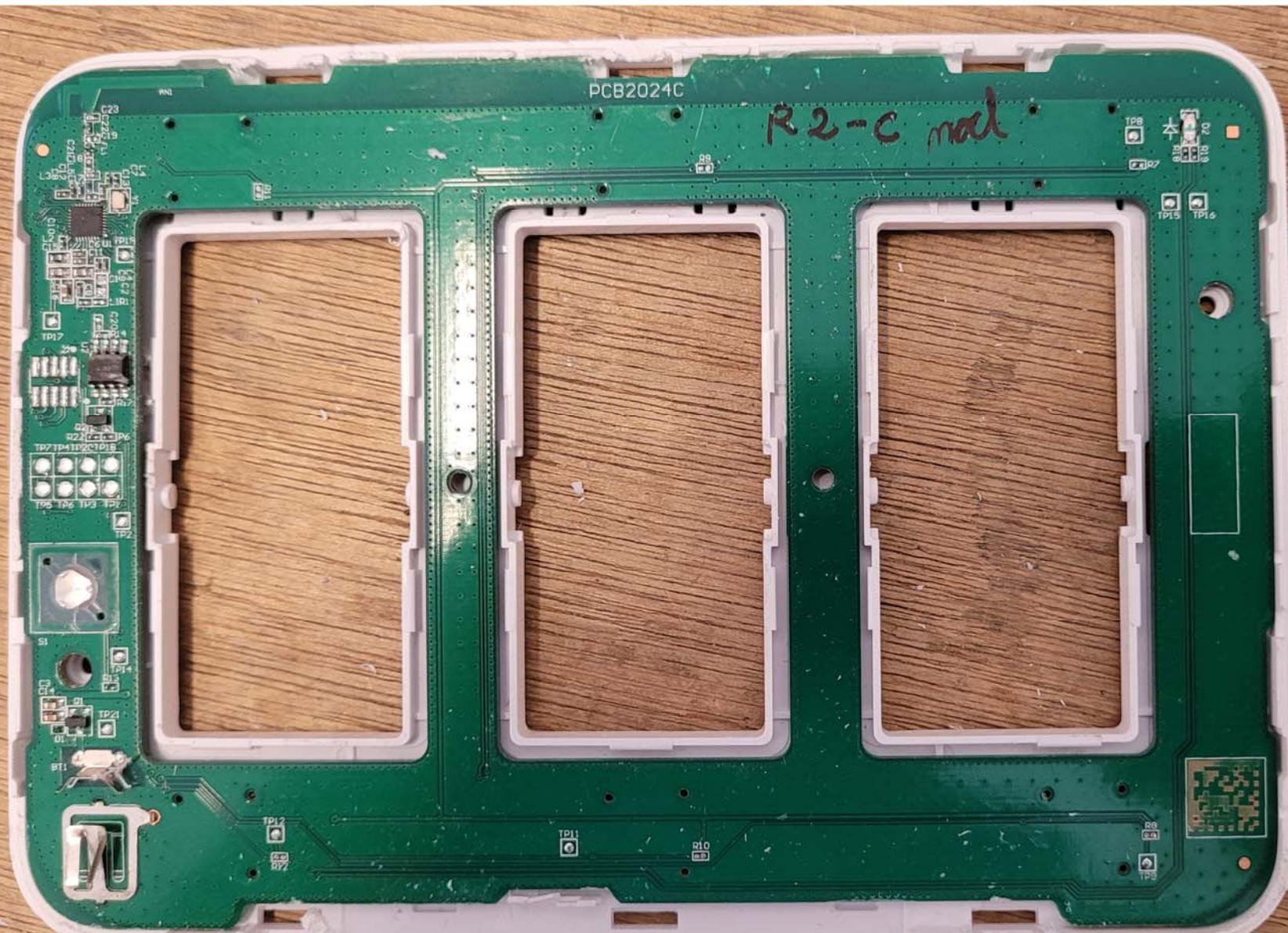
Top View of the PCB
