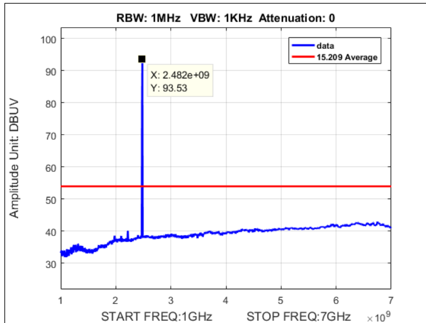
Plot 20. Average Radiated Spurious Emissions, BT, High Channel, 2480, 1-7 GHz
