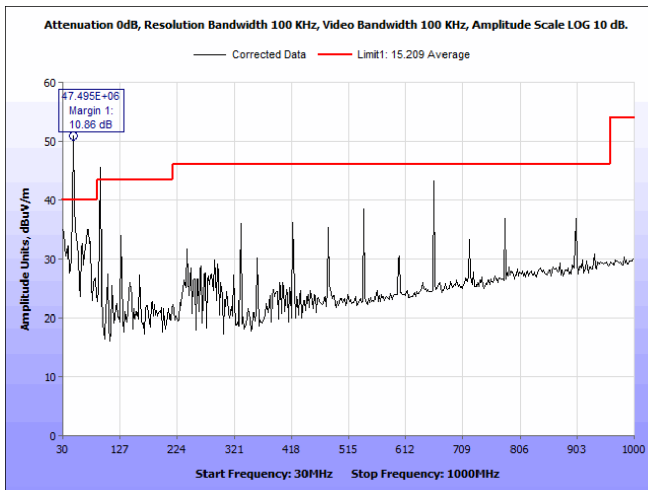
Plot 32. Radiated Emissions, High Channel, Below 1 GHz
