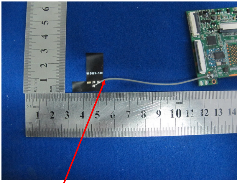
WiFi Antenna
