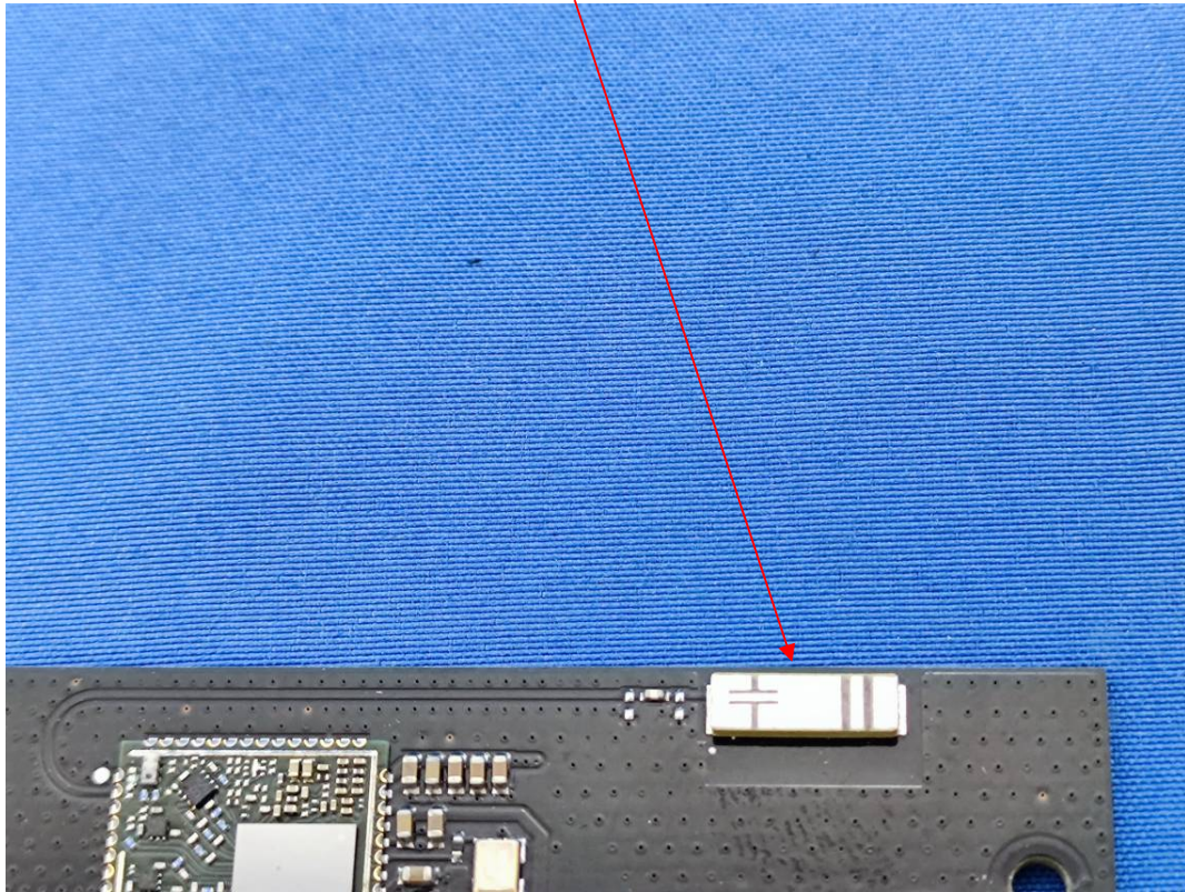
BT Antenna/ WIFI chain 0 Antenna
