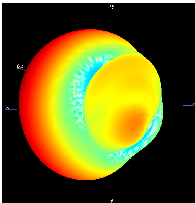
B1.1 3D Pattern for 2400MHz
