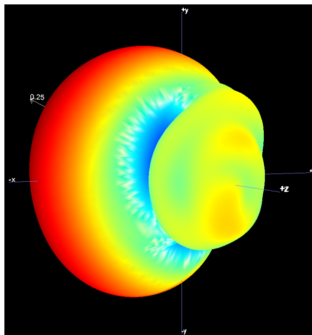
B1.2 3D Pattern for 2450MHz
