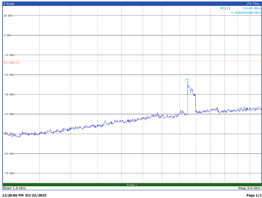
100 MHz signal, bottom channel, 1GHz – 3.6GHz – H Pol
