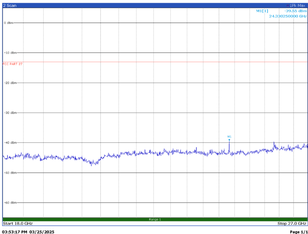
100 MHz signal, top channel, 18GHz – 27GHz – V Pol
