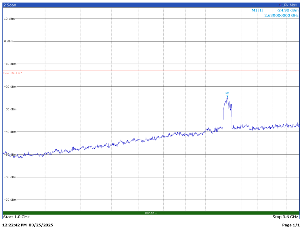
100 MHz signal, top channel, 1GHz – 3.6GHz – H Pol
