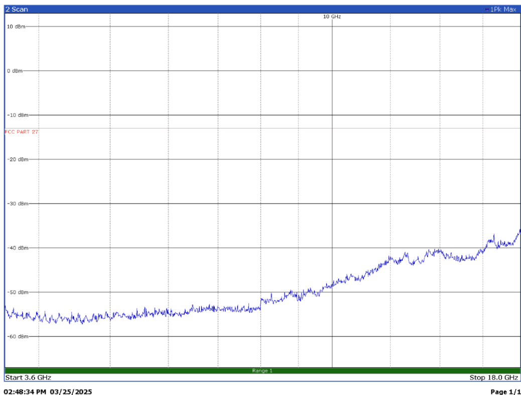
100 MHz signal, bottom channel, 3.6GHz – 18GHz – H Pol
