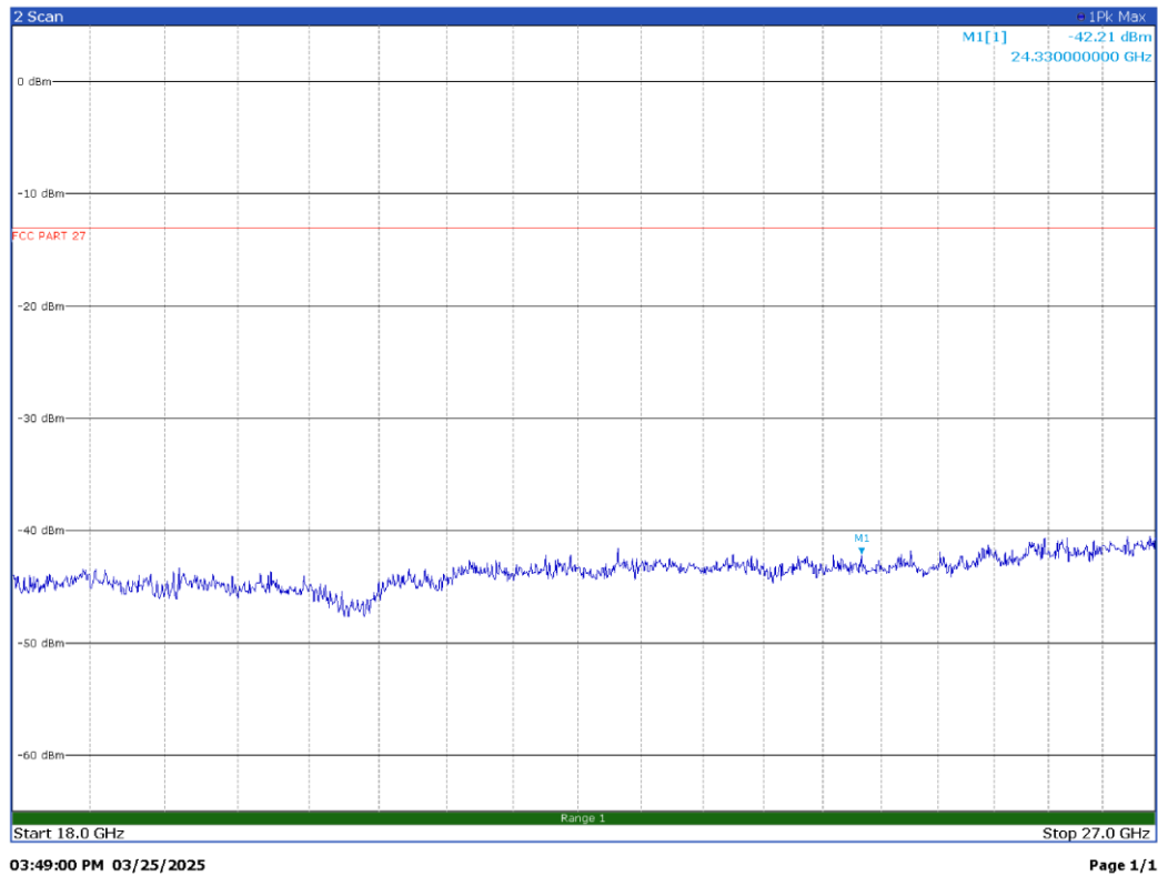
100 MHz signal, middle channel, 18GHz – 27GHz – H Pol
