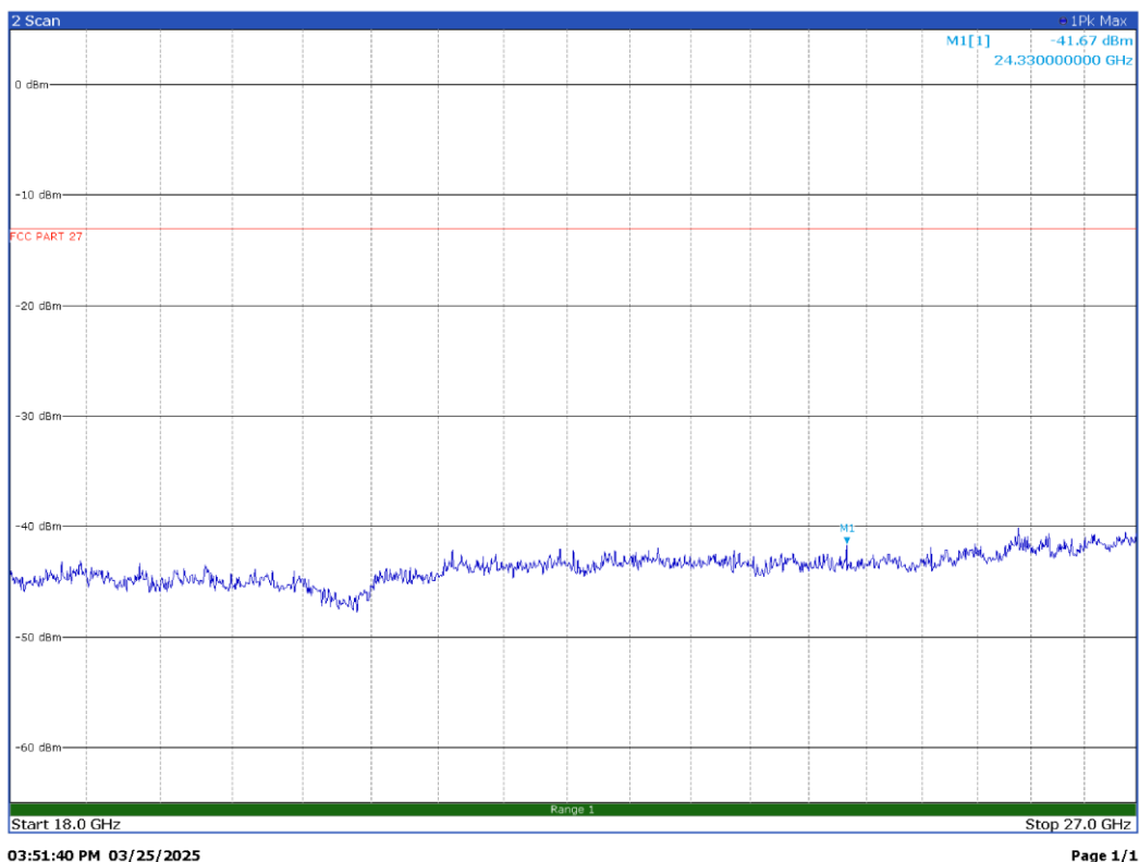
100 MHz signal, top channel, 18GHz – 27GHz – H Pol
