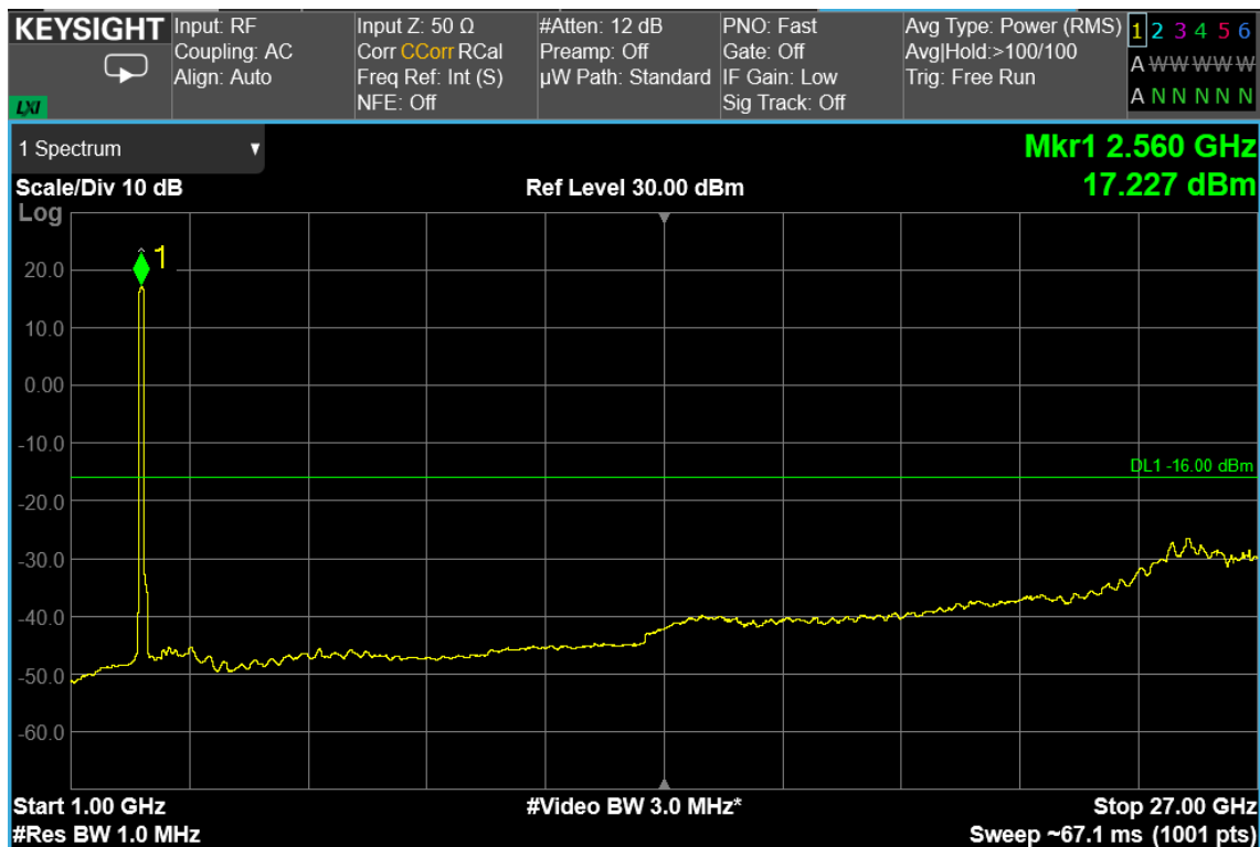
100 MHz signal, top channel, 1GHz – 27GHz
