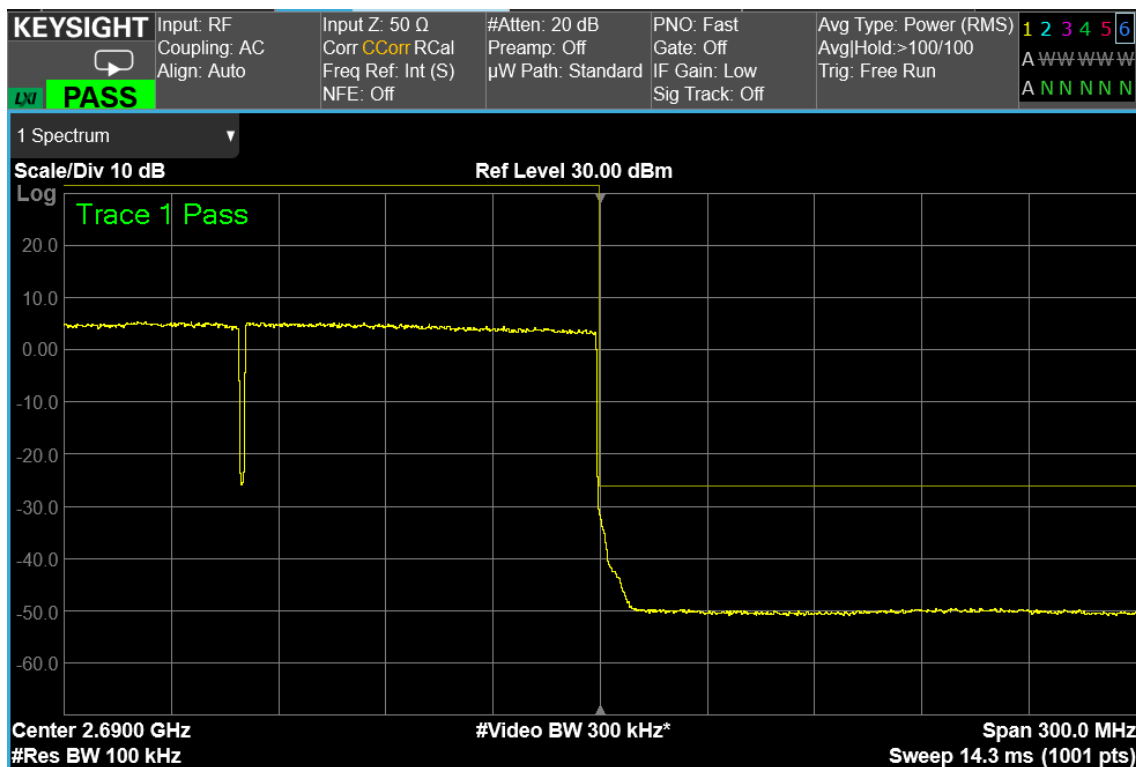
100+90 MHz signal, High Band Edge, 2 carrier, nominal input signal
