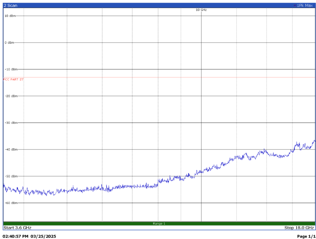
100 MHz signal, top channel, 3.6GHz – 18GHz – H Pol
