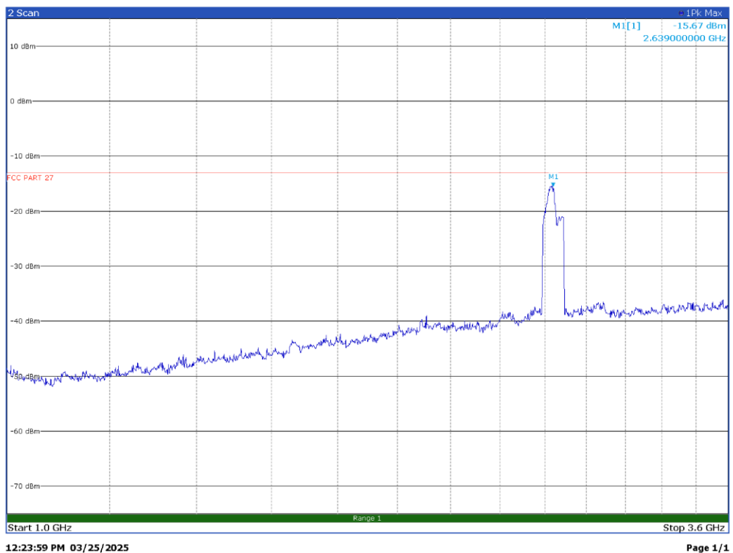
100 MHz signal, top channel, 1GHz – 3.6GHz – V Pol
