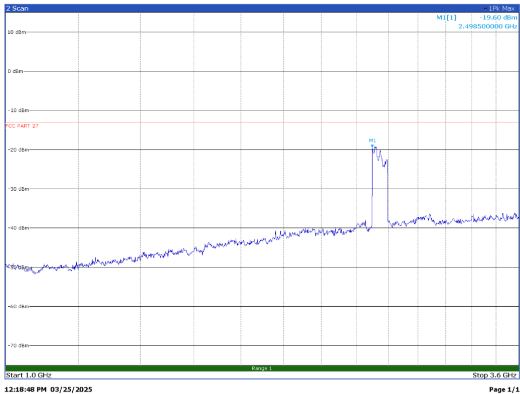
100 MHz signal, bottom channel, 1GHz – 3.6GHz – V Pol
