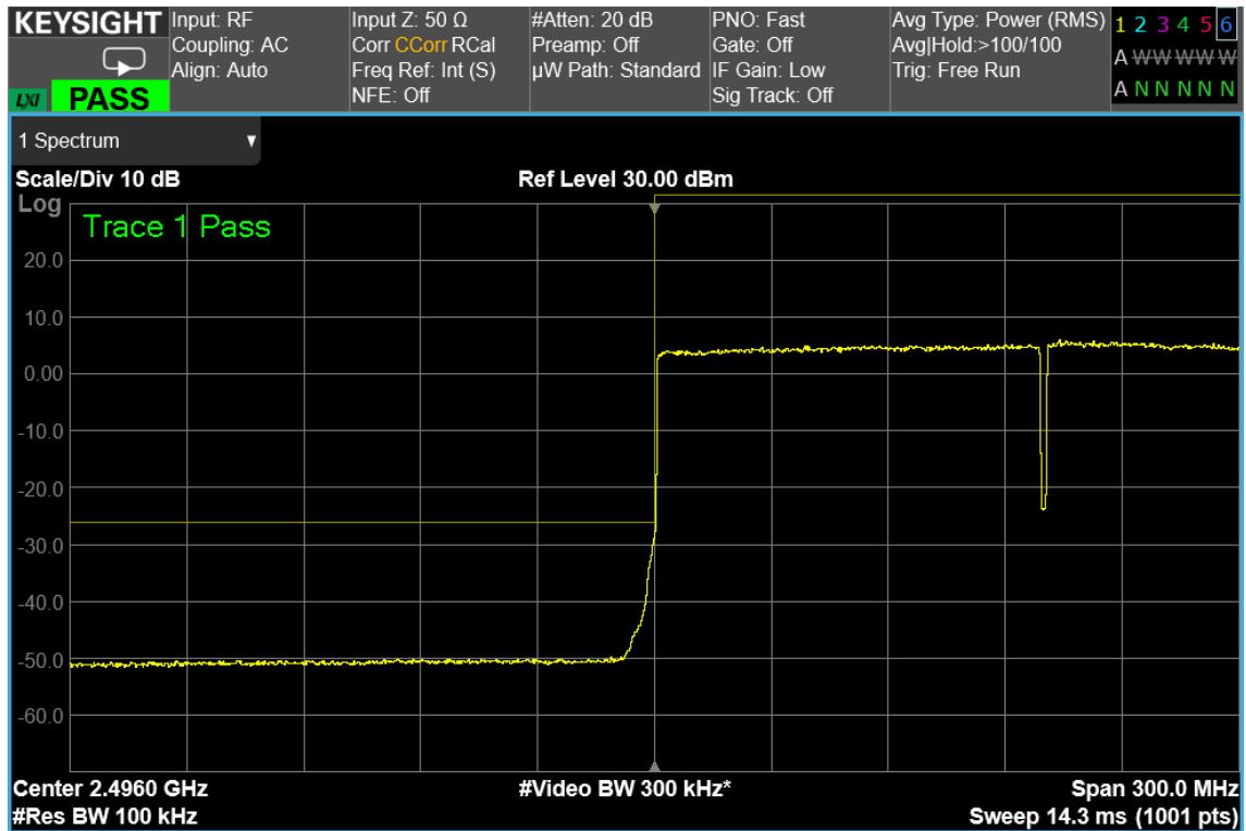
100+90 MHz signal, Low Band Edge, 2 carriers, nominal input signal
