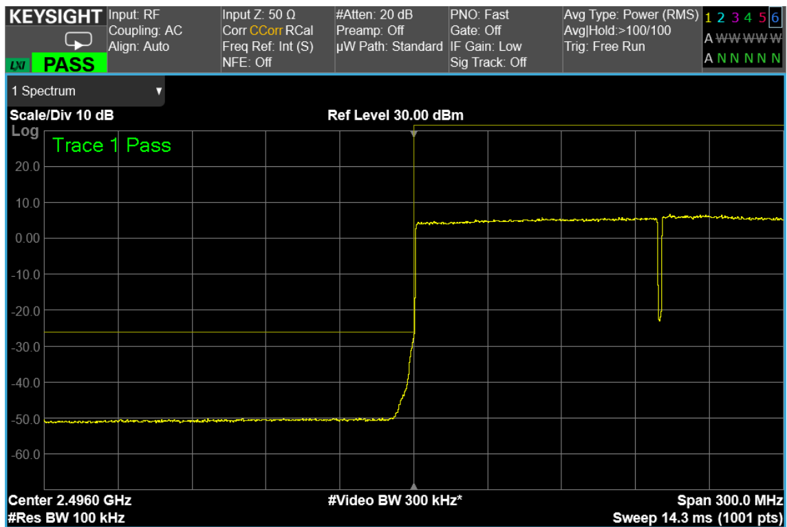
100+90 MHz signal, High Band Edge, 2 carrier, nominal input signal + 3dB
