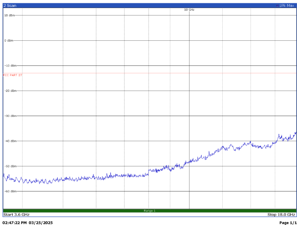
100 MHz signal, bottom channel, 3.6GHz – 18GHz – V Pol
