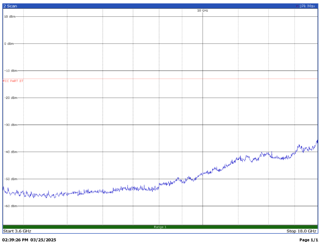
100 MHz signal, top channel, 3.6GHz – 18GHz – V Pol
