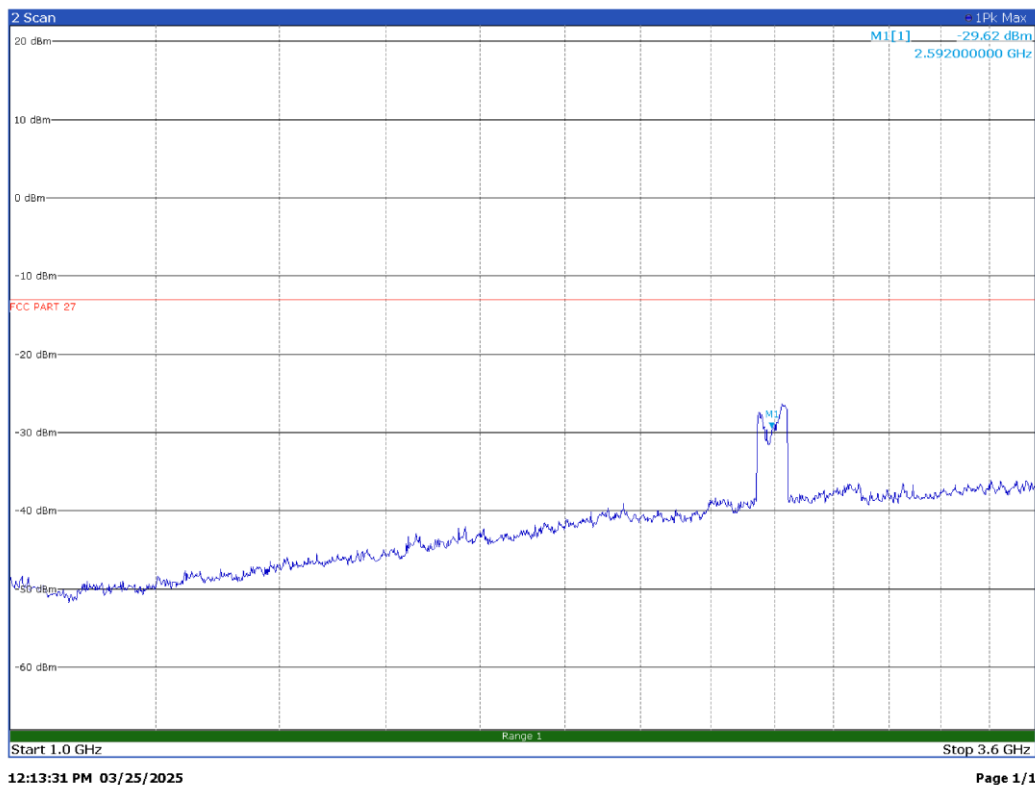
100 MHz signal, middle channel, 1GHz – 3.6GHz – H Pol
