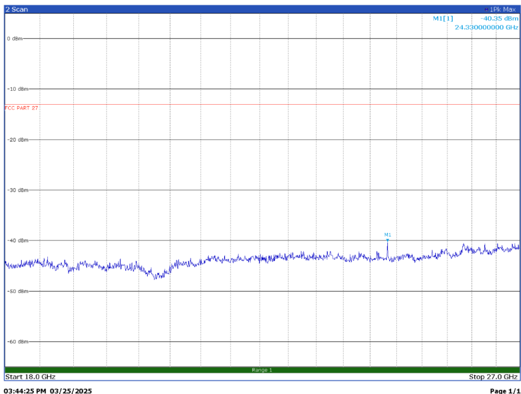
100 MHz signal, bottom channel, 18GHz – 27GHz – V Pol
