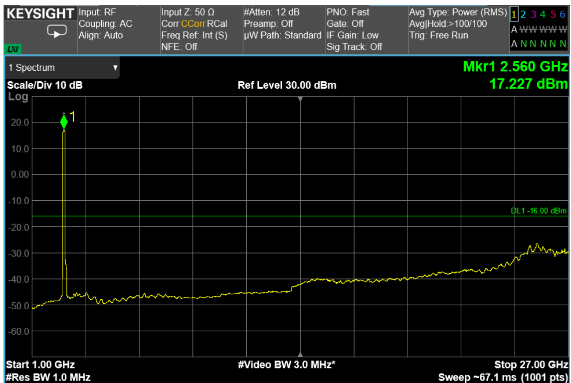
100 MHz signal, bottom channel, 1GHz – 27GHz
