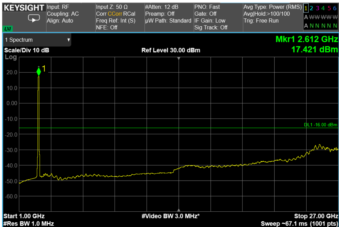
100 MHz signal, middle channel, 1GHz – 27GHz
