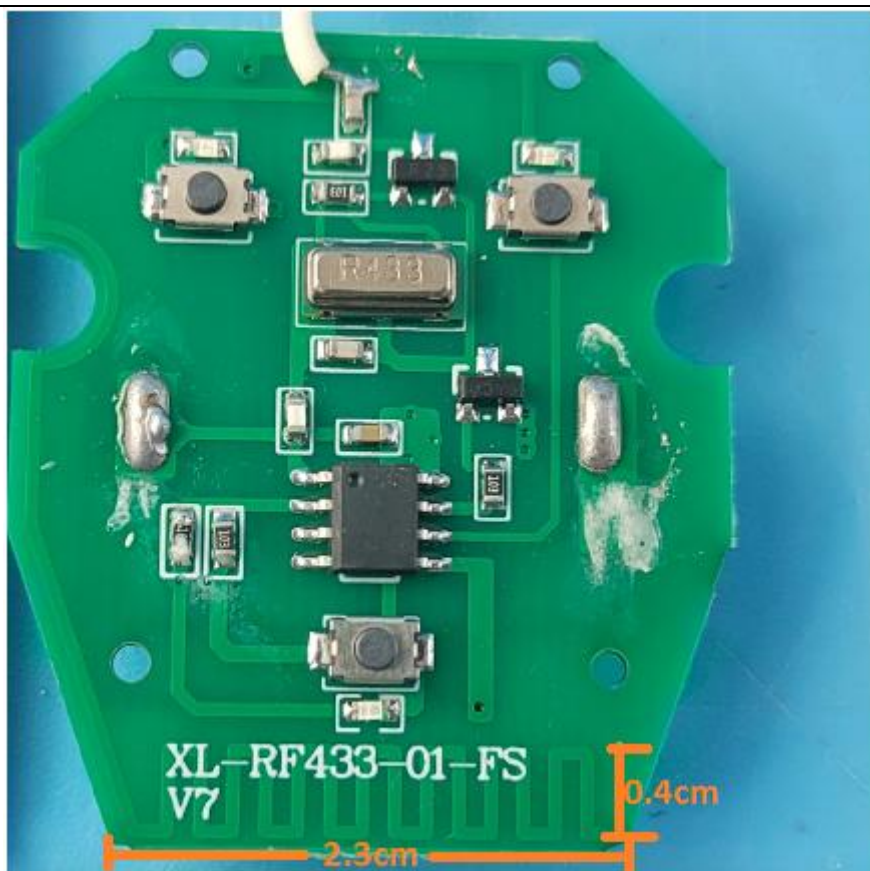
Antenna diagram
