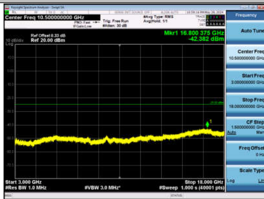
7-7-20MHz-20MHz-QPSK-QPSK-20850-21048-1RB#0-0R B#0-3000~18000MHz-PASS
