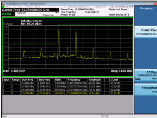
15MHz-10MHz_QPSK@QPSK-QPSK@QPSK_40315-40435_435_1RB#0@75RB#0-1RB#49@50RB#0
