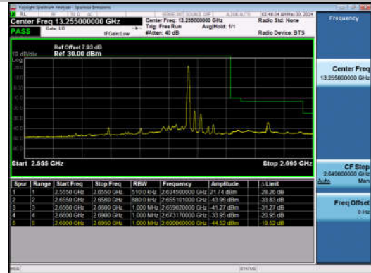
15MHz-20MHz_QPSK@QPSK-QPSK@QPSK_40969-41140_1RB#74@75RB#0-0RB#0@100RB#0
