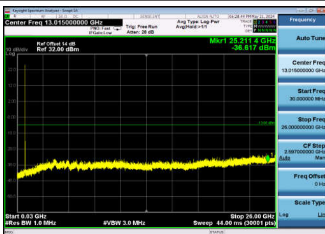
FDD26_Part 22_LowRange_15MHz_30MHz~26GHz
