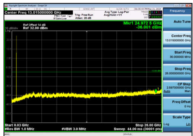
FDD26_Part 22_MidRange_15MHz_30MHz~26GHz
