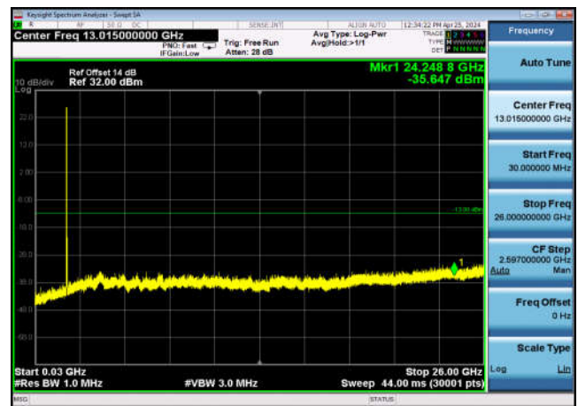
FDD26_Part 22_HighRange_15MHz_30MHz~26GHz
