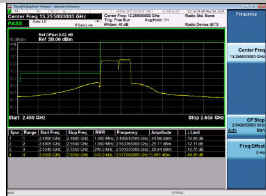
15MHz-10MHz_QPSK@QPSK-QPSK@QPSK_40315-40435_75RB#0@75RB#0-50RB#0@50RB#0
