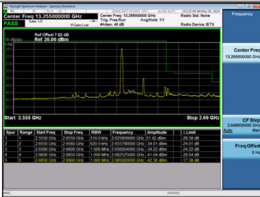
15MHz-15MHz_QPSK@QPSK-QPSK@QPSK_41015-41165_1RB#0@75RB#0-0RB#0@75RB#0
