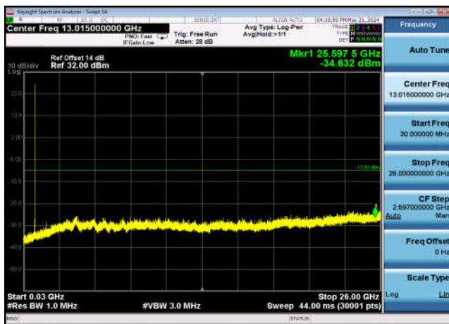
FDD05_MidRange_10MHz_30MHz~26GHz
