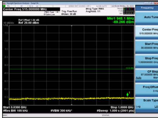
7-7-20MHz-20MHz-QPSK-QPSK-20850-21048-1RB#0-0R B#0-30~1000MHz-PASS
