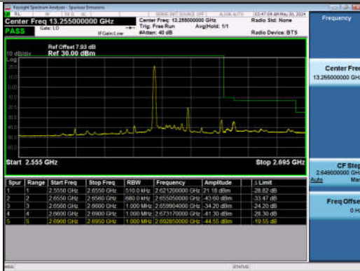
15MHz-20MHz_QPSK@QPSK-QPSK@QPSK_40969-41140_140_1RB#0@75RB#0-0RB#0@100RB#0
