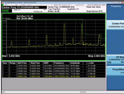
15MHz-10MHz_QPSK@QPSK-QPSK@QPSK_41067-41187_1RB#0@75RB#0-1RB#49@50RB#0
