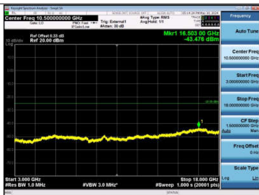
41-41-20MHz-20MHz-QPSK-QPSK-40641-40839-1RB#0-0 RB#0-3000~18000MHz-PASS
