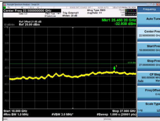
41-41-20MHz-20MHz-QPSK-QPSK-40942-41140-1RB#0-0 RB#0-18000~27000MHz-PASS
