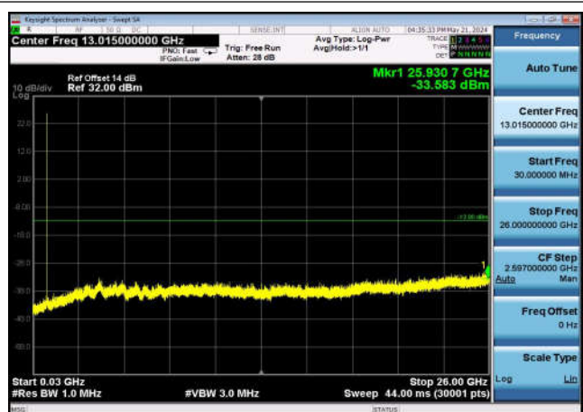
FDD26_Part 90_LowRange_10MHz_30MHz~26GHz
