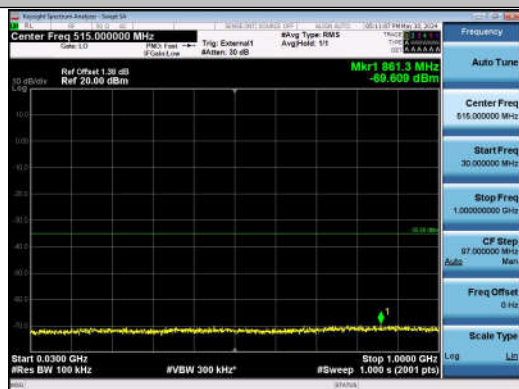
41-41-20MHz-20MHz-QPSK-QPSK-40340-40538-1RB#0-0 RB#0-30~1000MHz-PASS
