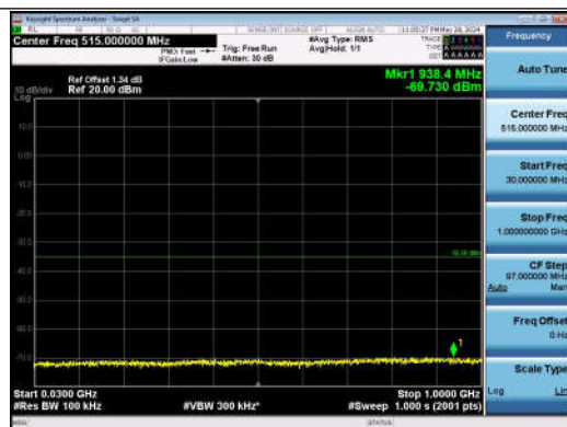
7-7-20MHz-20MHz-QPSK-QPSK-21152-21350-1RB#0-0R B#0-30~1000MHz-PASS
