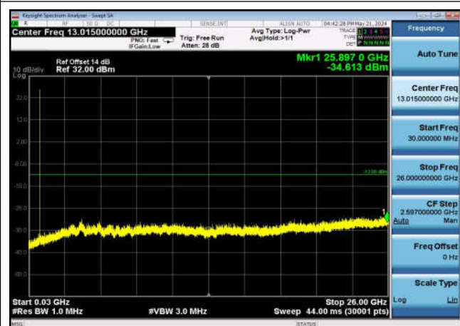
FDD26_Part 90_MidRange_10MHz_30MHz~26GHz
