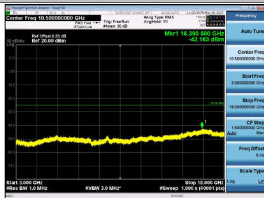
7-7-20MHz-20MHz-QPSK-QPSK-21152-21350-1RB#0-0R B#0-3000~18000MHz-PASS
