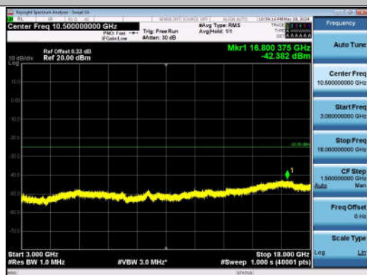
7-7-20MHz-20MHz-QPSK-QPSK-20850-21048-1RB#0-0R B#0-3000~18000MHz-PASS
