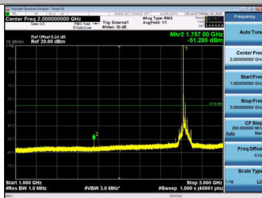
41-41-20MHz-20MHz-QPSK-QPSK-40942-41140-1RB#0-0 RB#0-1000~3000MHz-PASS
