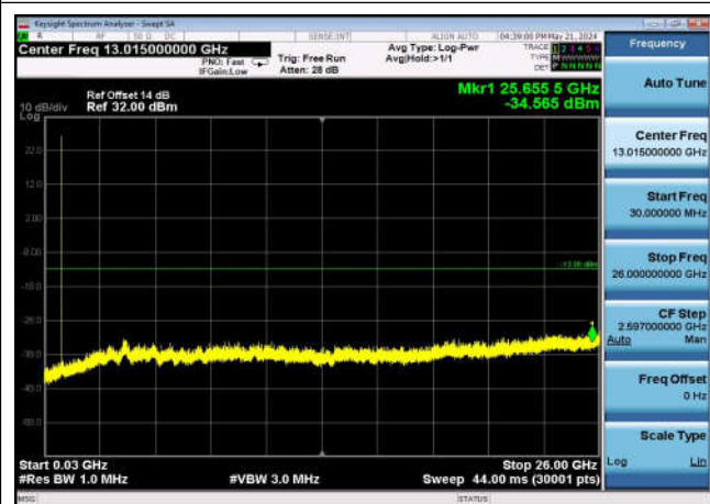
TDD41_LowRange_20MHz_30MHz~26GHz
