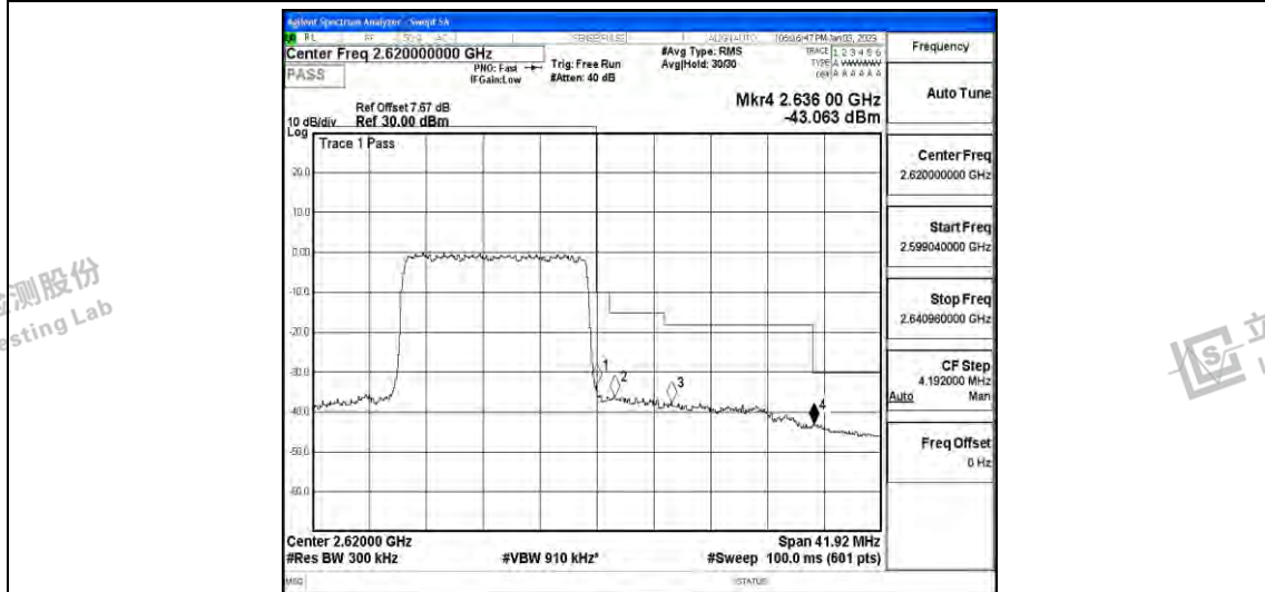
Band38-20MHz-QPSK-37850-100RB#0
