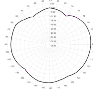
Total(H-XY), Max= -0.45dBi, CirD=8.76
