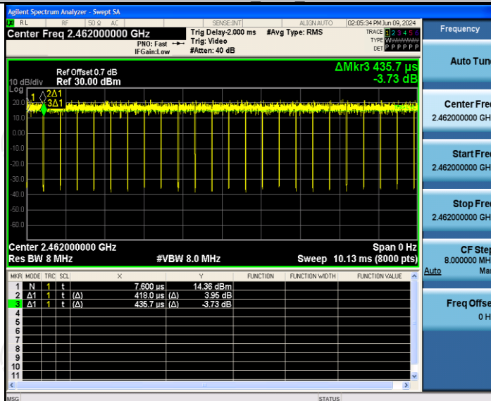
11N20SISO Ant2 2462
