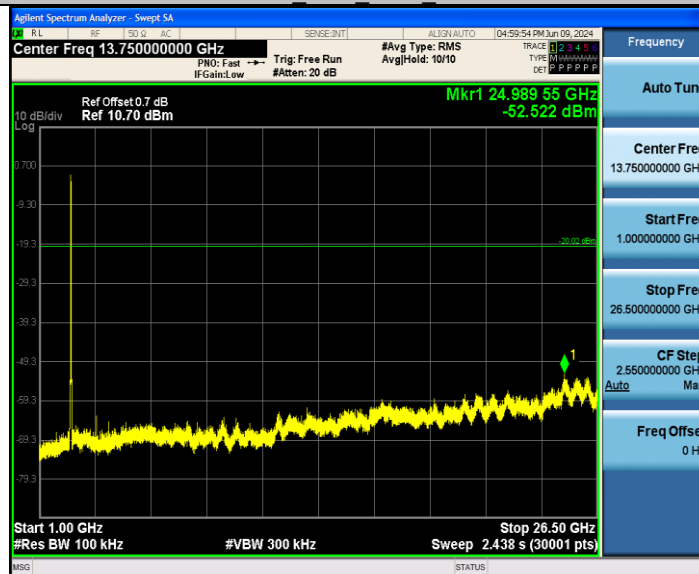
11AX20SISO Ant3 2462 0-Reference
