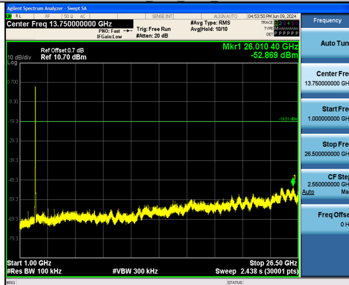
11AX20SISO Ant2 2437 1000~26500
