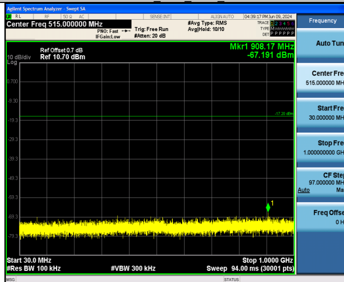
11AX40SISO Ant2 2437 30~1000
