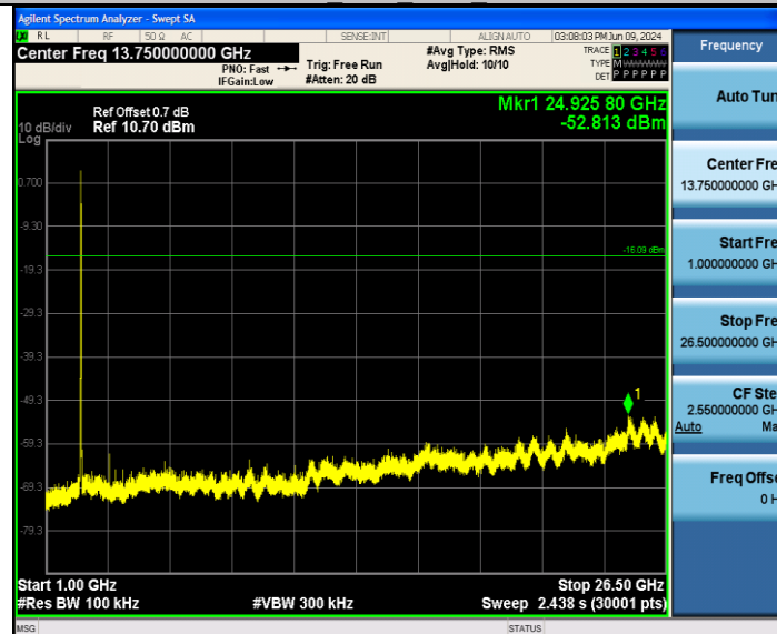
11AX40SISO Ant3 2437 1000~26500
