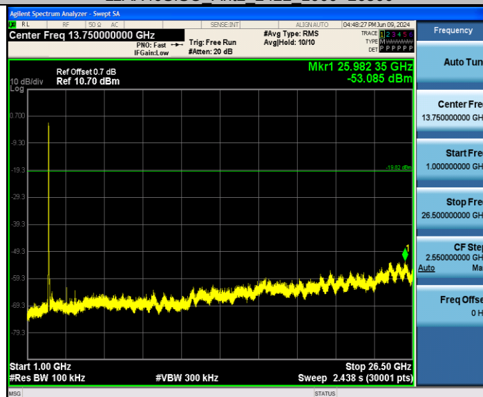
11AX20SISO Ant3 2437 0~Reference
