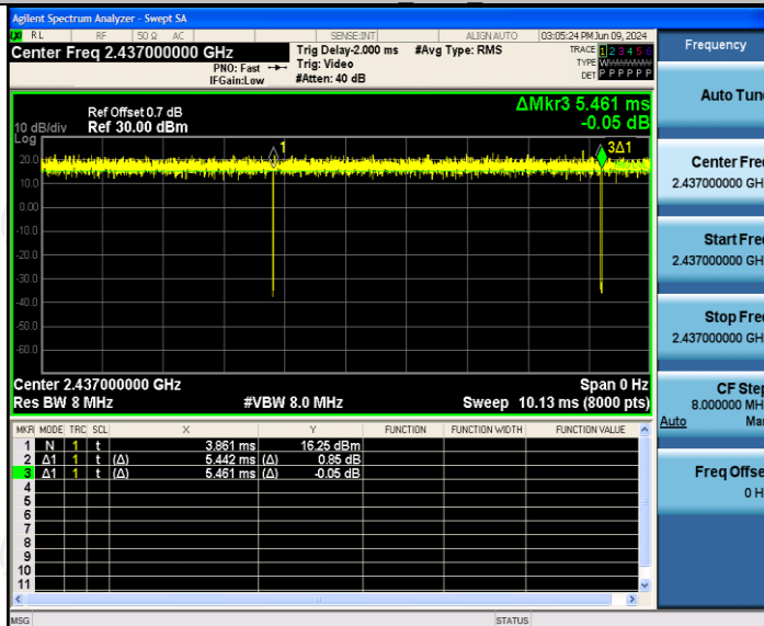
11AX40SISO Ant3 2437
