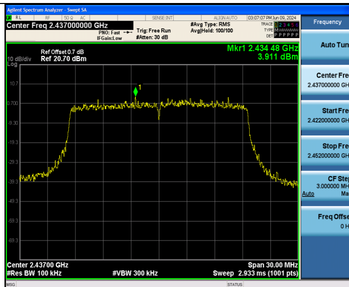
11AX40SISO Ant3 2437 0~Reference
