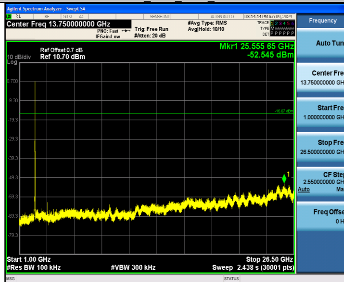
11AX20SISO Ant2 2462 0~Reference
