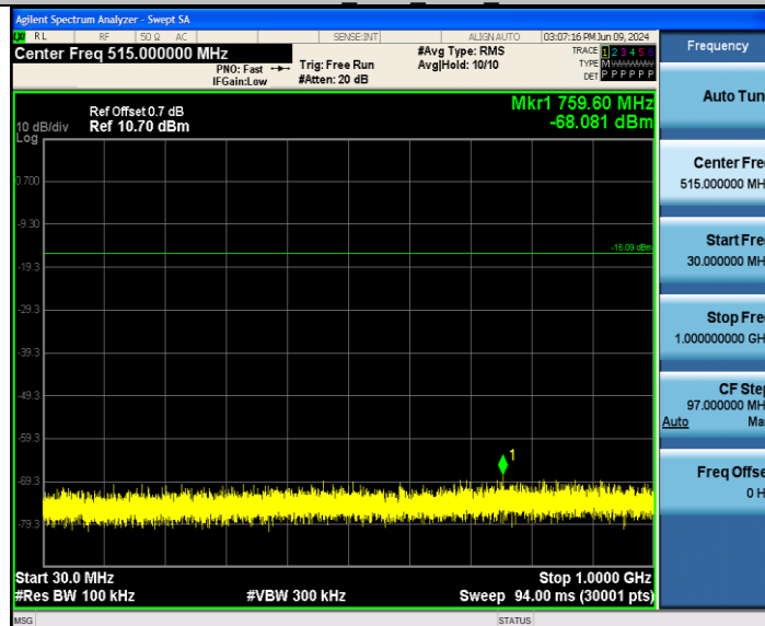
11AX40SISO Ant3 2437 30~1000
